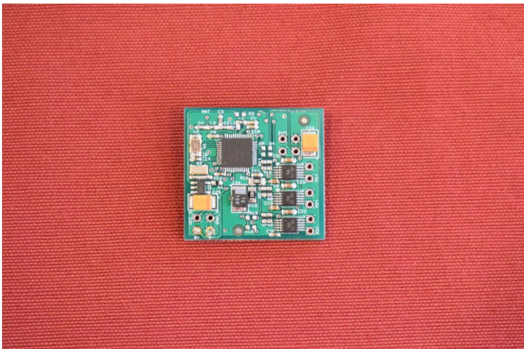
Picture 2: RF module 2.4 GHz – bottom view
