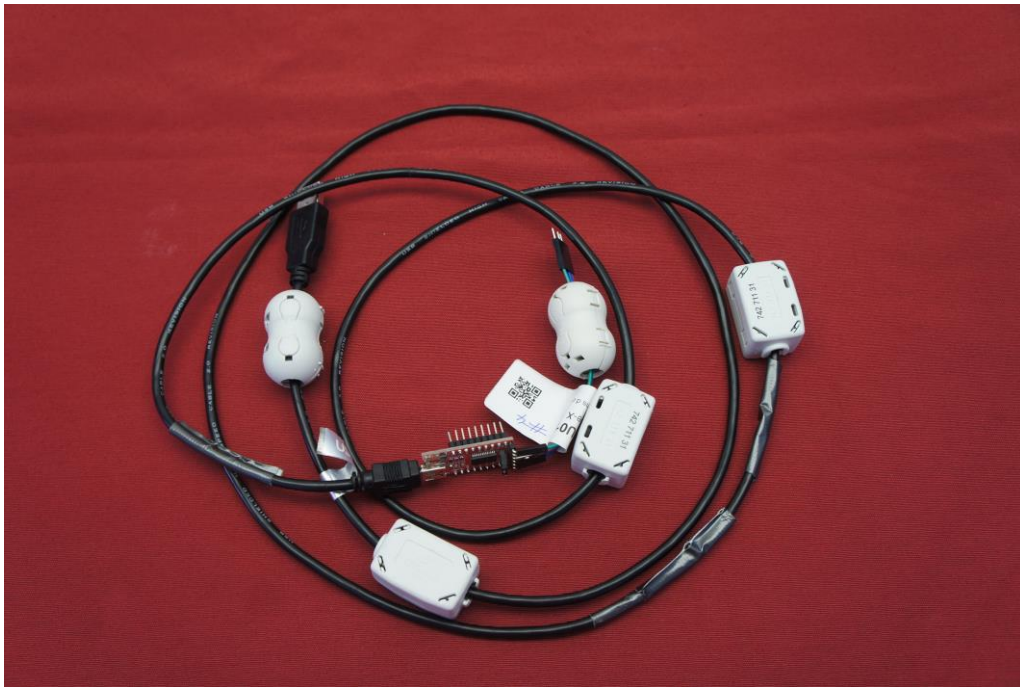
Picture 3: Front view of test cable with UART-USB-adapter
