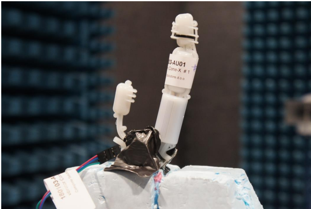
Picture 3: EUT position 3 – front view
