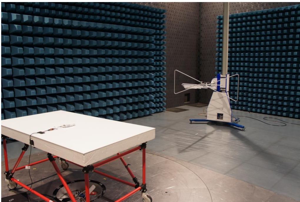
Picture 6: SAC, radiated emission test 30 MHz – 1 GHz – position 1 (front view)
