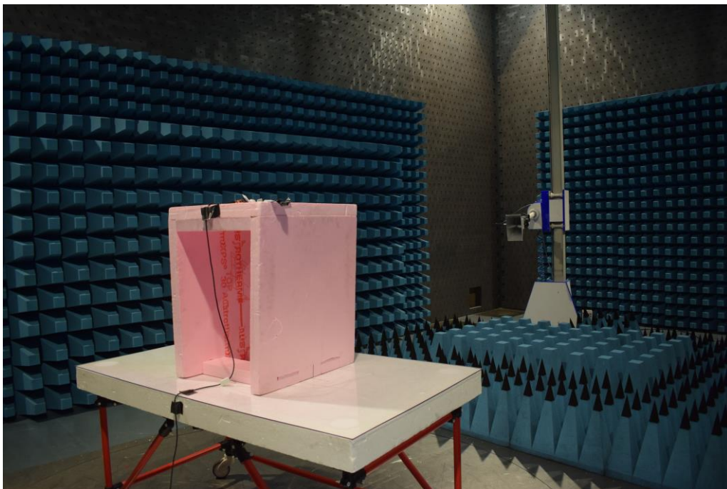
Picture 8: SAC, radiated emission test 1 GHz – 10 GHz – position 1 (front view)
