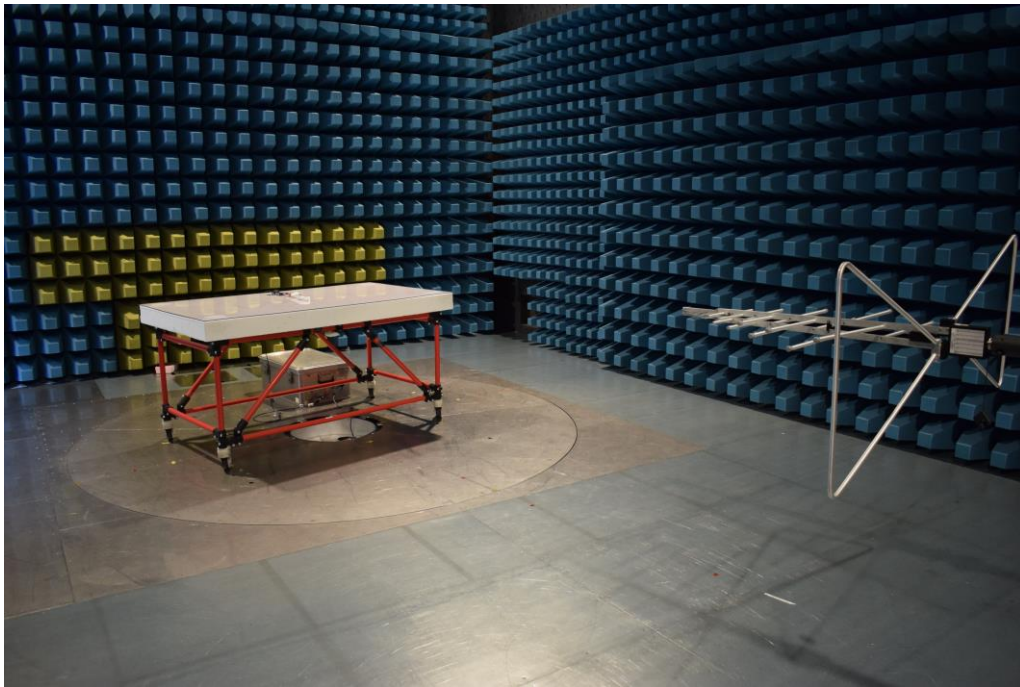
Picture 5: SAC, radiated emission test 30 MHz – 1 GHz – position 1 (rear view)
