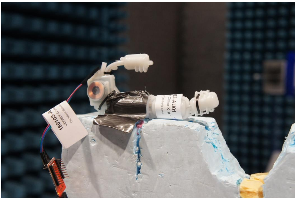
Picture 2: EUT position 2 – front view
