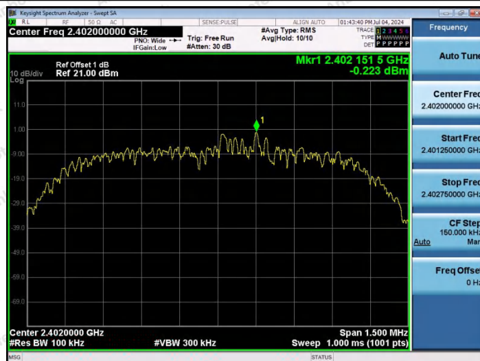
2DH5-Ant1-2402-0~Reference-PASS
