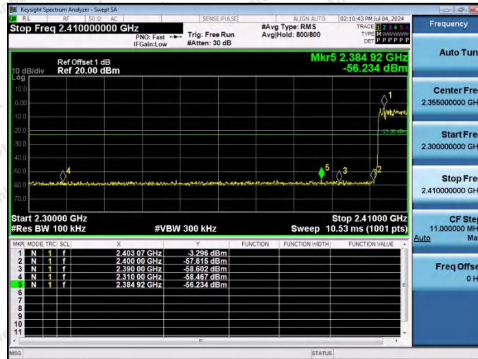
2DH5-Ant1-Hop_2402-PASS
