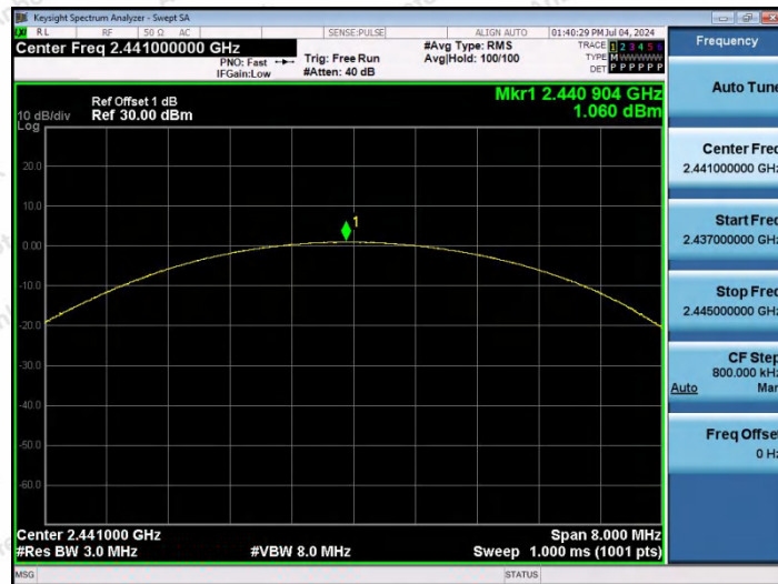
DH5-Ant1-2441-PASS
