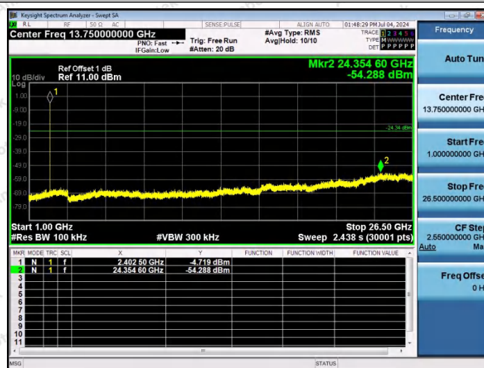
3DH5-Ant1-2402-1000~26500-PASS
