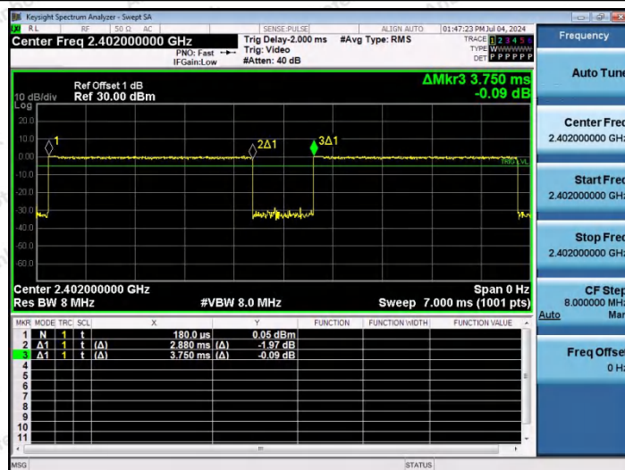
NTVN-3DH5-Ant1-2402
