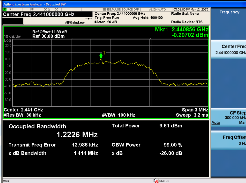
3DH5-Ant1-2441
