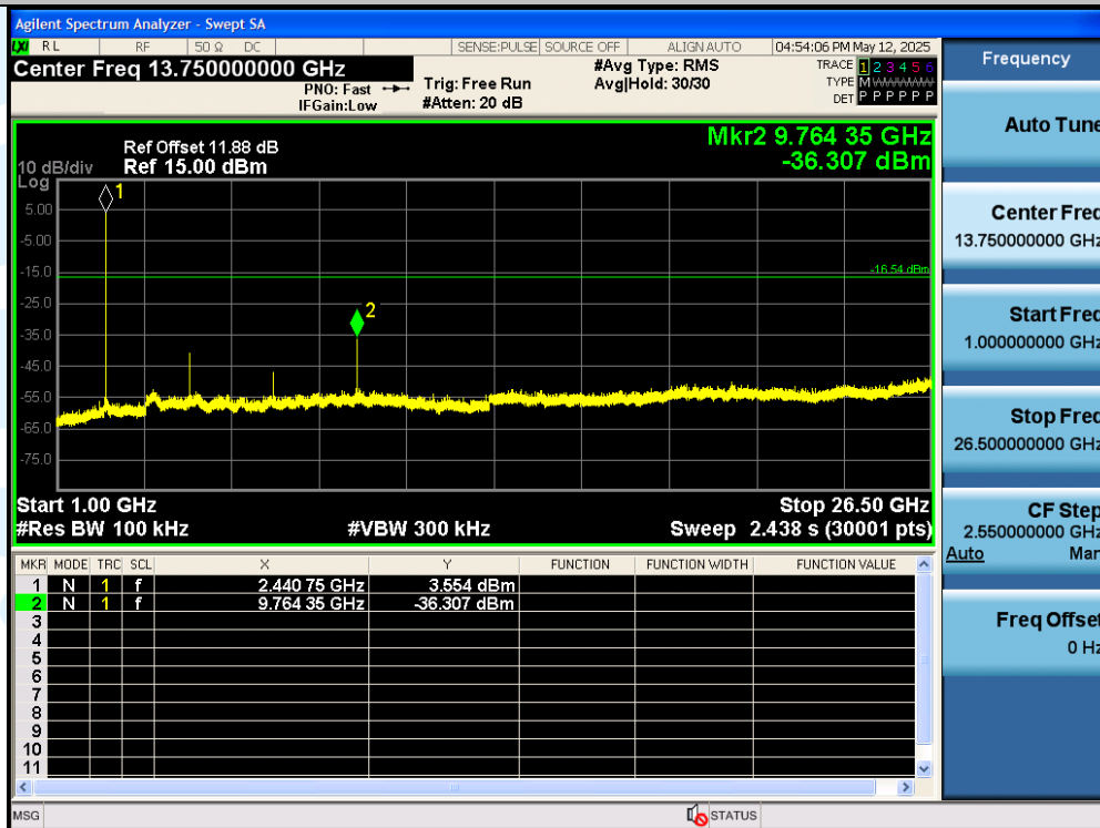
2DH5-Ant1-2441-1000~26500-PASS
