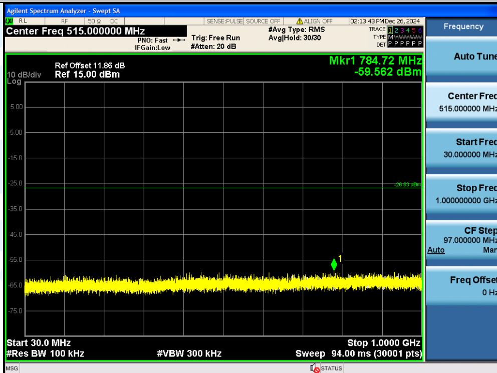
2DH5-Ant1-2402-30~1000-PASS
