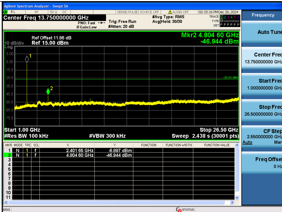
2DH5-Ant1-2402-1000~26500-PASS
