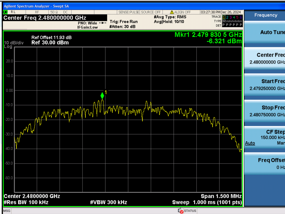
2DH5-Ant1-2480-0~Reference-PASS
