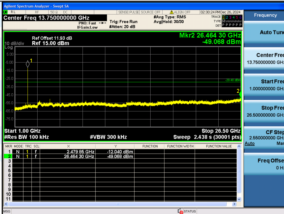
3DH5-Ant1-2480-1000~26500-PASS
