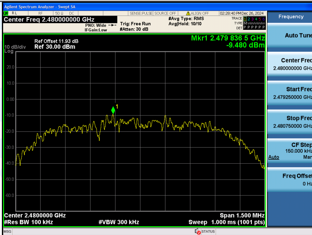
3DH5-Ant1-2480-0~Reference-PASS
