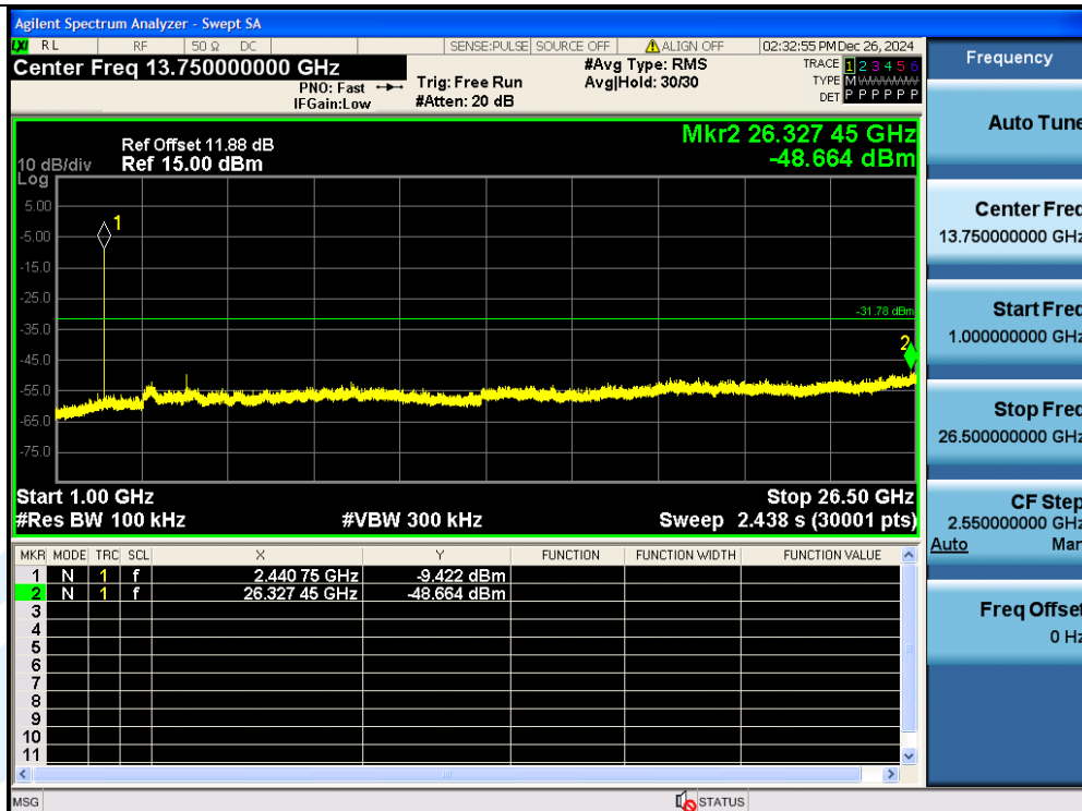
3DH5-Ant1-2441-1000~26500-PASS
