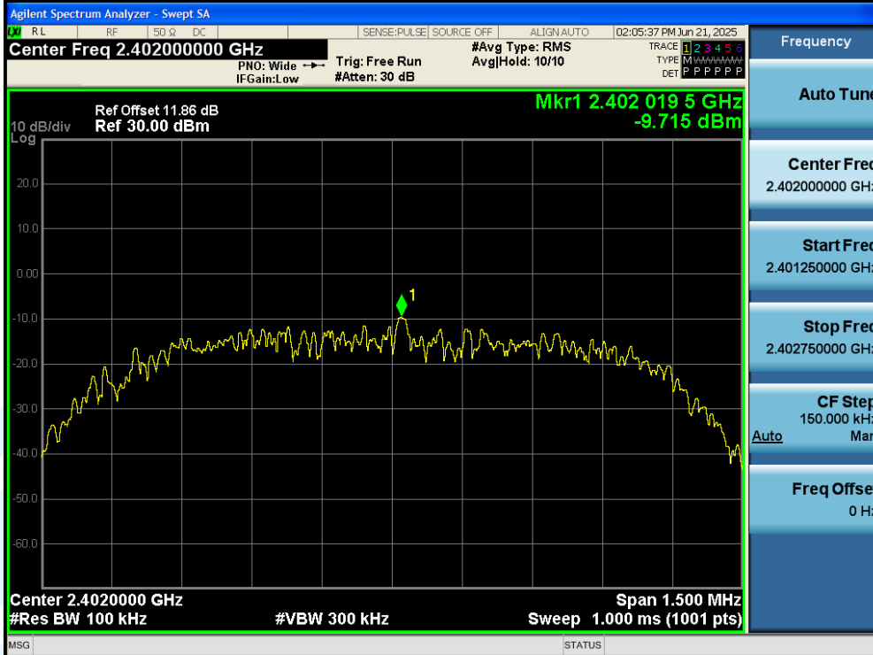
3DH5-Ant1-2402-0~Reference-PASS
