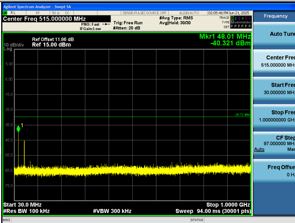
3DH5-Ant1-2402-30~1000-PASS
