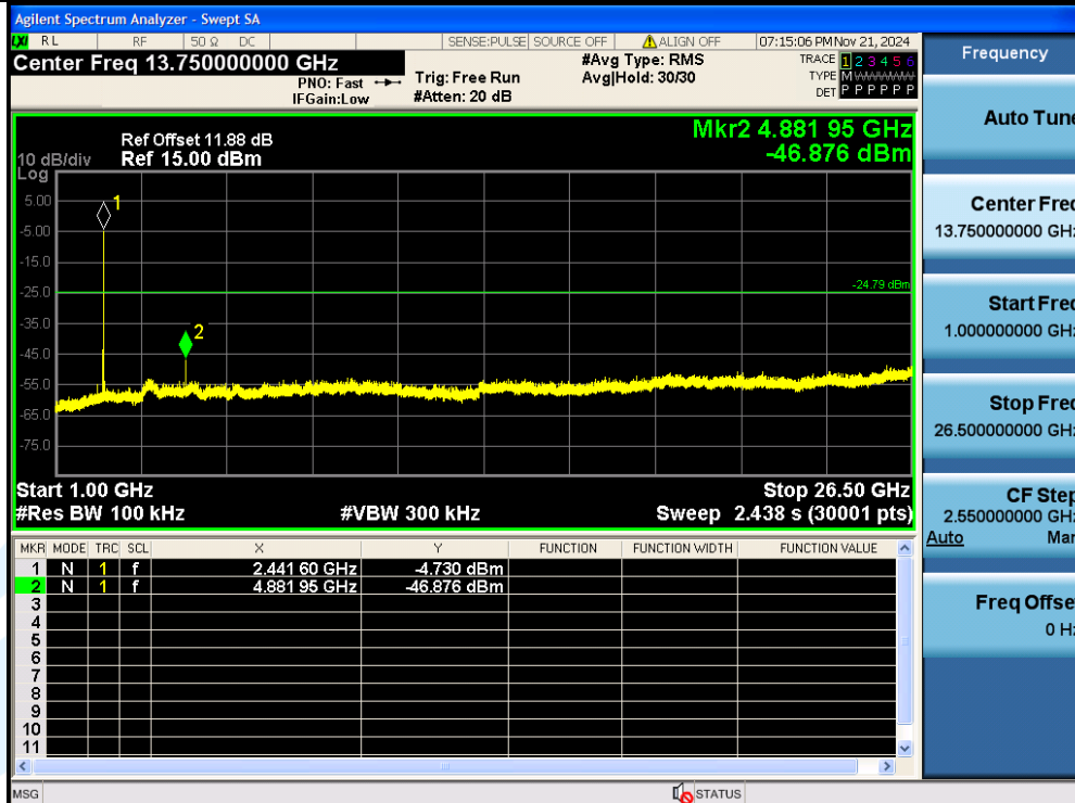
2DH5-Ant1-2441-1000~26500-PASS
