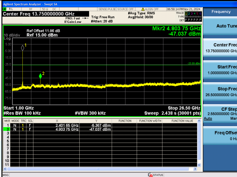
DH5-Ant1-2402-1000~26500-PASS
