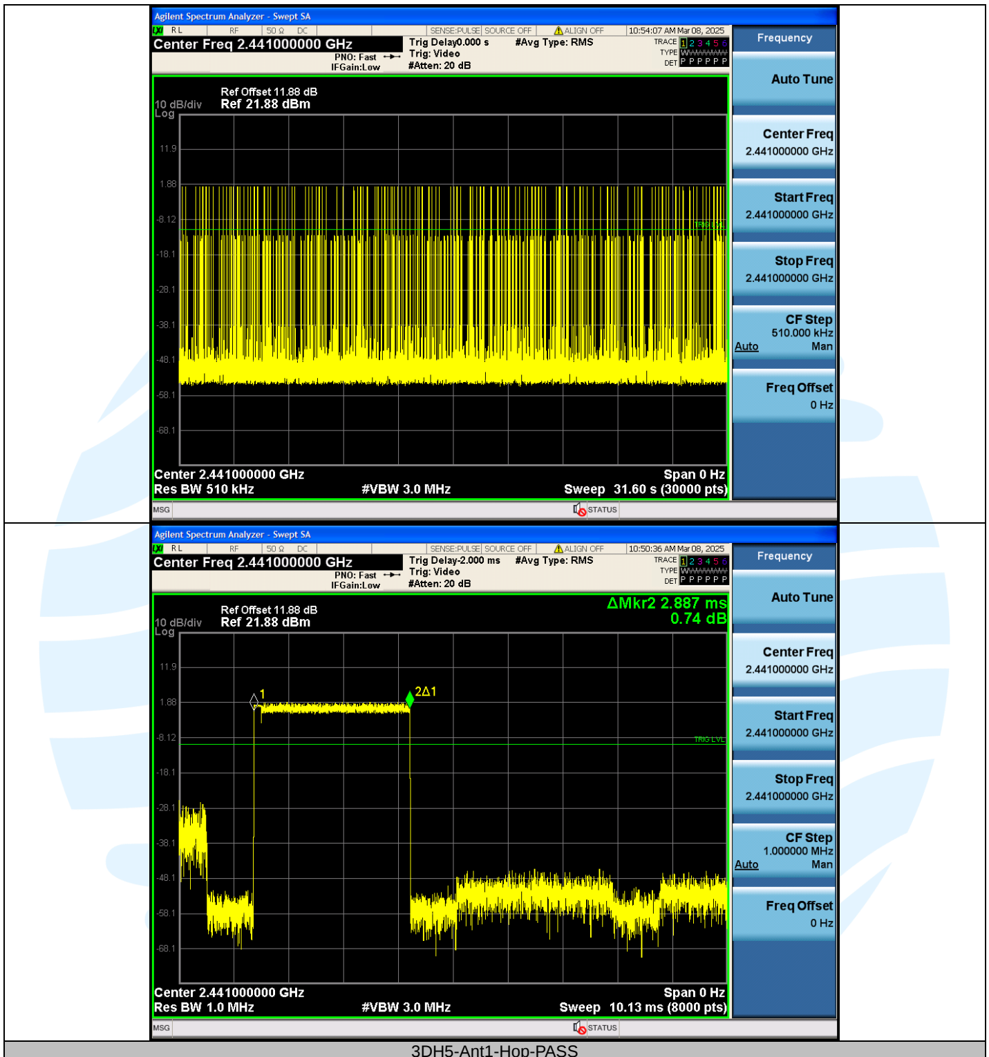
3DH5-Ant1-Hop-PASS
