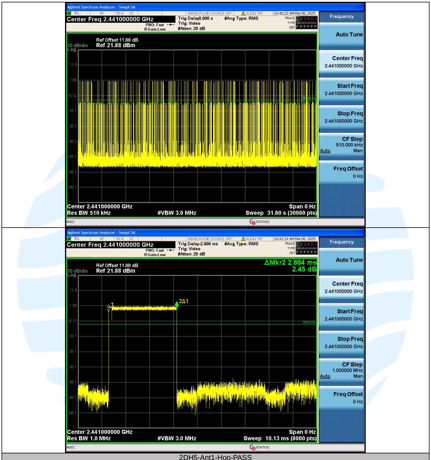
2DH5-Ant1-Hop-PASS
