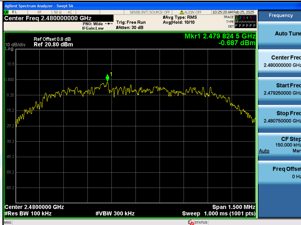
3DH5-Ant1-2480-0-Reference-PASS
