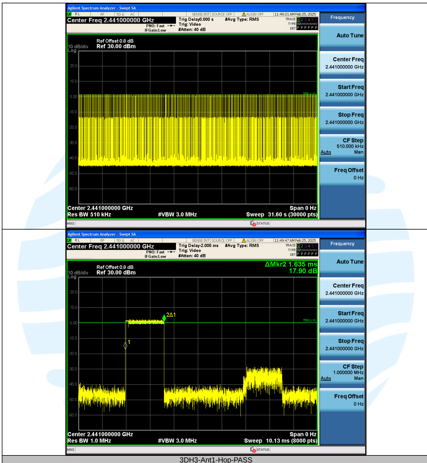
3DH3-Ant1-Hop-PASS
