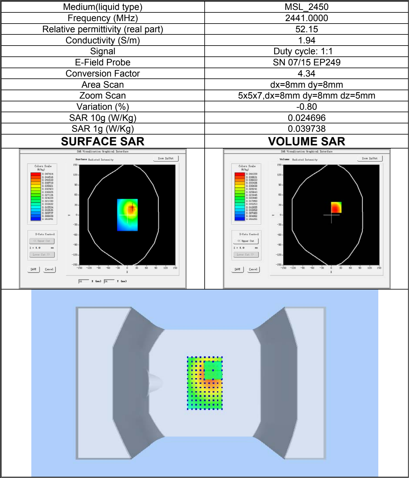
Plot 4:Middle channel (Body, Front Surface) Product Description:Remote Controller Test Date: 2017-10-12
