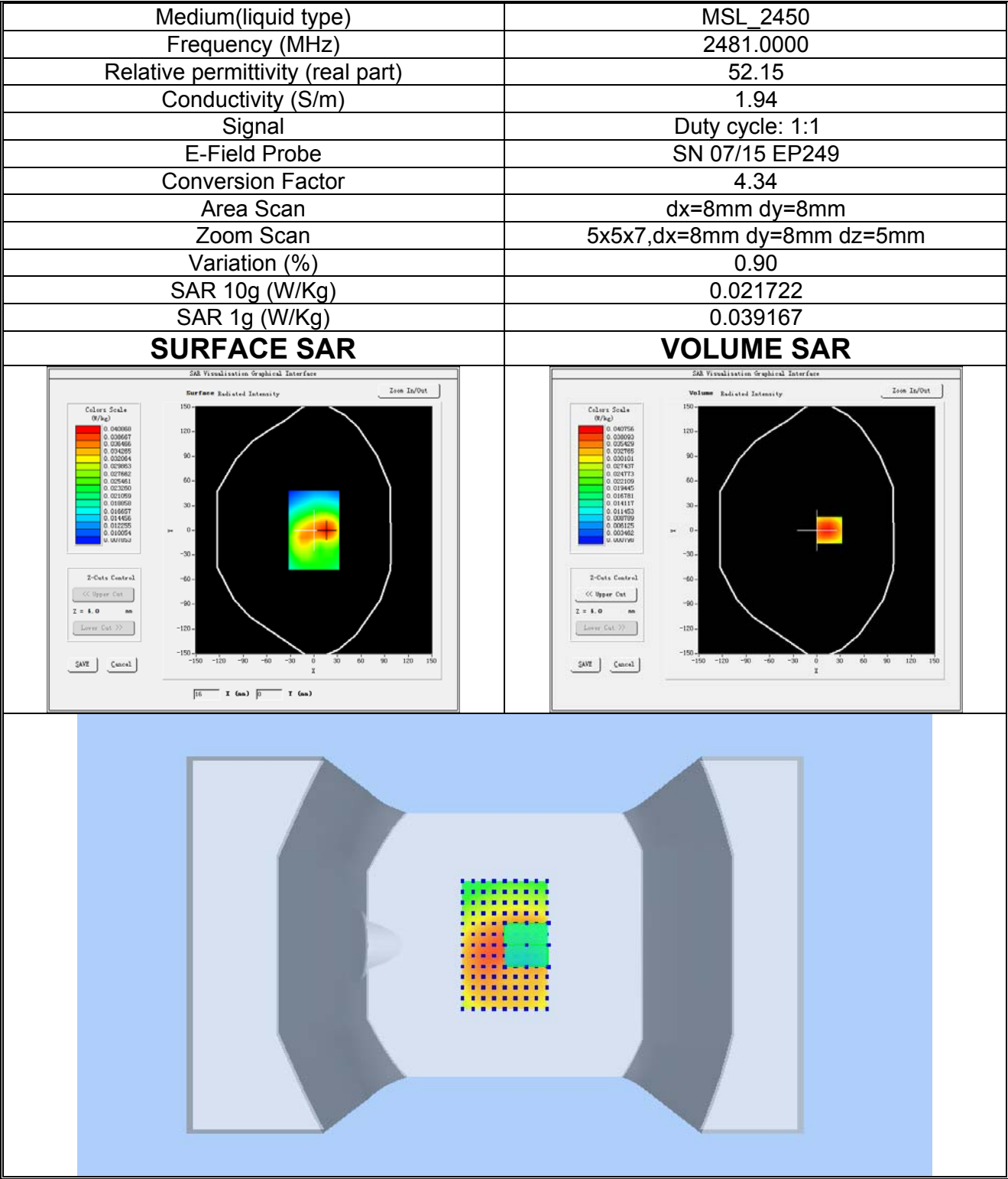
Plot 9:High channel (Body, Top Edge) Product Description:Remote Controller Test Date: 2017-10-12
