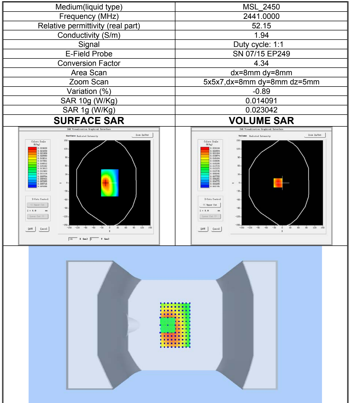
Plot 5: Middle channel (Body, Back Surface) Product Description: Remote Controller Test Date: 2017-10-12
