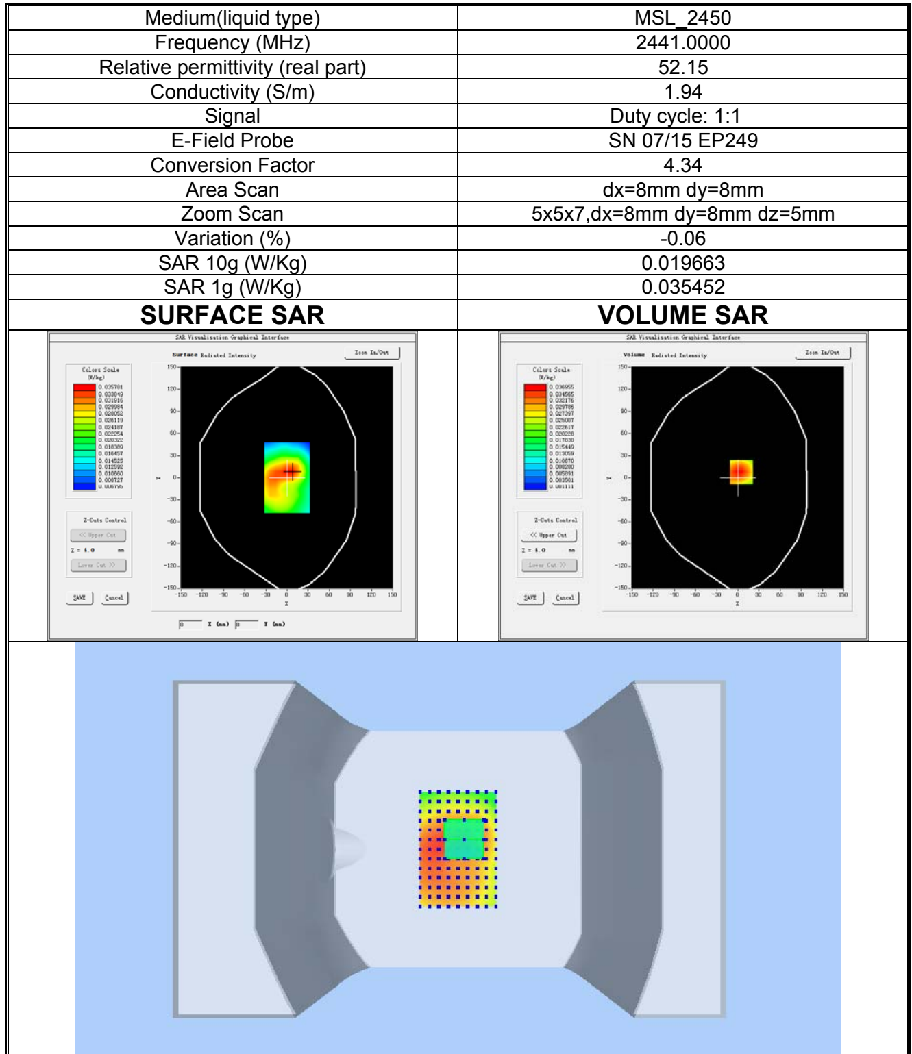
Plot 6: Middle channel (Body, Top Edge) Product Description: Remote Controller Test Date: 2017-10-12
