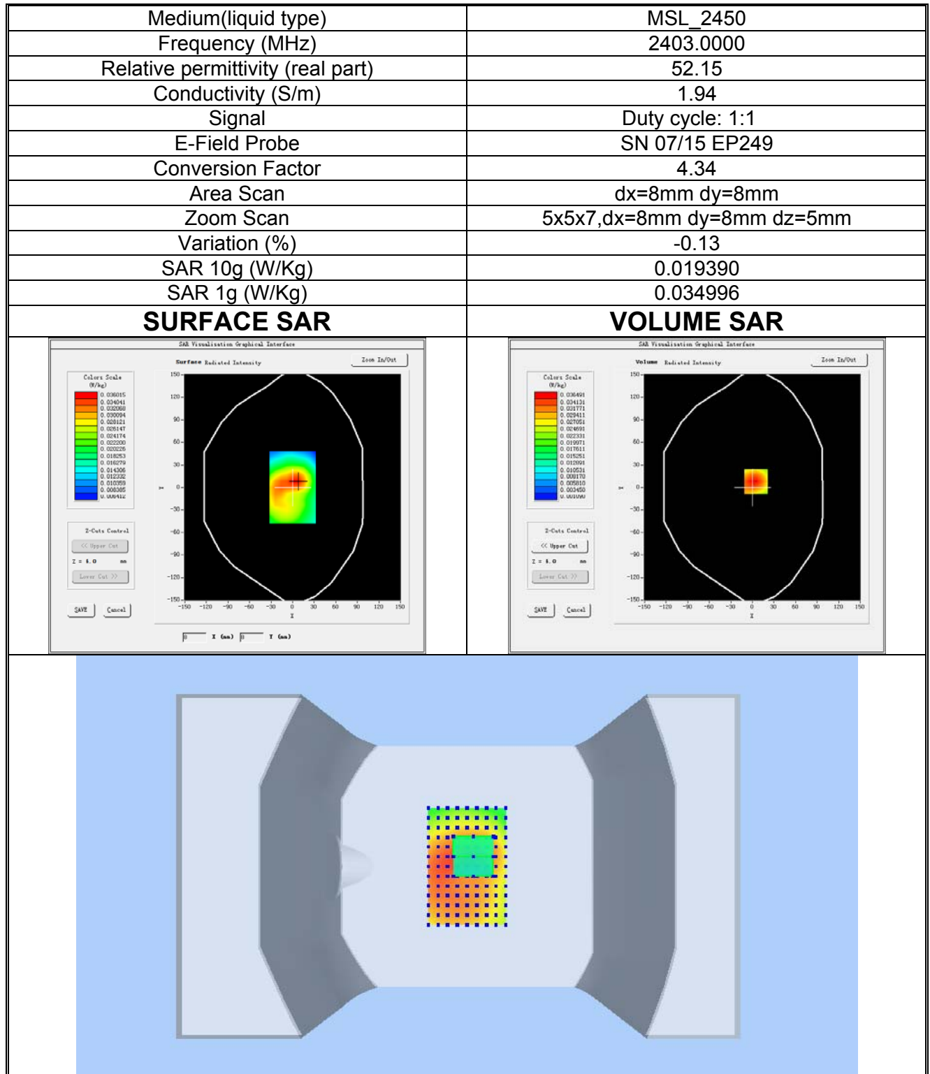
Plot 3:Low channel (Body, Top Edge) Product Description:Remote Controller Test Date: 2017-10-12
