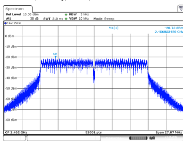
(802.11g) PSD plot on channel 11
