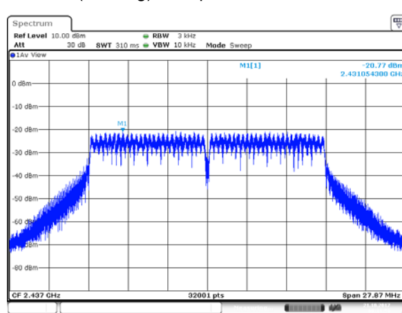
(802.11g) PSD plot on channel 6
