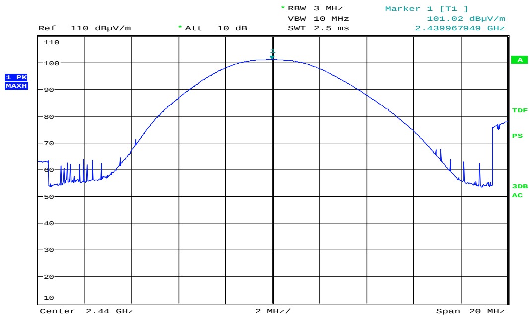
Conducted Power, 2440 MHz, BT LE 2Mb
