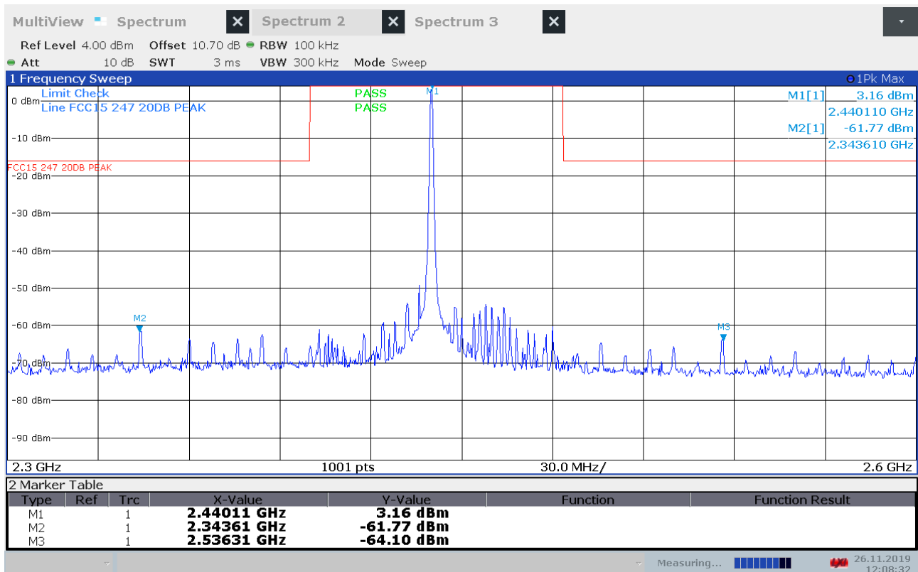
Conducted Emissions, 2300 - 2600 MHz, 2440 MHz, BT LE LR
