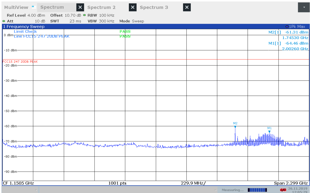
Conducted Emissions, 1 – 2300 MHz, 2402 MHz, BT LE LR
