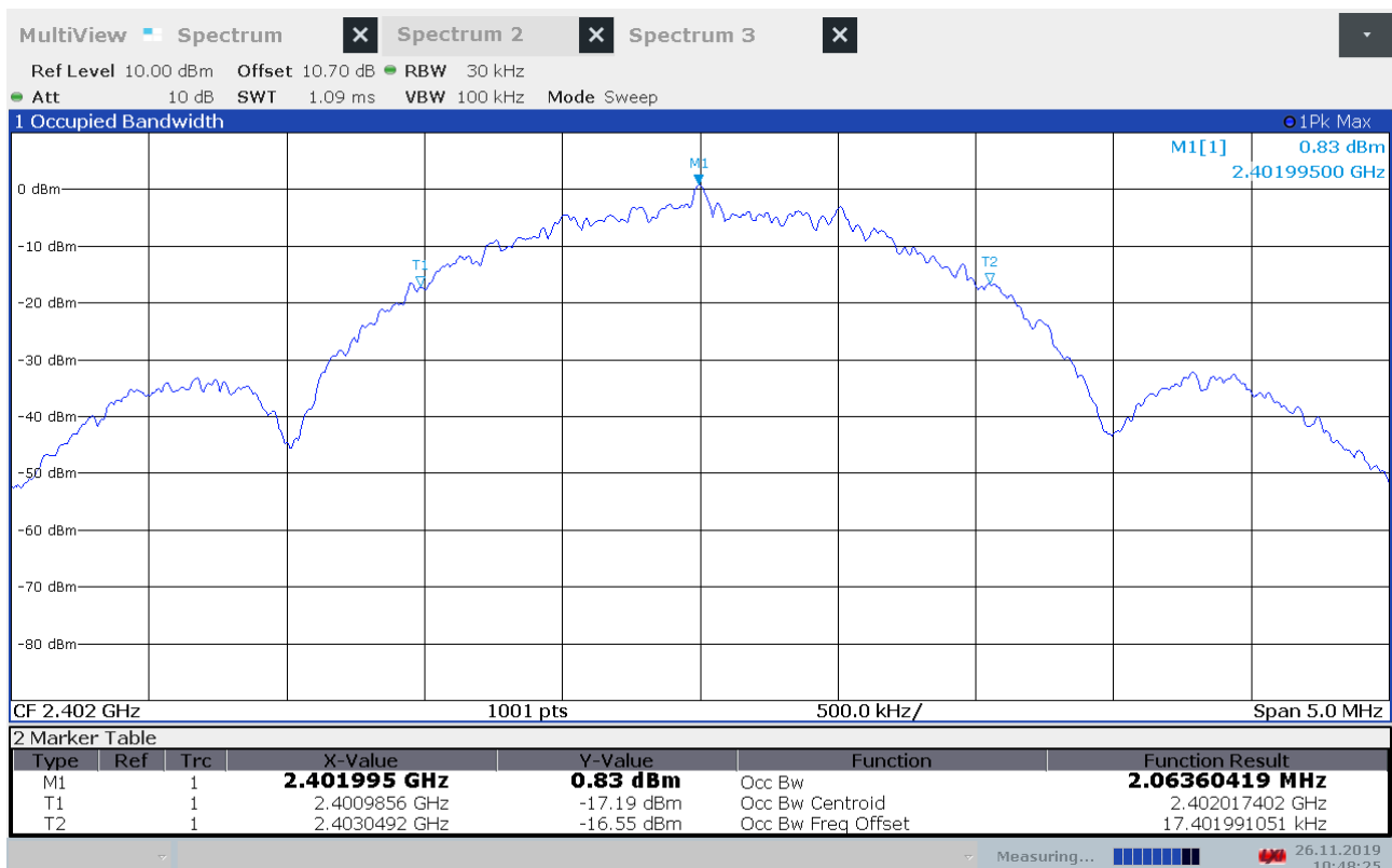
99% Bandwidth, 2402 MHz, BT LE 2Mb
