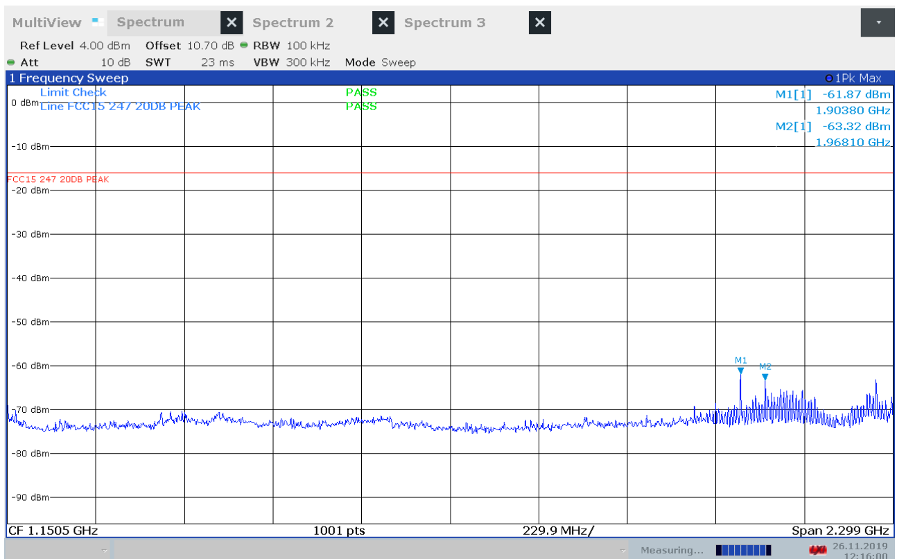
Conducted Emissions, 1 – 2300 MHz, 2480 MHz, BT LE 2Mb
