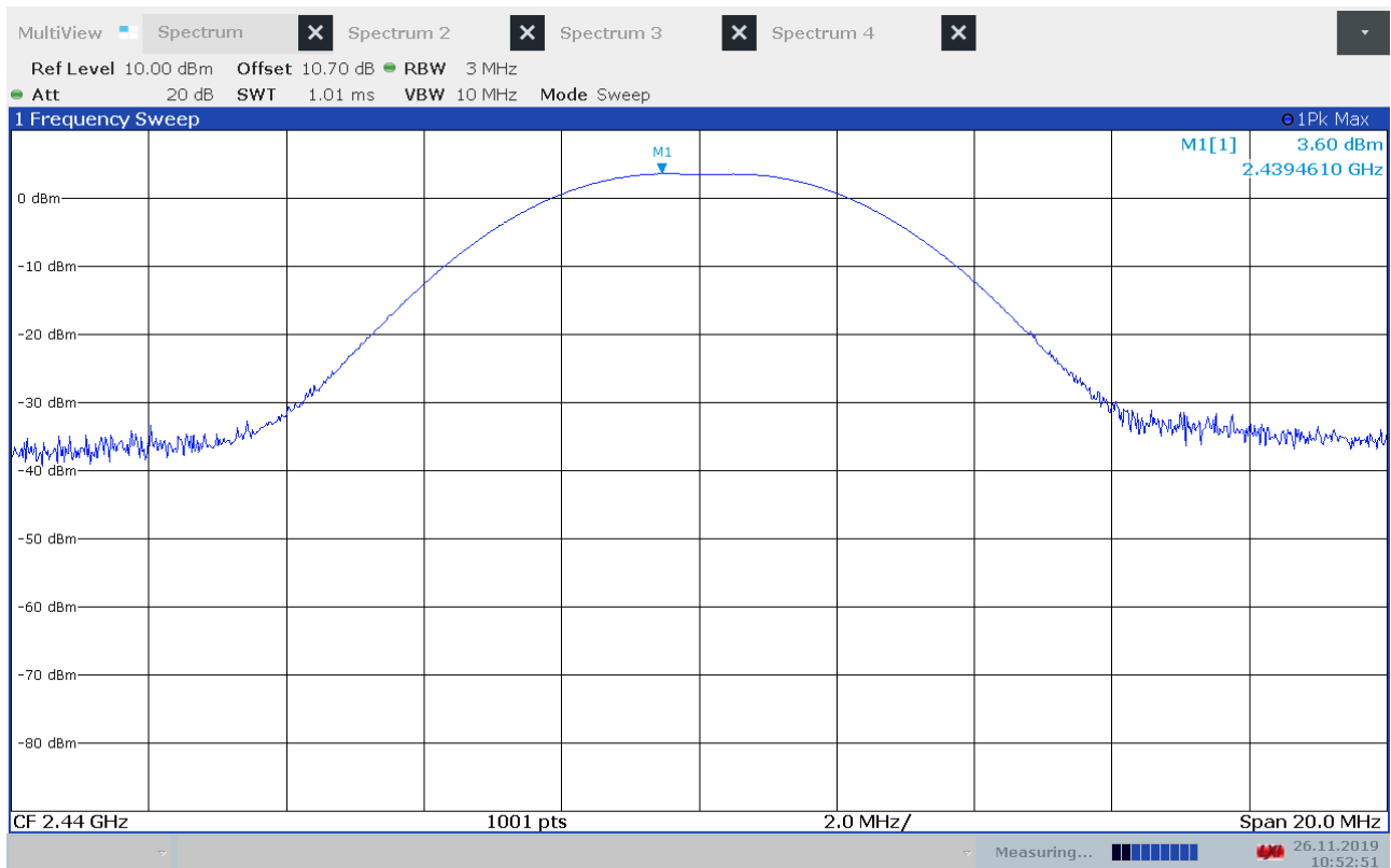
Conducted Power, 2440 MHz, BT LE 2Mb
