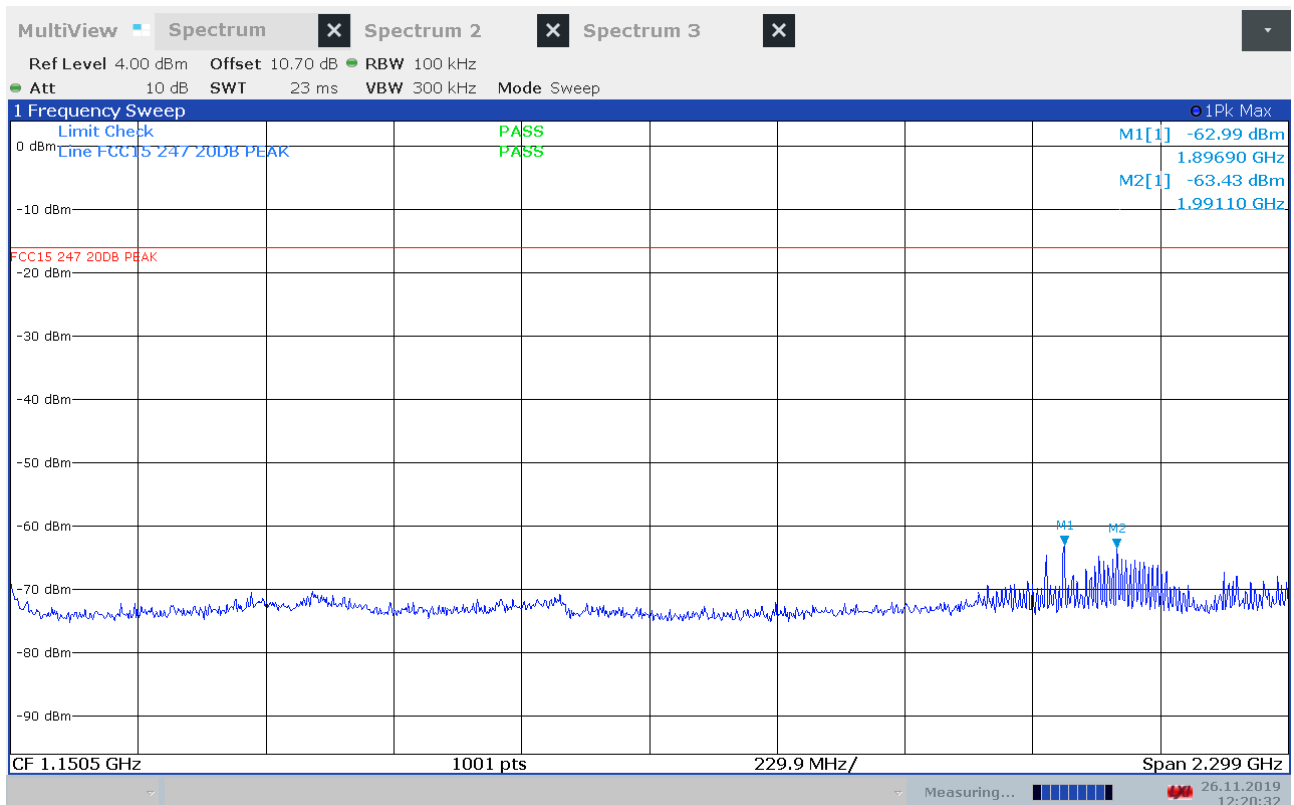
Conducted Emissions, 1 – 2300 MHz, 2440 MHz, BT LE 2Mb
