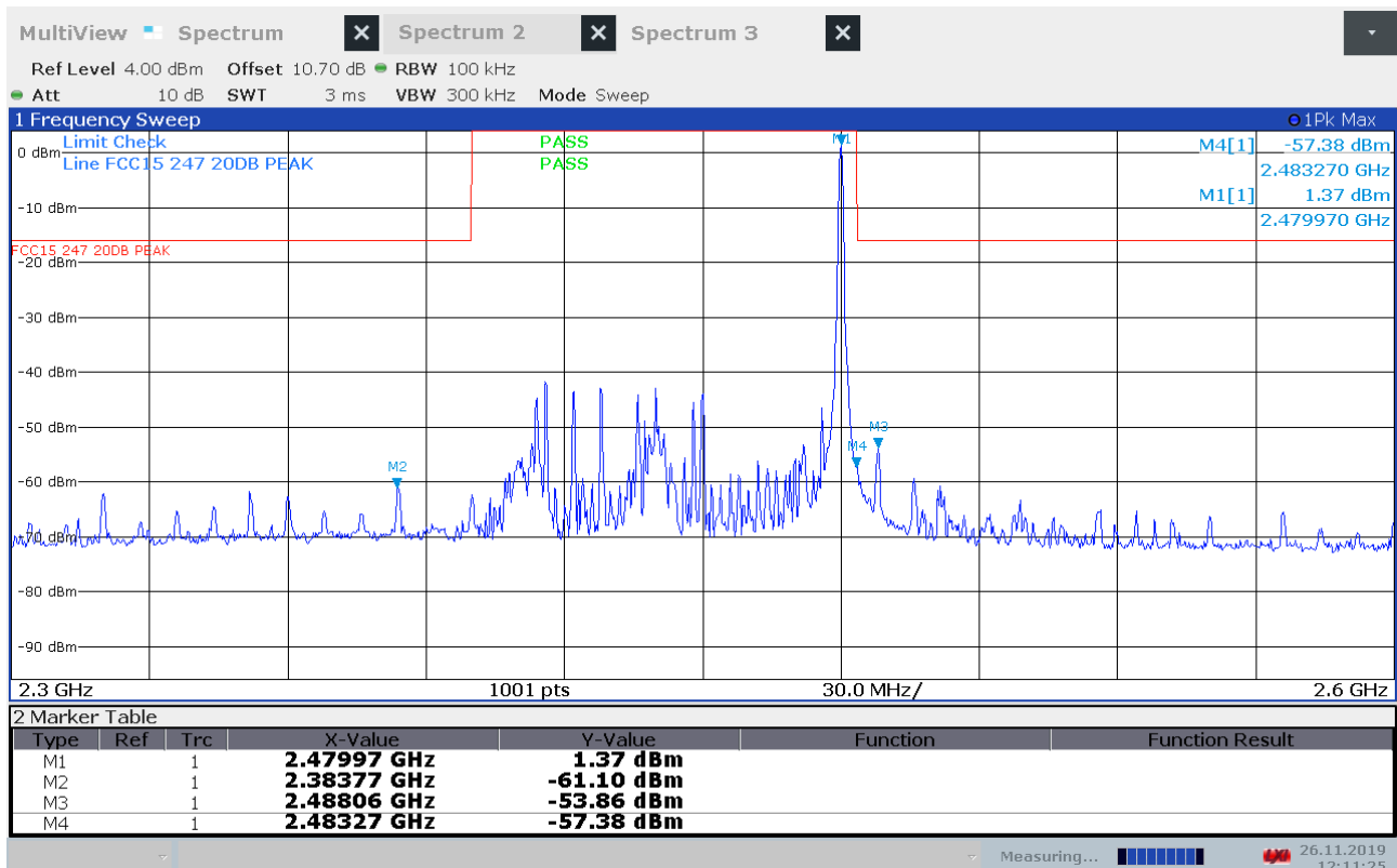
Conducted Emissions, 2300 - 2600 MHz, 2480 MHz, BT LE LR
