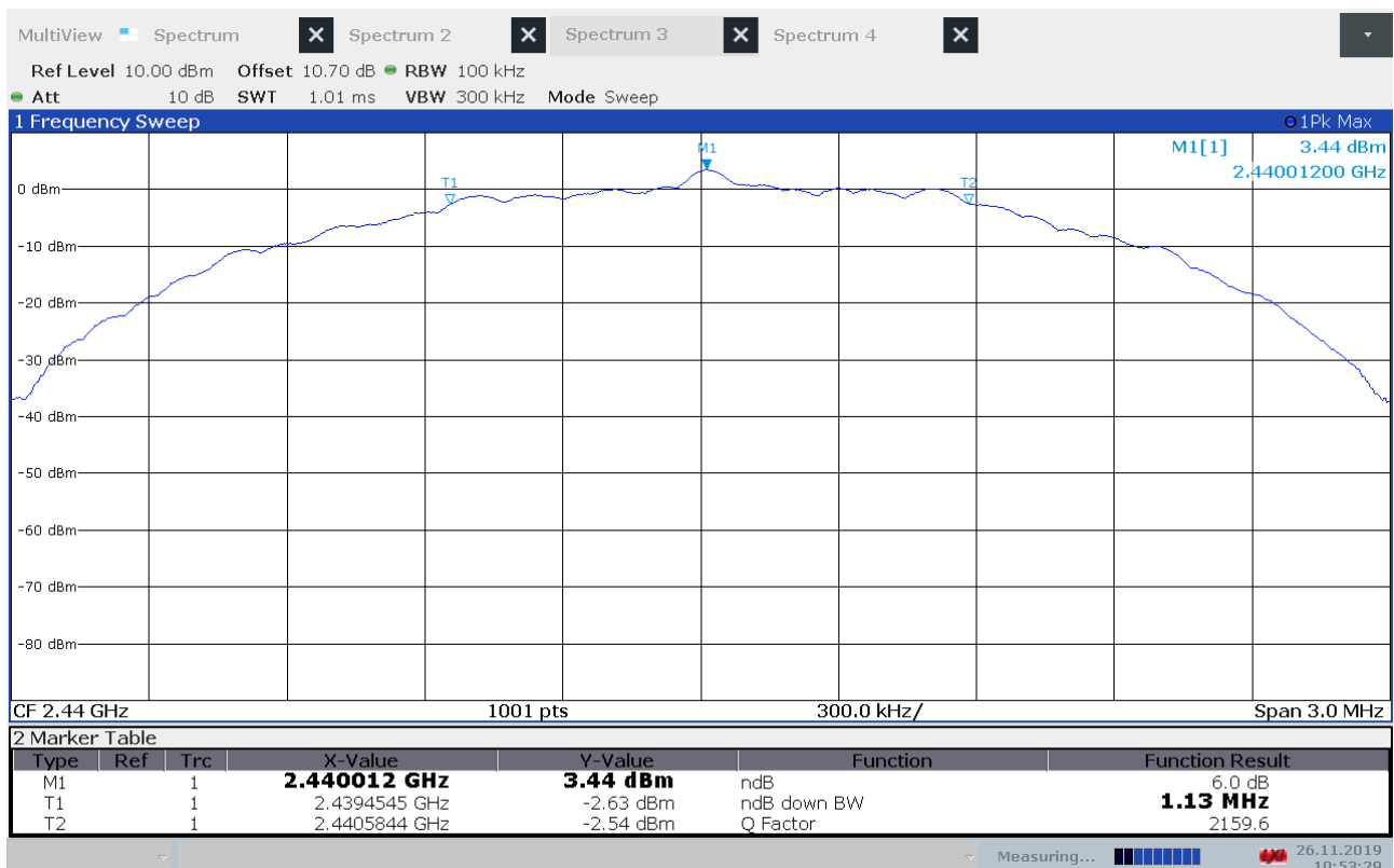
DTS Bandwidth, 2440 MHz, BT LE 2Mb
