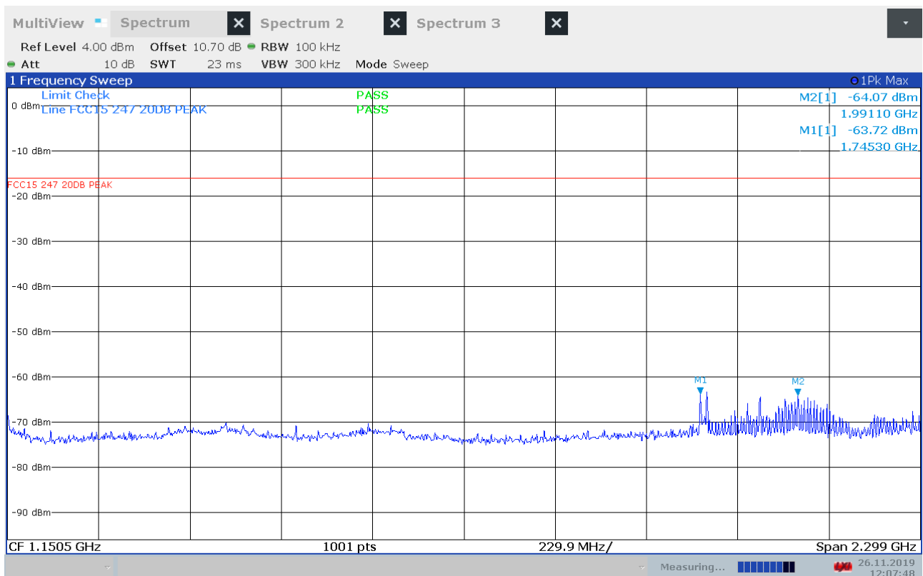
Conducted Emissions, 1 – 2300 MHz, 2440 MHz, BT LE LR
