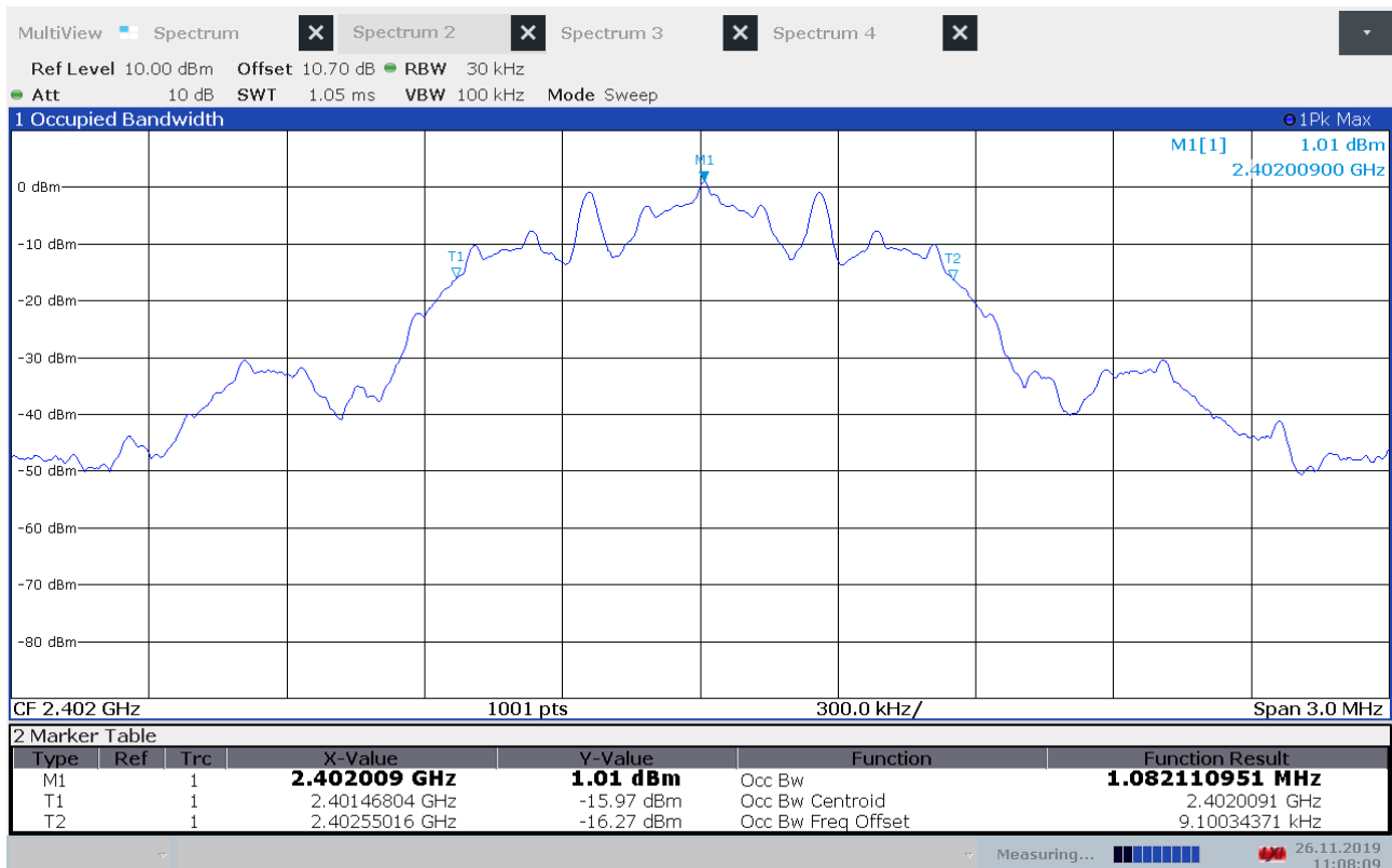
99% Bandwidth, 2402 MHz, BT LE LR
