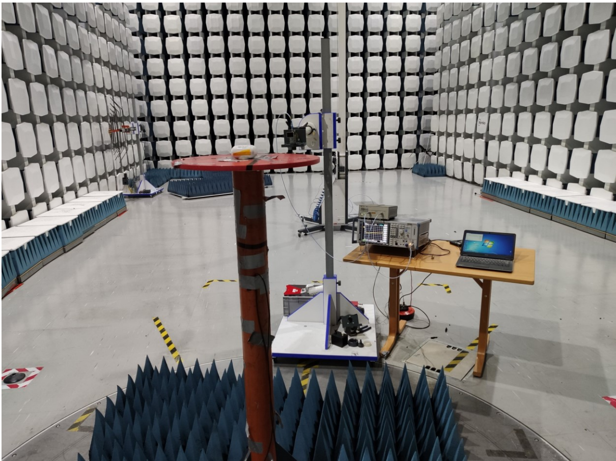
Radiated emissions, 18 – 26 GHz
