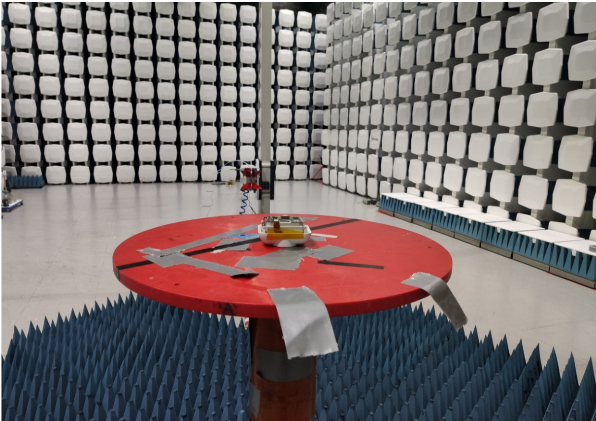
Radiated emissions, 3 – 18 GHz
