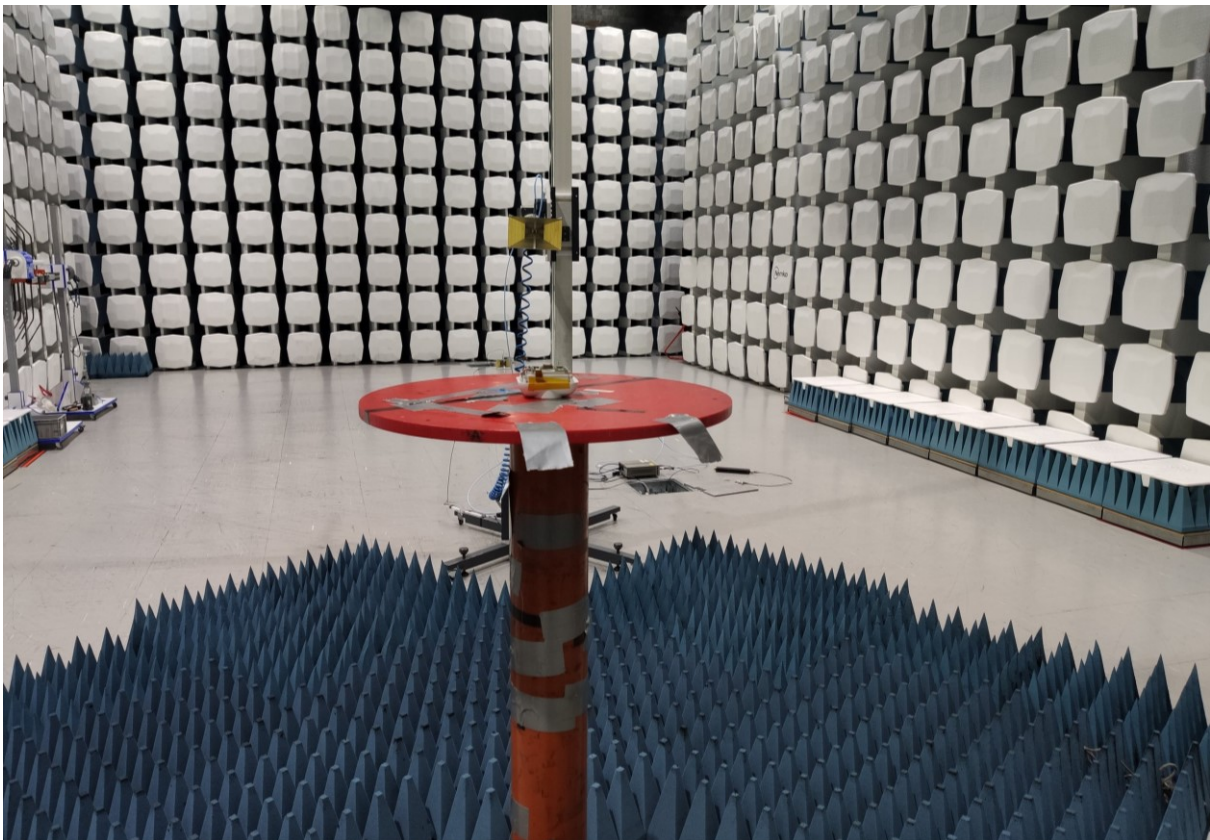
Radiated emissions, 1 – 4 GHz
