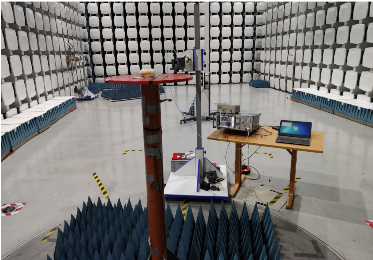
Radiated emissions, 18 – 26 GHz
