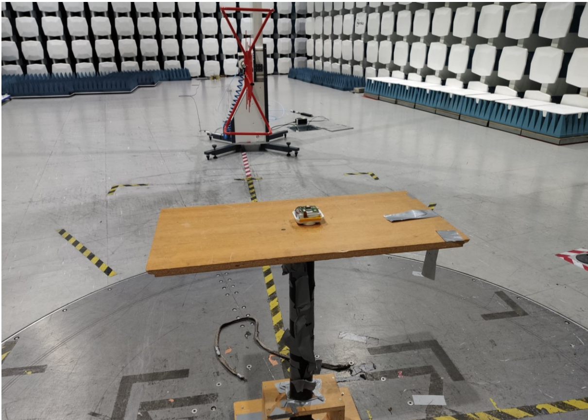
Radiated emissions, 30 - 200 MHz
