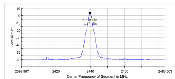
O-QPSK MIDDLE CHANNEL
