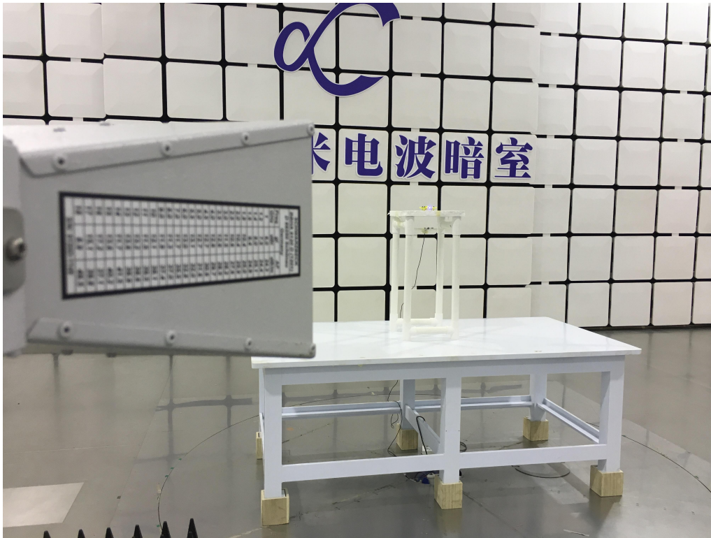
Radiated Test 5
