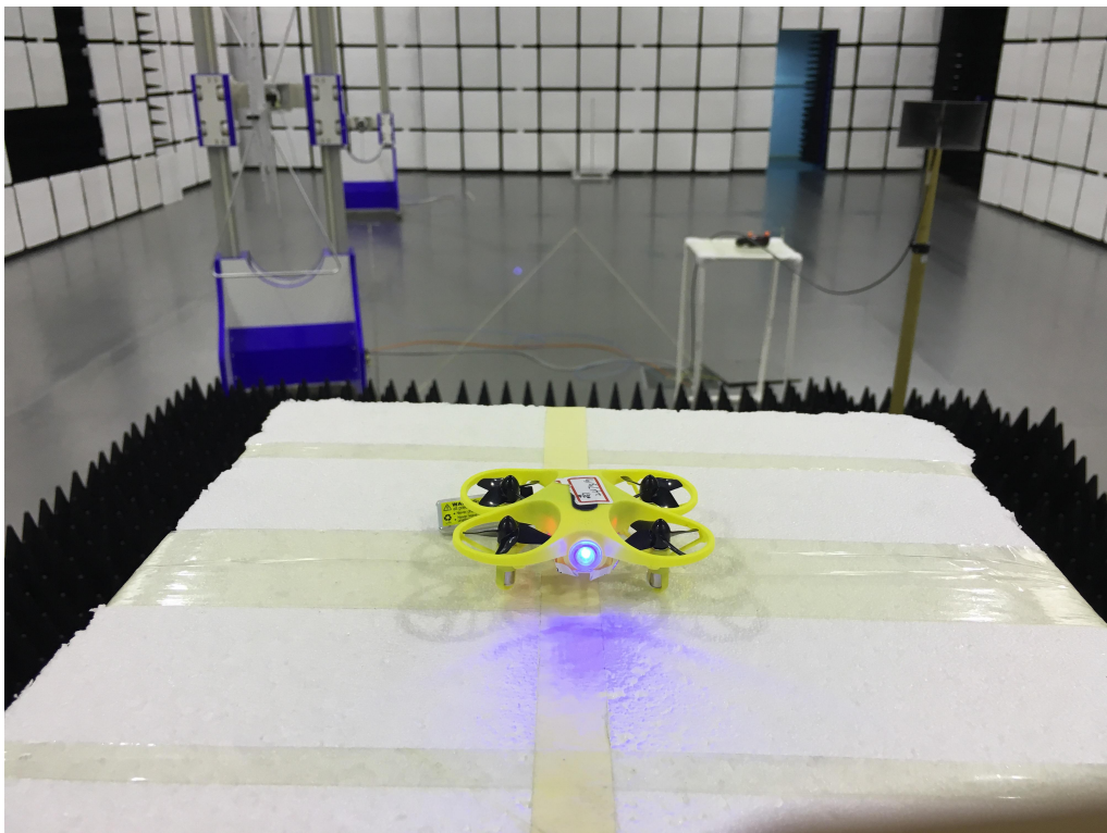
Radiated Test 6
