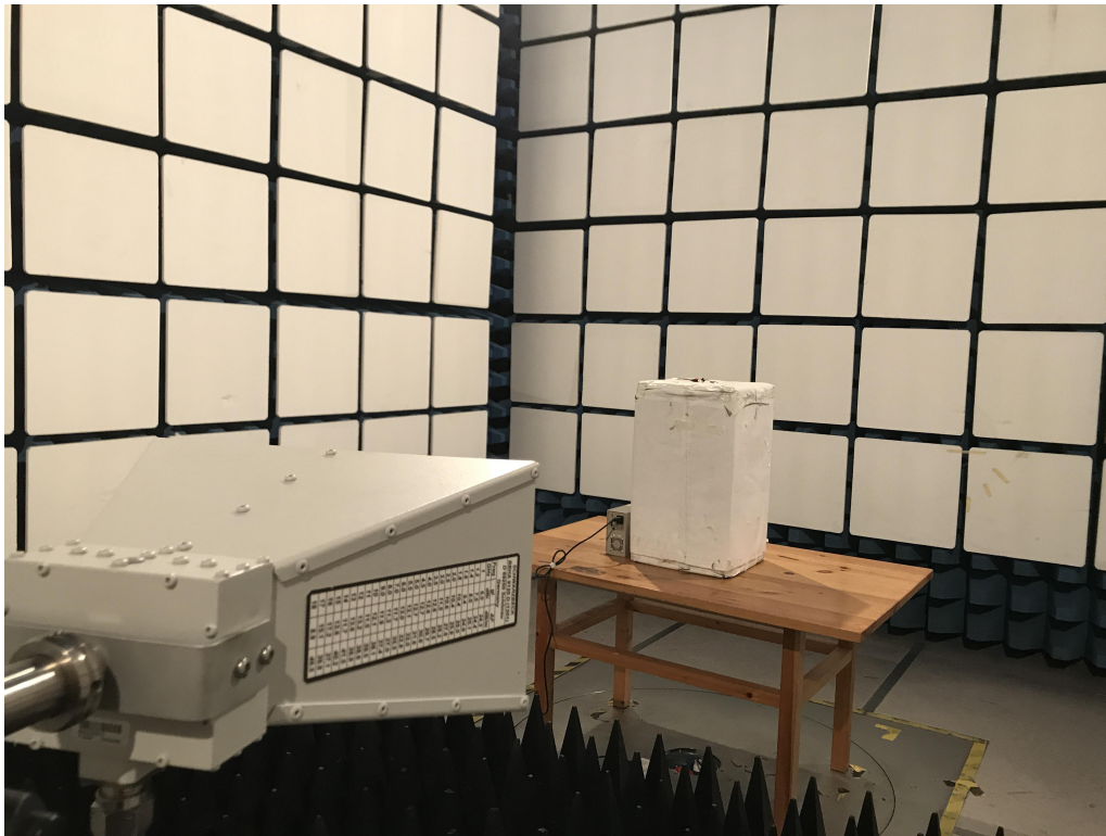
Radiated Test Photo 5
