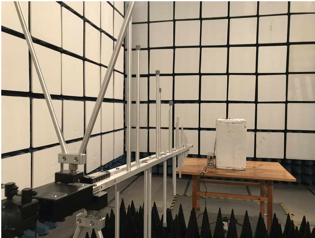
Radiated Test Photo 4
