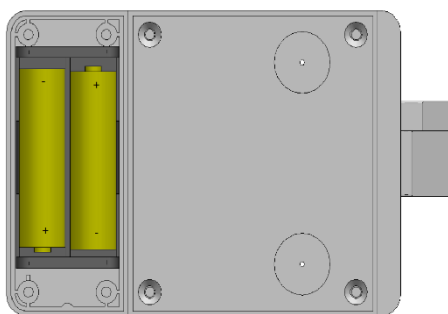
Battery replacement
