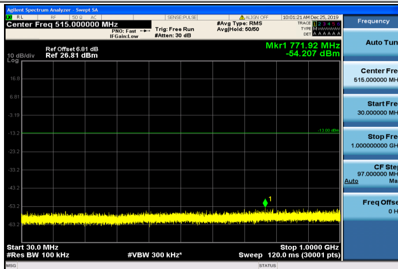
Band25-20MHz-16QAM-26590-1RB#0-30~1000MHz
