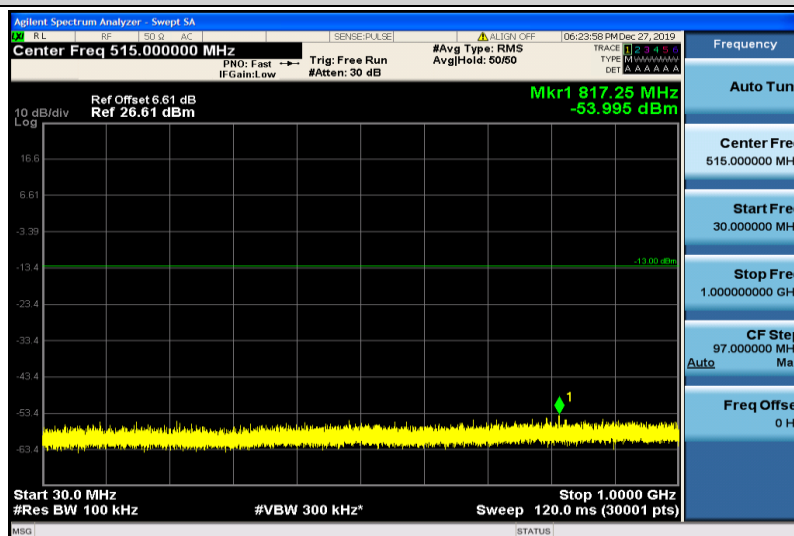
Band25-10MHz-16QAM-26640-1RB#0-30~1000MHz
