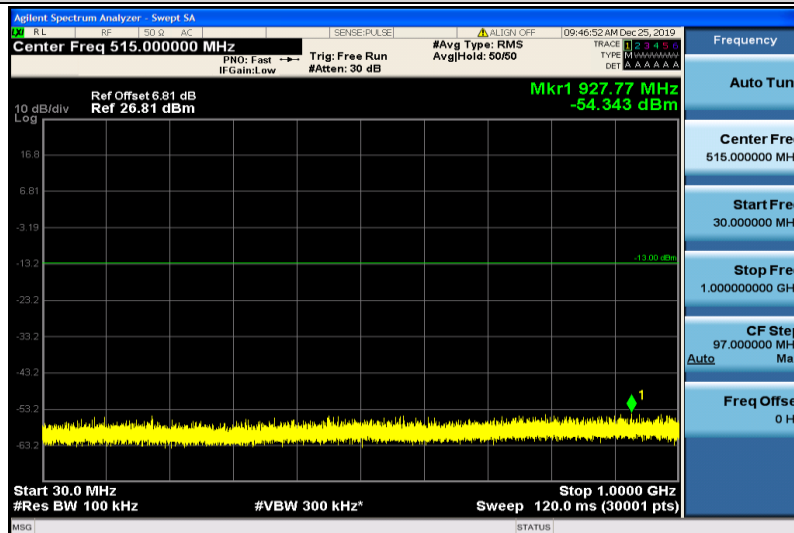
Band25-15MHz-QPSK-26365-1RB#0-30~1000MHz
