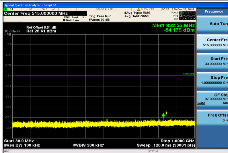
Band25-10MHz-16QAM-26365-1RB#0-30~1000MHz
