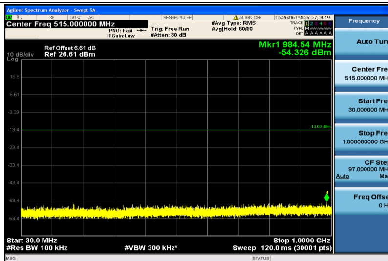
Band25-15MHz-16QAM-26115-1RB#0-30~1000MHz
