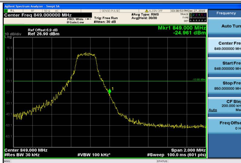
Band26-3MHz-QPSK-27025-1RB#14
