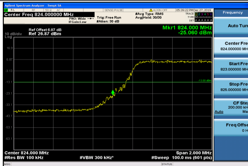
Band26-5MHz-QPSK-26815-25RB#0
