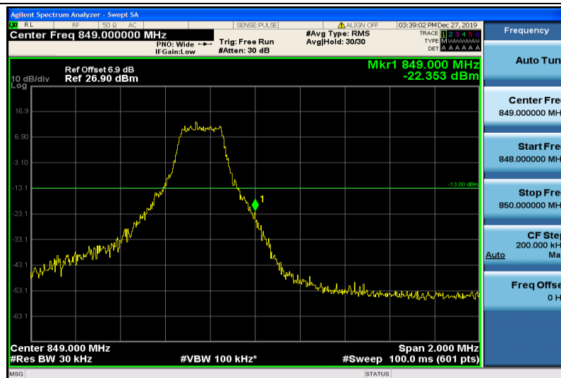
Band26-3MHz-16QAM-27025-1RB#14
