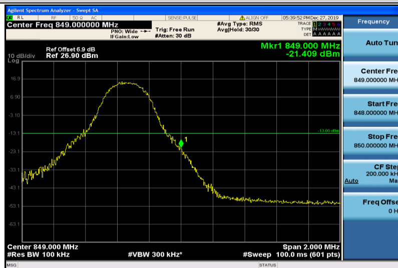
Band26-5MHz-16QAM-27015-1RB#24
