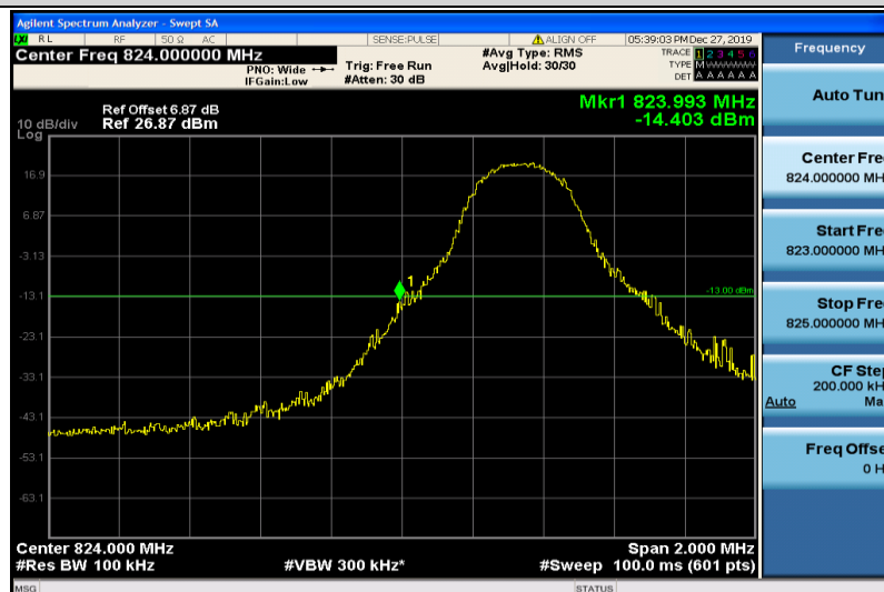
Band26-5MHz-QPSK-26815-1RB#0
