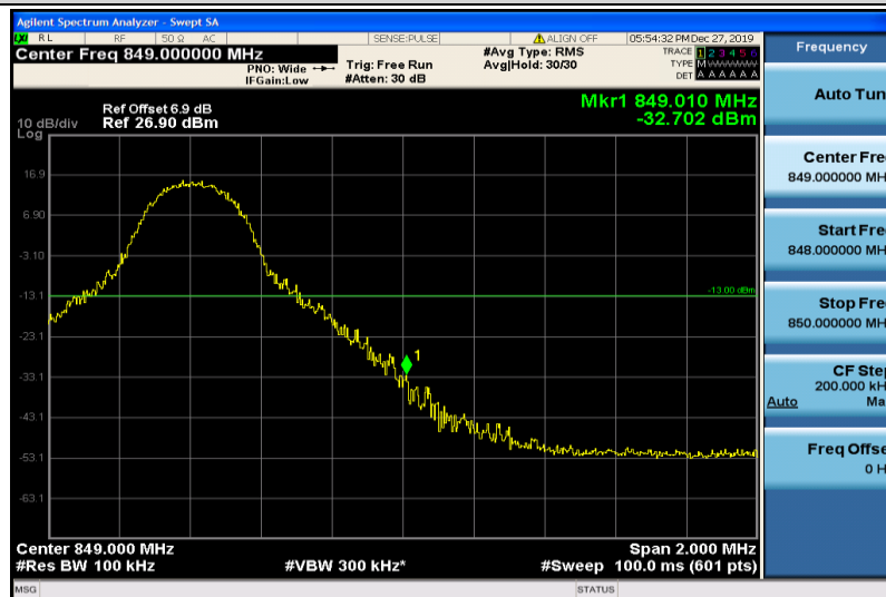
Band26-10MHz-16QAM-26990-1RB#49
