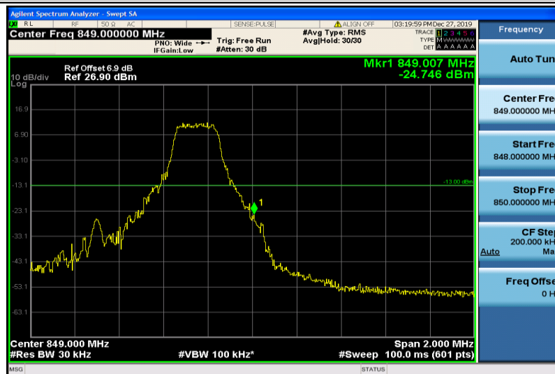
Band26-1.4MHz-16QAM-27033-1RB#5
