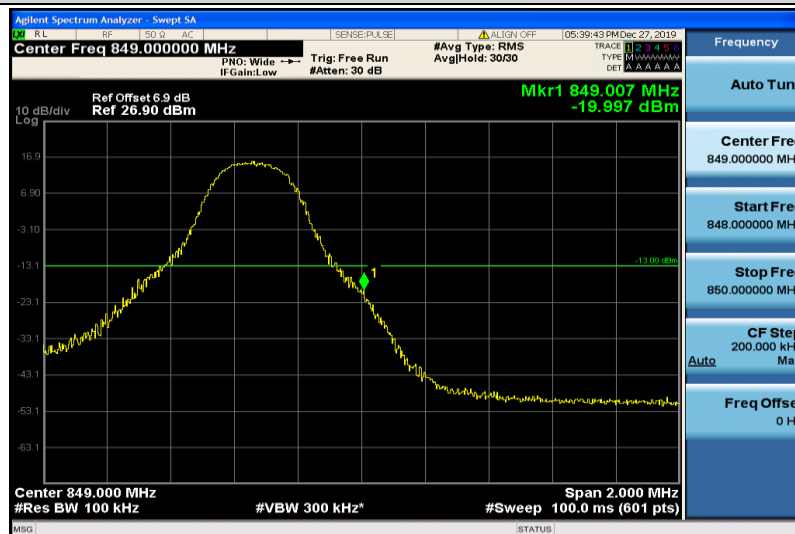
Band26-5MHz-QPSK-27015-1RB#24
