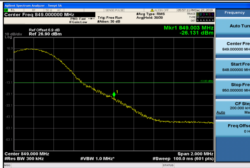
Band26-15MHz-16QAM-26965-1RB#74
