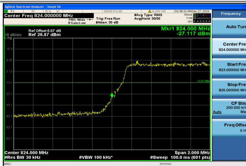
Band26-3MHz-QPSK-26805-15RB#0
