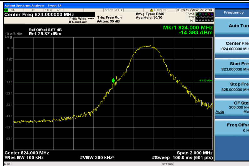
Band26-5MHz-16QAM-26815-1RB#0
