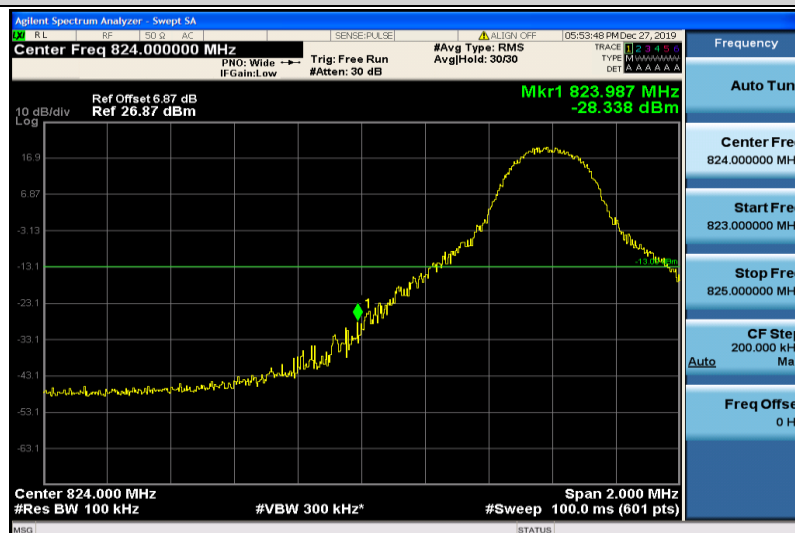
Band26-10MHz-16QAM-26840-1RB#0
