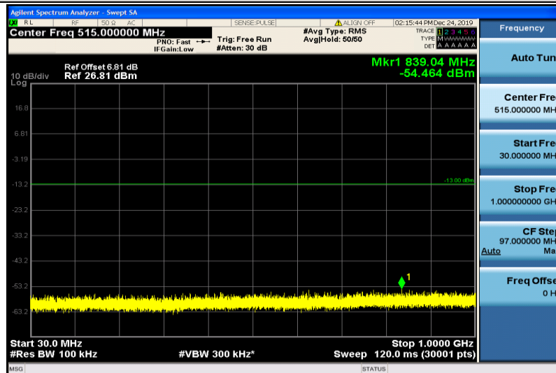
Band2-1.4MHz-16QAM-18900-1RB#0-30~1000MHz
