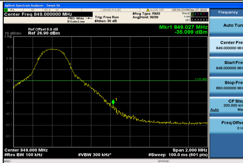
Band26-10MHz-QPSK-26990-1RB#49
