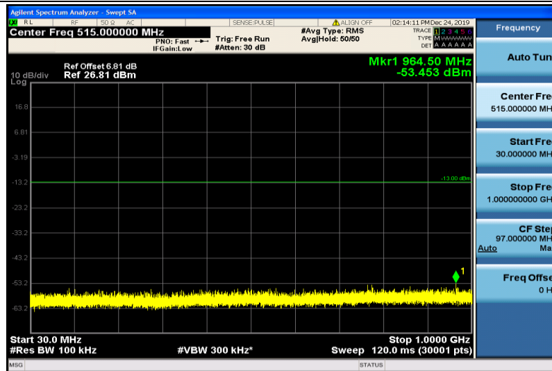
Band2-1.4MHz-16QAM-18607-1RB#0-30~1000MHz
