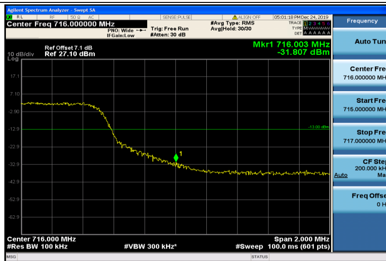
Band17-10MHz-16QAM-23800-50RB#0
