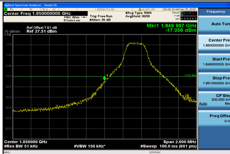
Band25-5MHz-QPSK-26065-1RB#0
