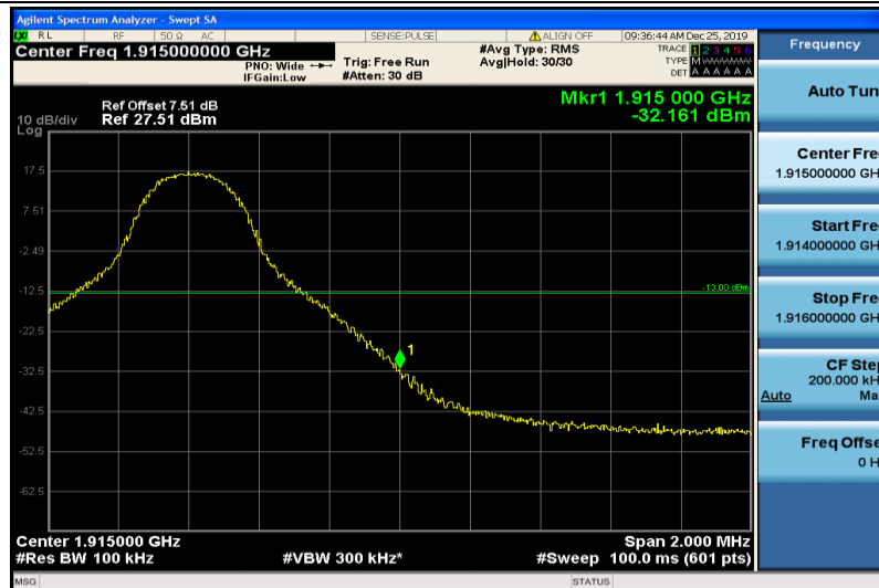
Band25-10MHz-QPSK-26640-1RB#49
