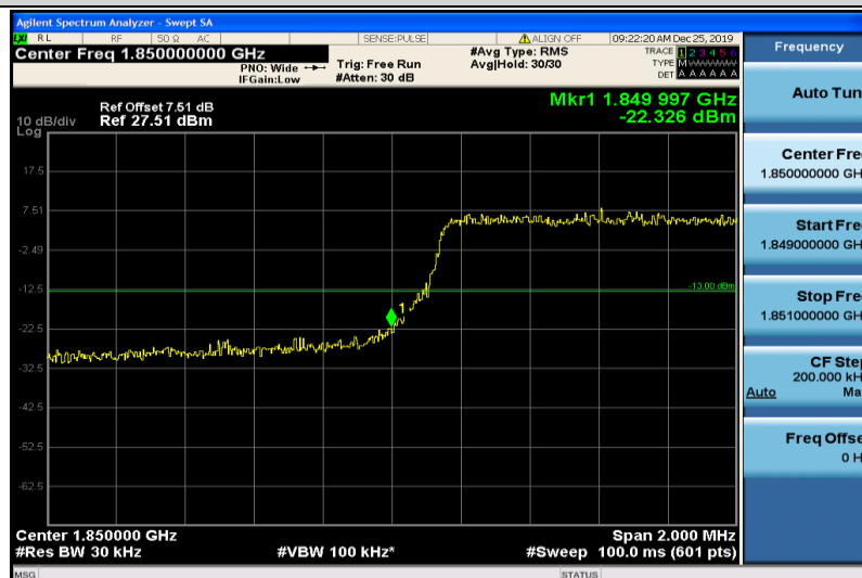
Band25-3MHz-16QAM-26055-15RB#0
