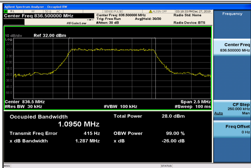
Band26-1.4MHz-16QAM-26915-6RB#0-1.0950
