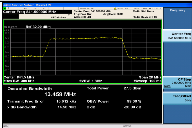
Band26-15MHz-16QAM-26965-75RB#0-13.458
