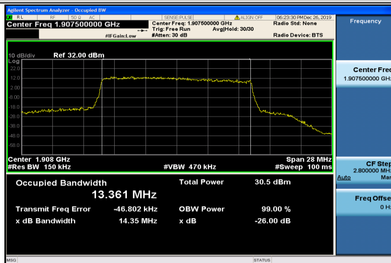
Band25-15MHz-16QAM-26615-75RB#0-13.361
