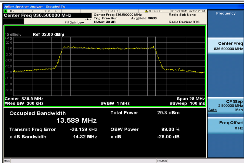
Band26-15MHz-16QAM-26915-75RB#0-13.589
