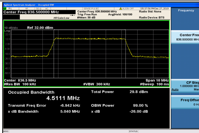
Band26-5MHz-QPSK-26915-25RB#0-4.5111
