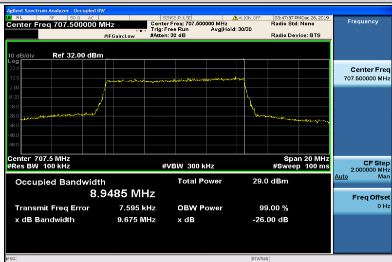
Band12-10MHz-QPSK-23095-50RB#0-8.9485
