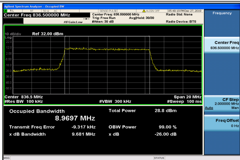
Band26-10MHz-16QAM-26915-50RB#0-8.9697
