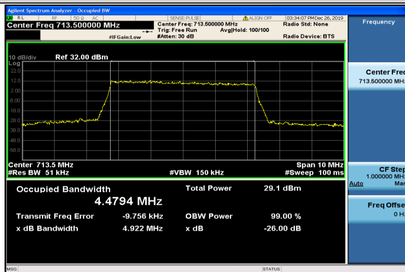
Band12-5MHz-QPSK-23155-25RB#0-4.4794
