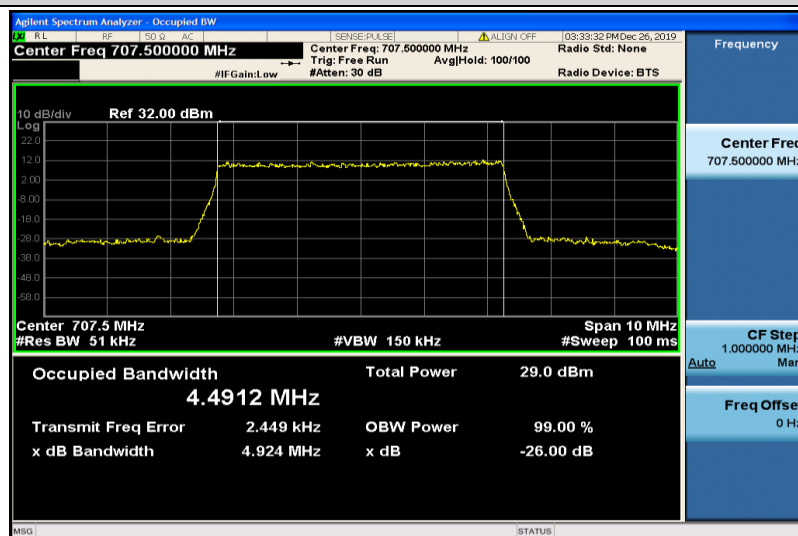
Band12-5MHz-QPSK-23095-25RB#0-4.4912
