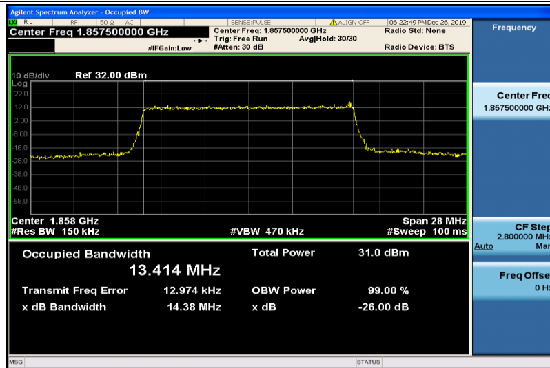
Band25-15MHz-16QAM-26115-75RB#0-13.414
