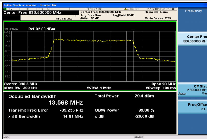
Band26-15MHz-QPSK-26915-75RB#0-13.568
