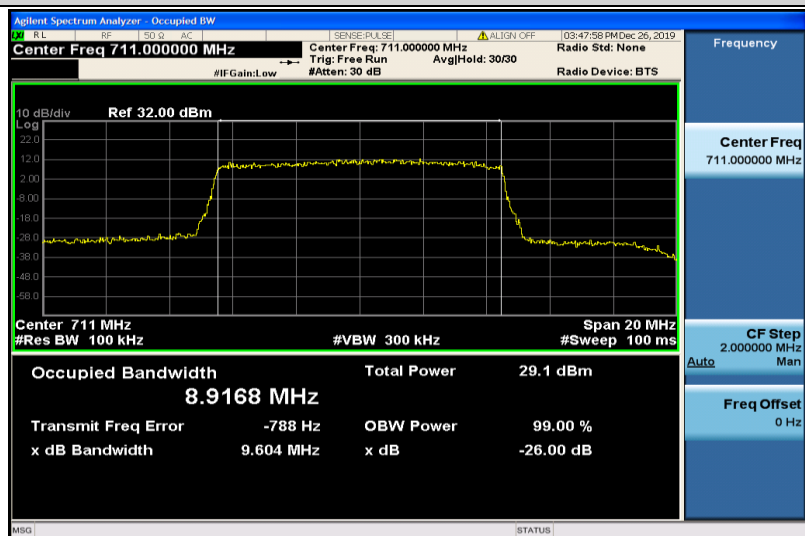
Band12-10MHz-QPSK-23130-50RB#0-8.9168
