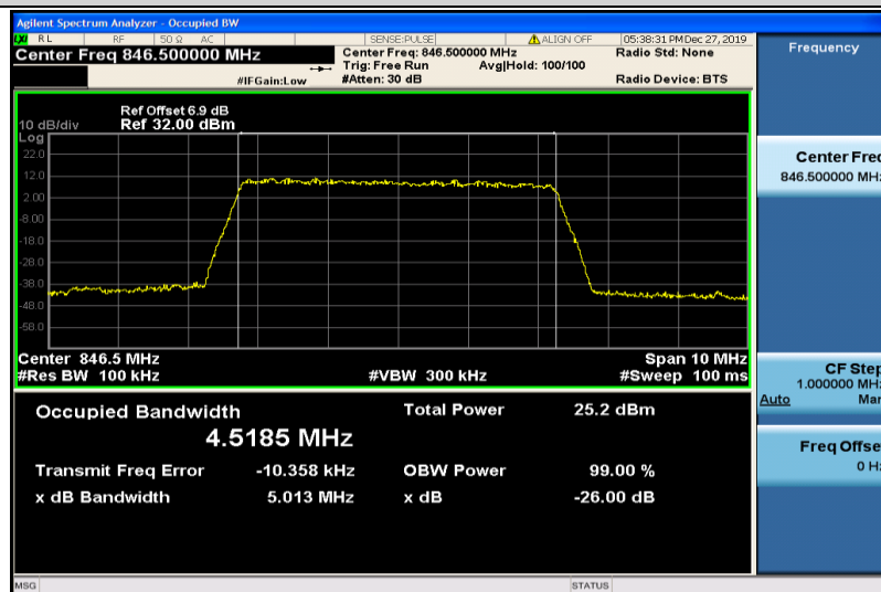
Band26-5MHz-QPSK-27015-25RB#0-4.5185
