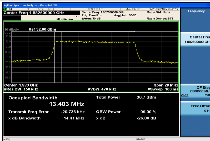
Band25-15MHz-16QAM-26365-75RB#0-13.403
