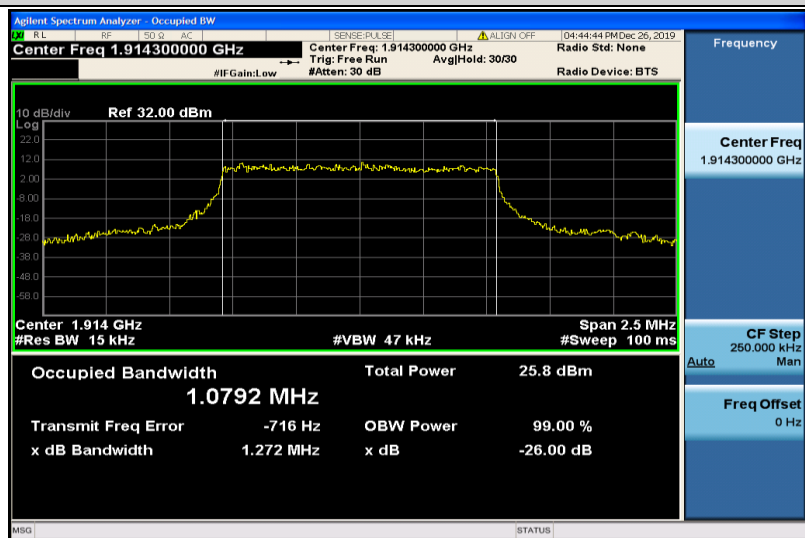
Band25-1.4MHz-16QAM-26683-6RB#0-1.0792
