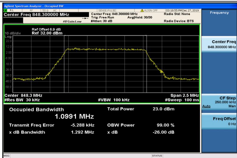
Band26-1.4MHz-16QAM-27033-6RB#0-1.0991
