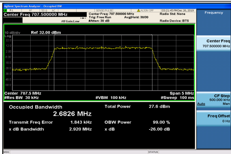
Band12-3MHz-16QAM-23095-15RB#0-2.6826
