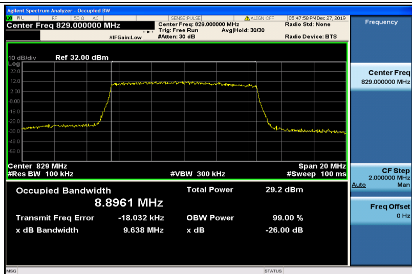
Band26-10MHz-16QAM-26840-50RB#0-8.8961
