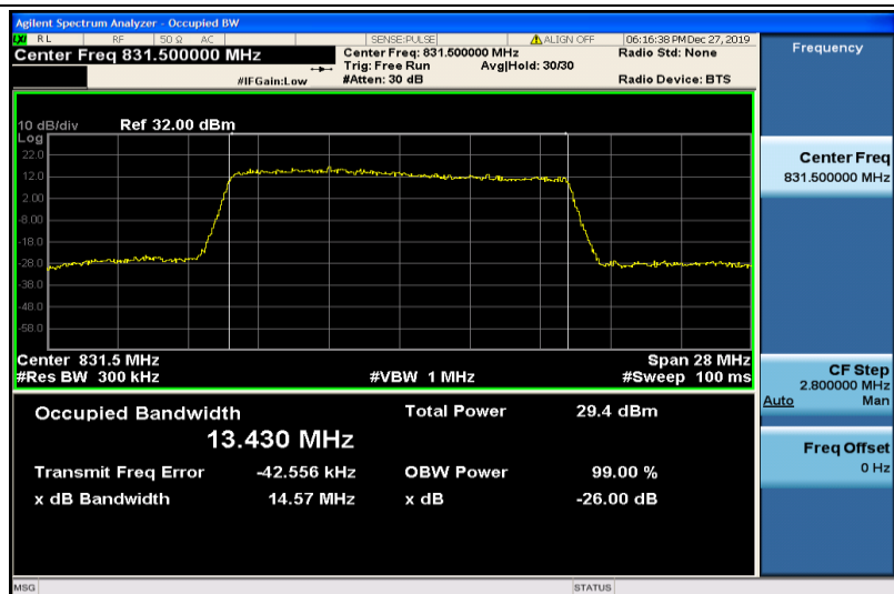
Band26-15MHz-16QAM-26865-75RB#0-13.430
