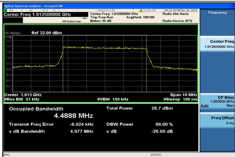
Band25-5MHz-QPSK-26665-25RB#0-4.4888
