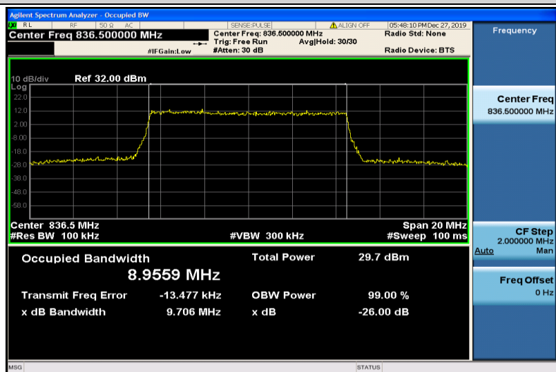
Band26-10MHz-QPSK-26915-50RB#0-8.9559
