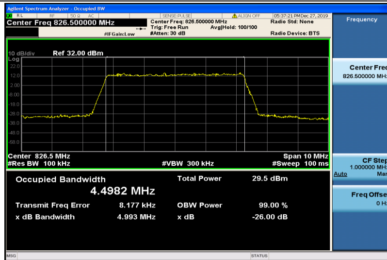
Band26-5MHz-QPSK-26815-25RB#0-4.4982
