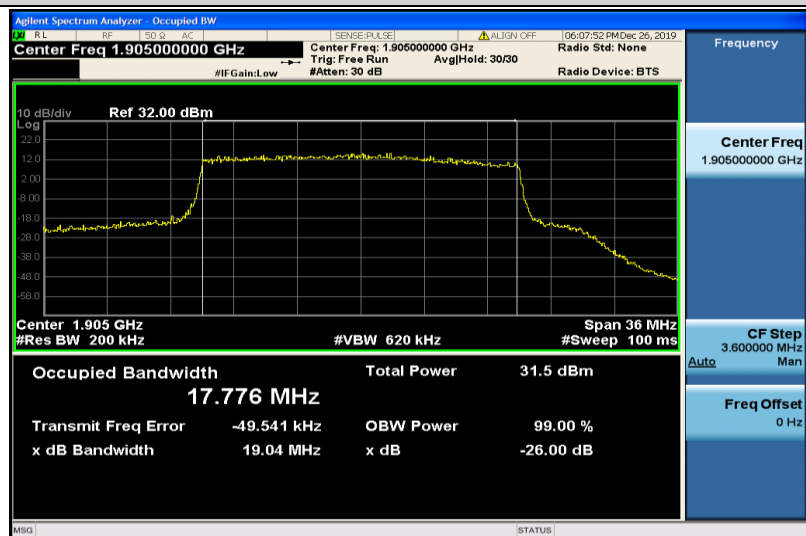
Band25-20MHz-QPSK-26590-100RB#0-17.776
