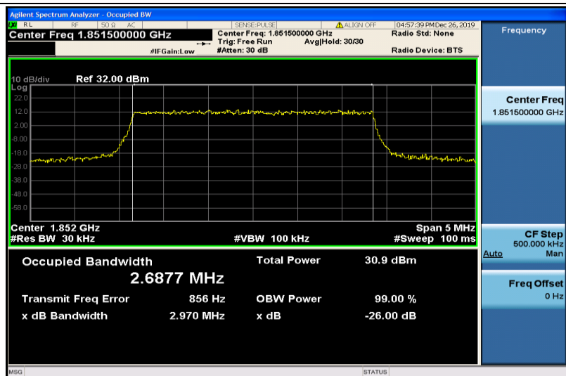
Band25-3MHz-QPSK-26055-15RB#0-2.6877
