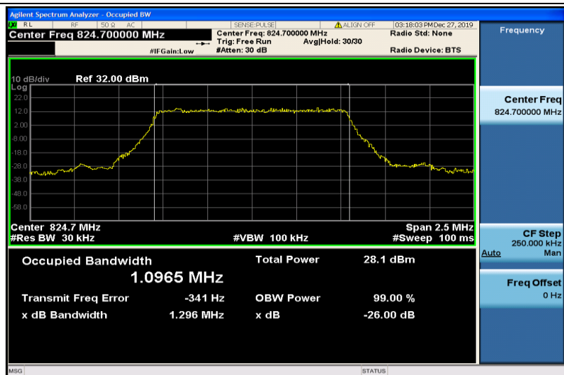
Band26-1.4MHz-QPSK-26797-6RB#0-1.0965
