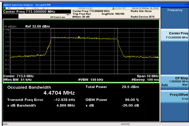
Band17-5MHz-16QAM-23825-25RB#0-4.4704
