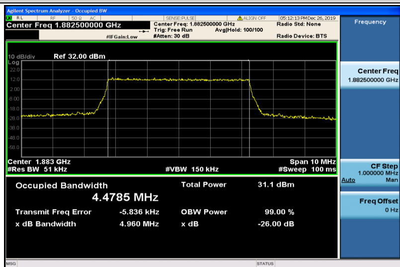
Band25-5MHz-QPSK-26365-25RB#0-4.4785
