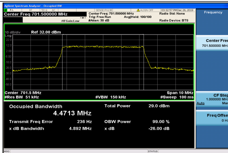
Band12-5MHz-QPSK-23035-25RB#0-4.4713
