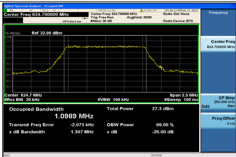
Band26-1.4MHz-16QAM-26797-6RB#0-1.0989
