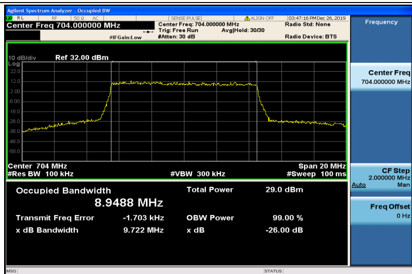
Band12-10MHz-QPSK-23060-50RB#0-8.9488
