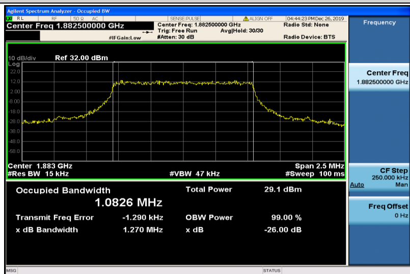
Band25-1.4MHz-16QAM-26365-6RB#0-1.0826
