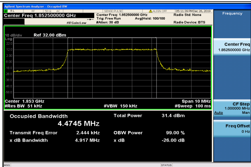
Band25-5MHz-QPSK-26065-25RB#0-4.4745
