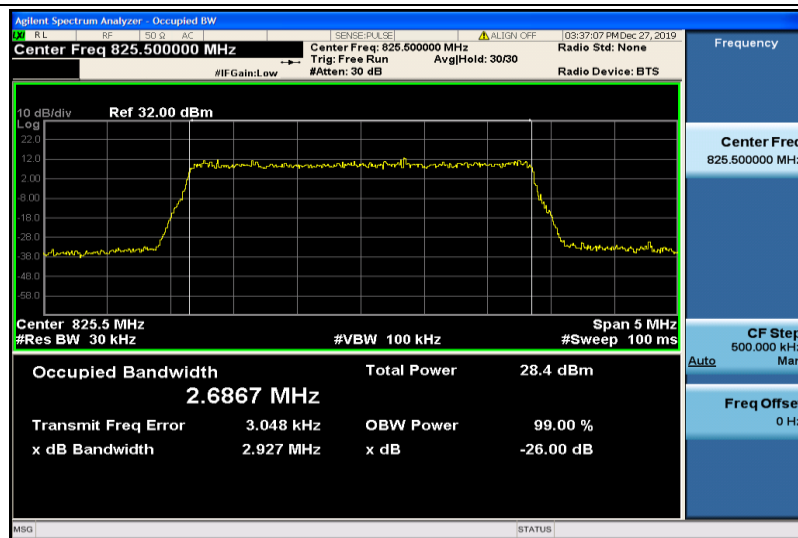
Band26-3MHz-QPSK-26805-15RB#0-2.6867
