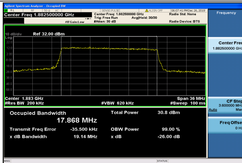
Band25-20MHz-16QAM-26365-100RB#0-17.868
