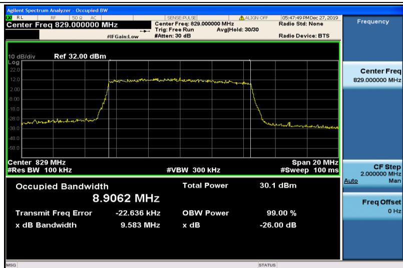
Band26-10MHz-QPSK-26840-50RB#0-8.9062
