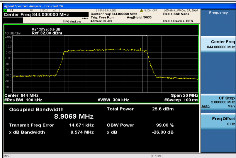
Band26-10MHz-16QAM-26990-50RB#0-8.9069
