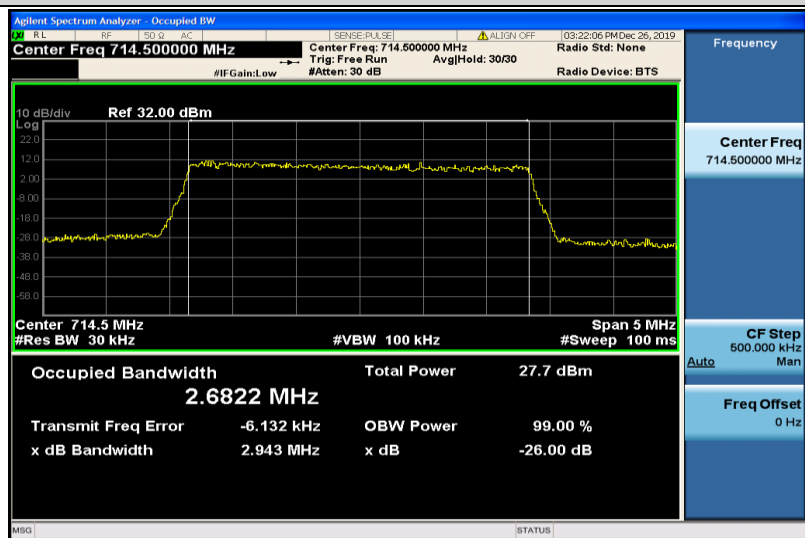
Band12-3MHz-16QAM-23165-15RB#0-2.6822
