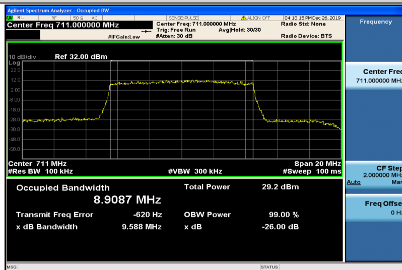
Band17-10MHz-16QAM-23800-50RB#0-8.9087
