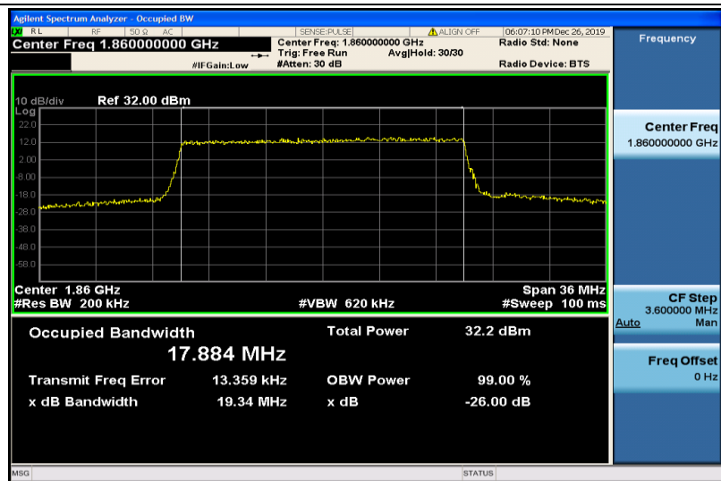
Band25-20MHz-QPSK-26140-100RB#0-17.884
