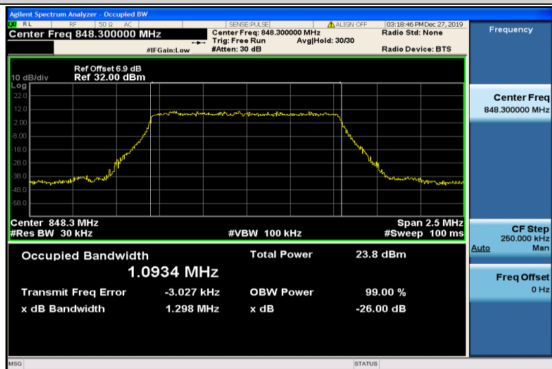
Band26-1.4MHz-QPSK-27033-6RB#0-1.0934
