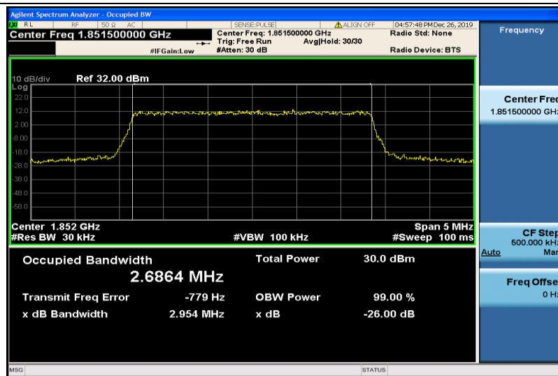
Band25-3MHz-16QAM-26055-15RB#0-2.6864
