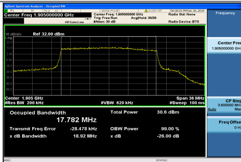
Band25-20MHz-16QAM-26590-100RB#0-17.782
