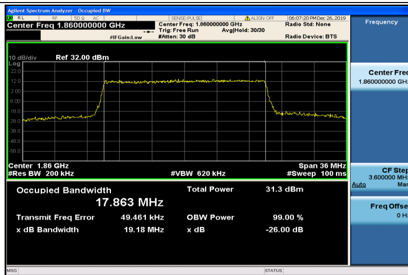
Band25-20MHz-16QAM-26140-100RB#0-17.863
