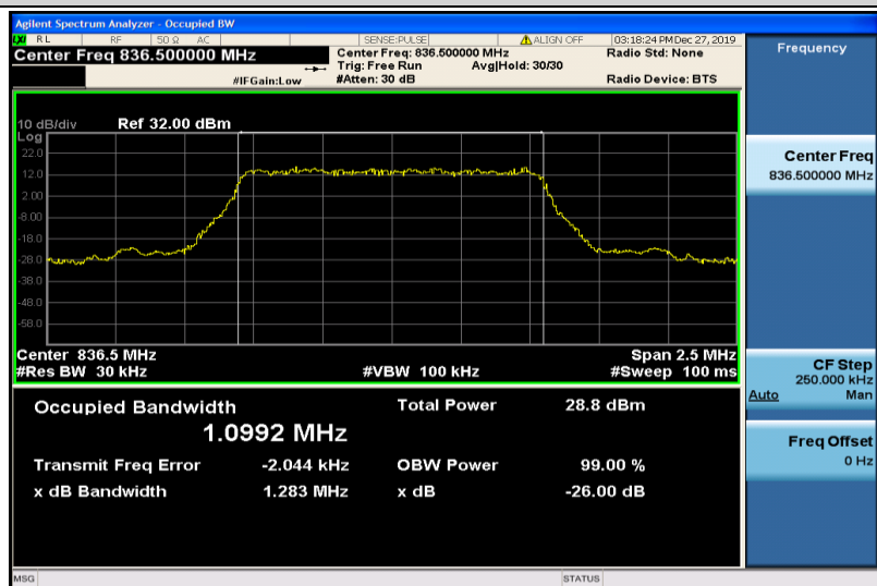
Band26-1.4MHz-QPSK-26915-6RB#0-1.0992
