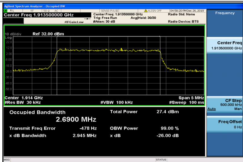
Band25-3MHz-QPSK-26675-15RB#0-2.6900
