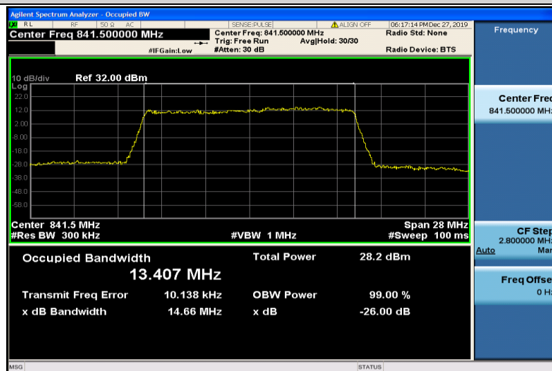
Band26-15MHz-QPSK-26965-75RB#0-13.407
