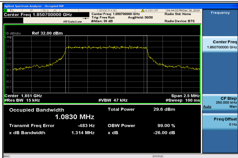
Band25-1.4MHz-16QAM-26047-6RB#0-1.0830
