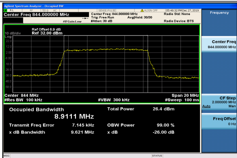
Band26-10MHz-QPSK-26990-50RB#0-8.9111
