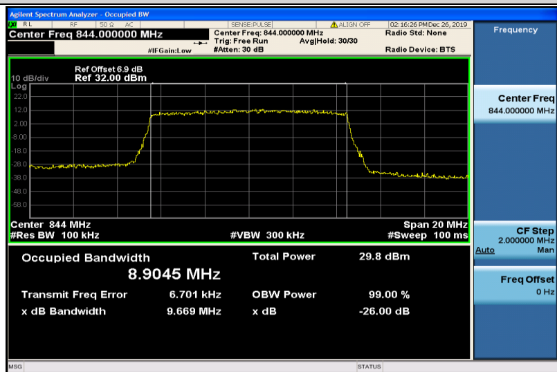
Band5-10MHz-QPSK-20600-50RB#0-8.9045
