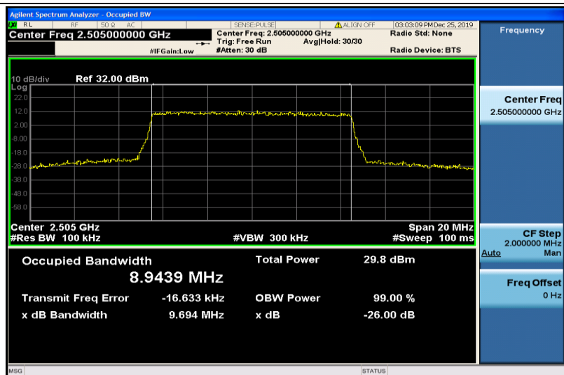
Band7-10MHz-16QAM-20800-50RB#0-8.9439
