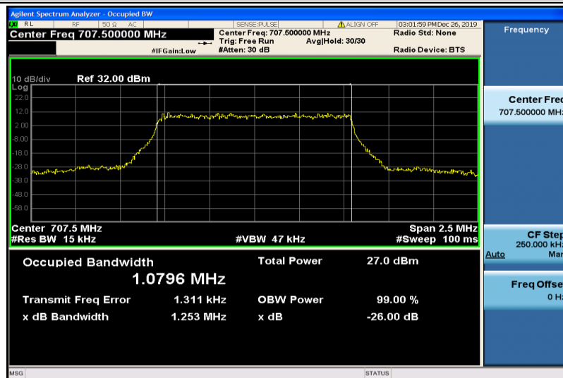
Band12-1.4MHz-16QAM-23095-6RB#0-1.0796
