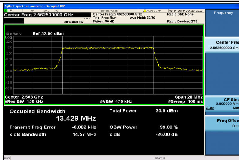
Band7-15MHz-QPSK-21375-75RB#0-13.429
