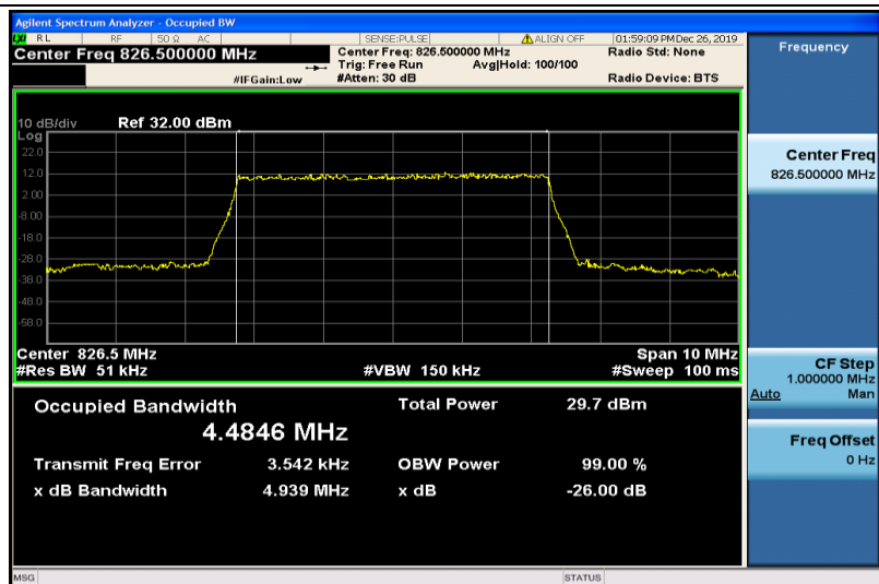
Band5-5MHz-QPSK-20425-25RB#0-4.4846
