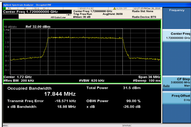
Band4-20MHz-QPSK-20050-100RB#0-17.844
