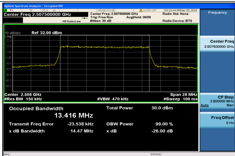
Band7-15MHz-16QAM-20825-75RB#0-13.416
