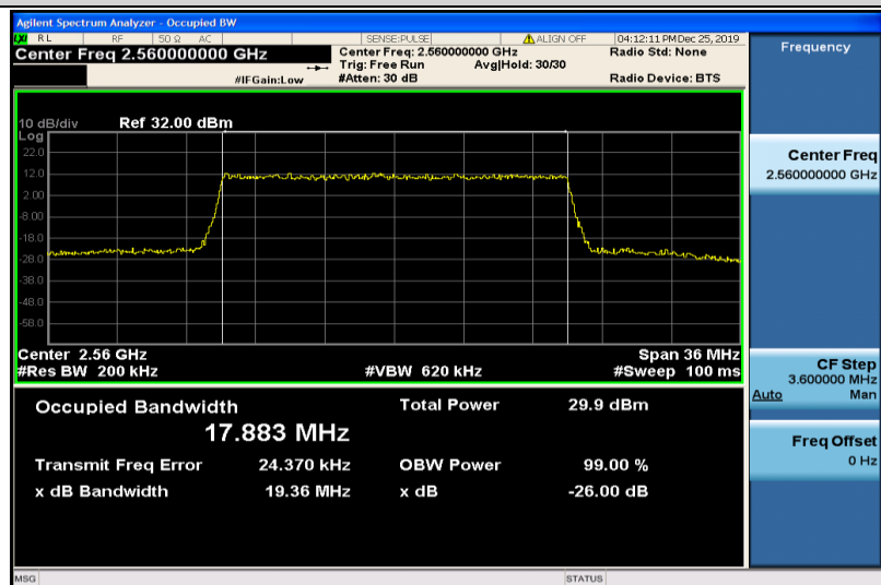
Band7-20MHz-16QAM-21350-100RB#0-17.883
