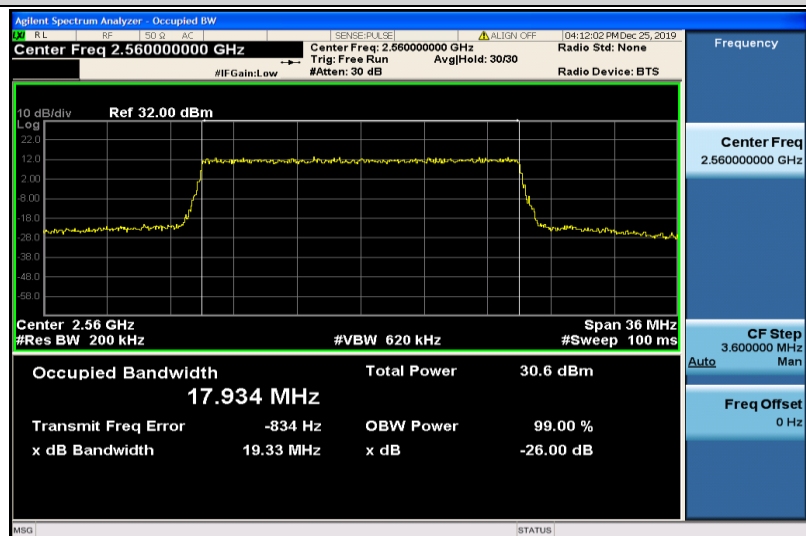
Band7-20MHz-QPSK-21350-100RB#0-17.934
