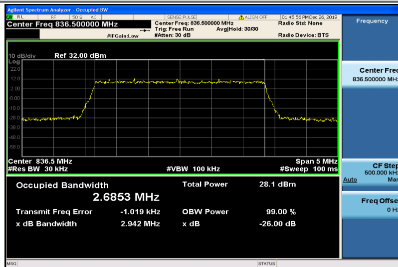
Band5-3MHz-16QAM-20525-15RB#0-2.6853
