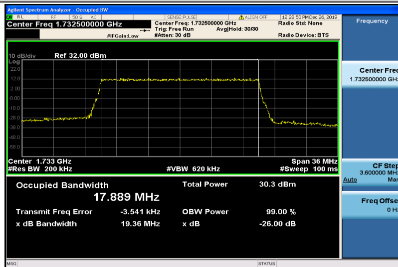
Band4-20MHz-16QAM-20175-100RB#0-17.889
