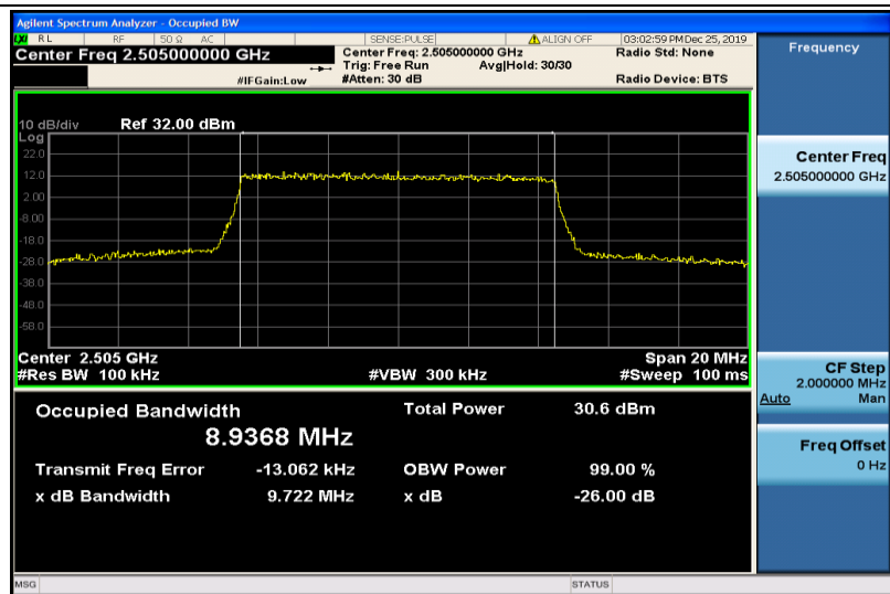
Band7-10MHz-QPSK-20800-50RB#0-8.9368
