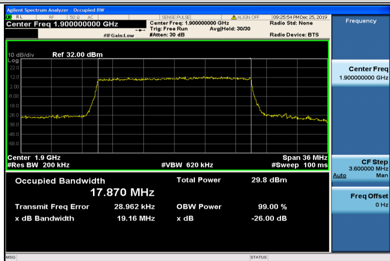
Band2-20MHz-16QAM-19100-100RB#0-17.870
