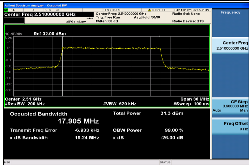
Band7-20MHz-QPSK-20850-100RB#0-17.905
