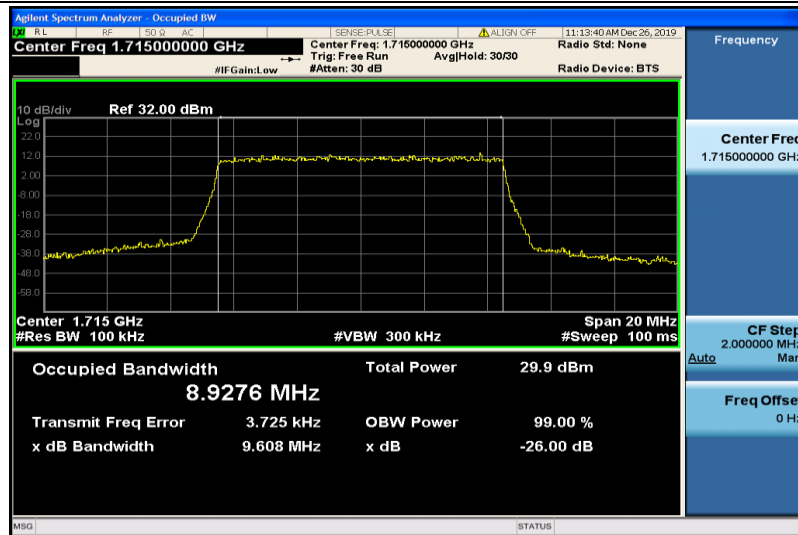
Band4-10MHz-16QAM-20000-50RB#0-8.9276
