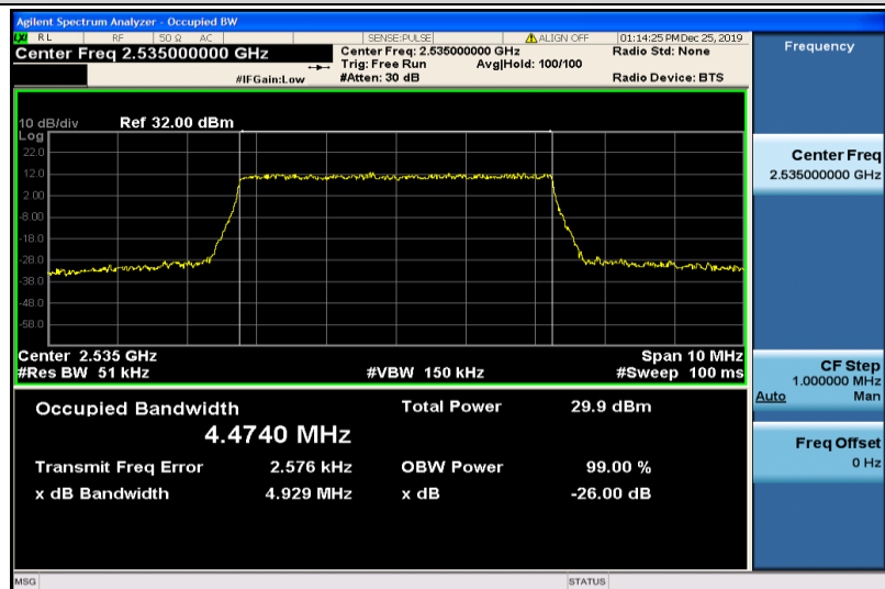
Band7-5MHz-QPSK-21100-25RB#0-4.4740
