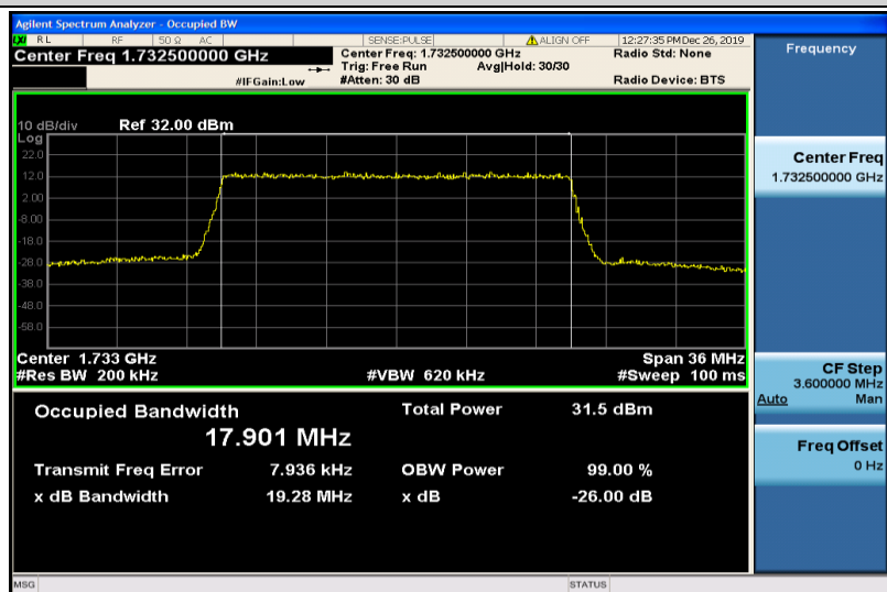
Band4-20MHz-QPSK-20175-100RB#0-17.901
