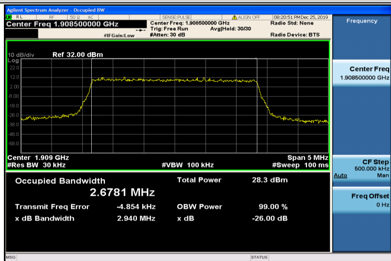
Band2-3MHz-16QAM-19185-15RB#0-2.6781
