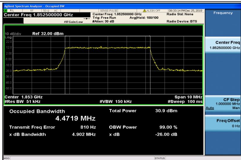
Band2-5MHz-QPSK-18625-25RB#0-4.4719
