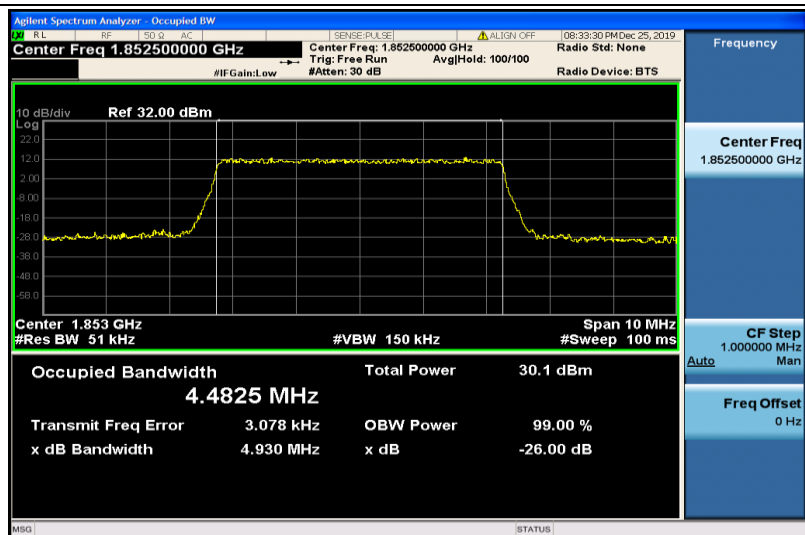
Band2-5MHz-16QAM-18625-25RB#0-4.4825
