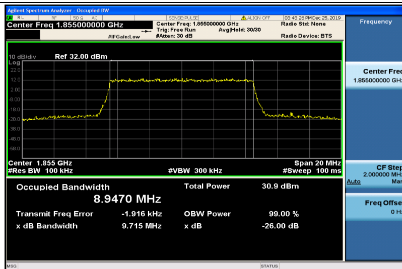
Band2-10MHz-QPSK-18650-50RB#0-8.9470
