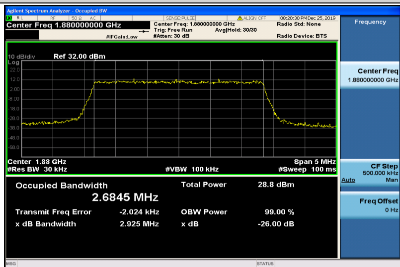
Band2-3MHz-16QAM-18900-15RB#0-2.6845
