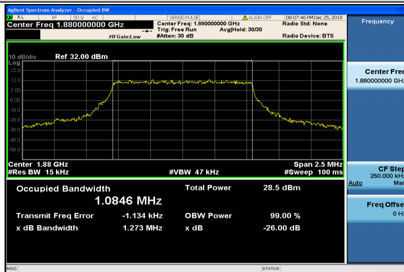
Band2-1.4MHz-16QAM-18900-6RB#0-1.0846
