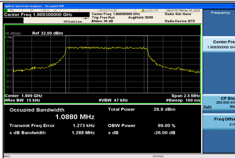
Band2-1.4MHz-QPSK-19193-6RB#0-1.0880
