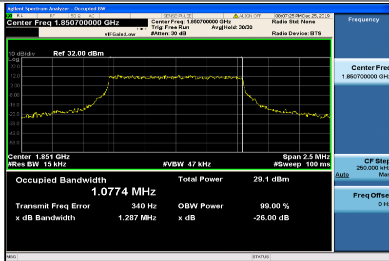
Band2-1.4MHz-16QAM-18607-6RB#0-1.0774
