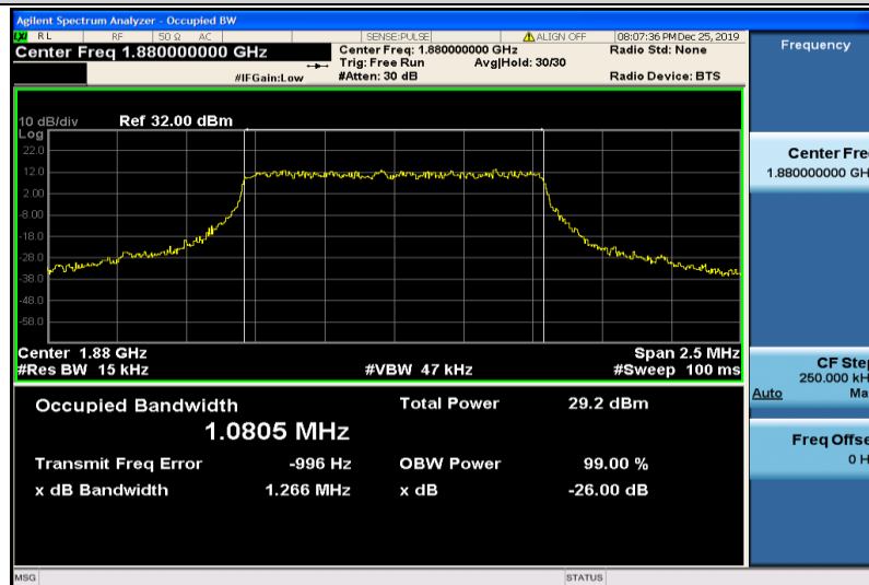
Band2-1.4MHz-QPSK-18900-6RB#0-1.0805
