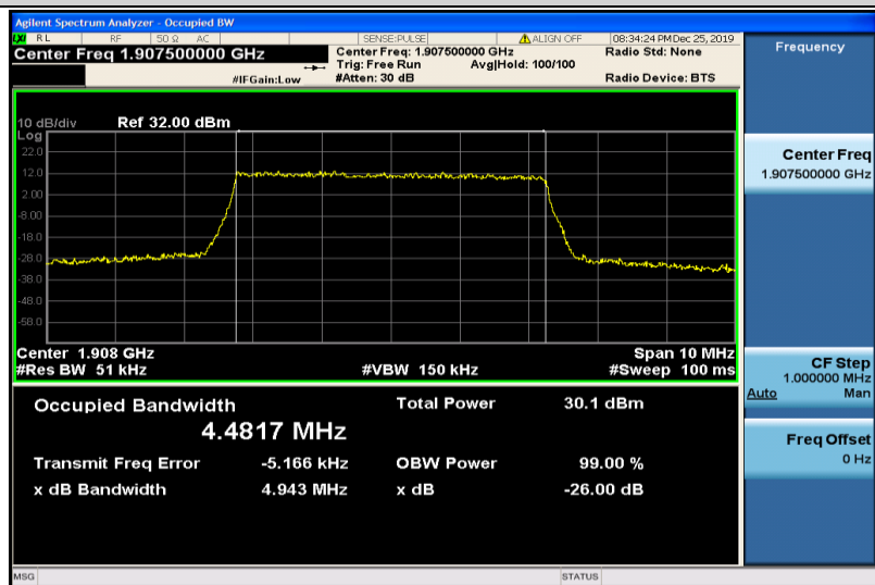
Band2-5MHz-QPSK-19175-25RB#0-4.4817
