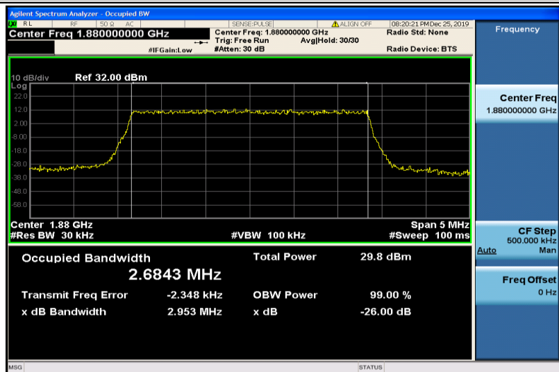
Band2-3MHz-QPSK-18900-15RB#0-2.6843
