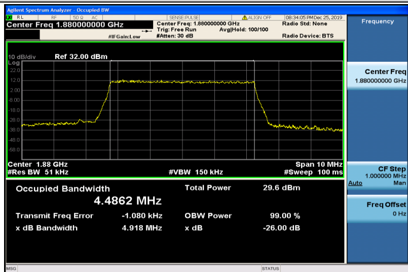
Band2-5MHz-16QAM-18900-25RB#0-4.4862
