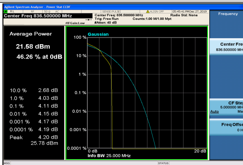
Band26-5MHz-16QAM-26915-1RB#0
