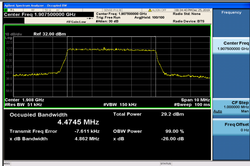
Band2-5MHz-16QAM-19175-25RB#0-4.4745
