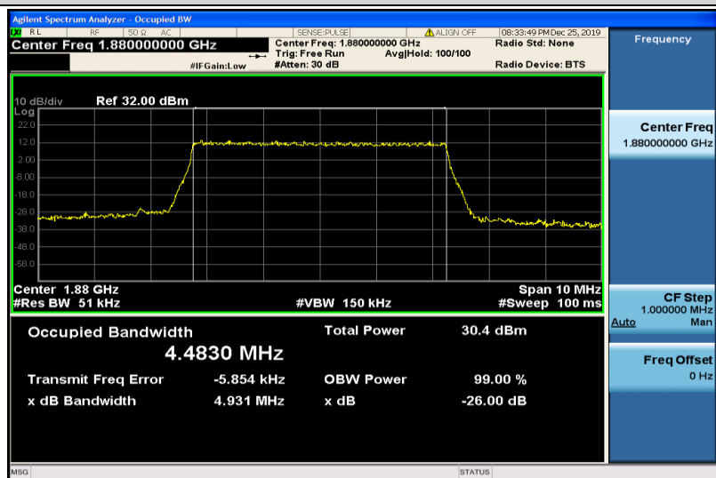
Band2-5MHz-QPSK-18900-25RB#0-4.4830
