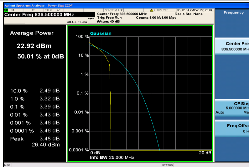
Band26-10MHz-QPSK-26915-1RB#0
