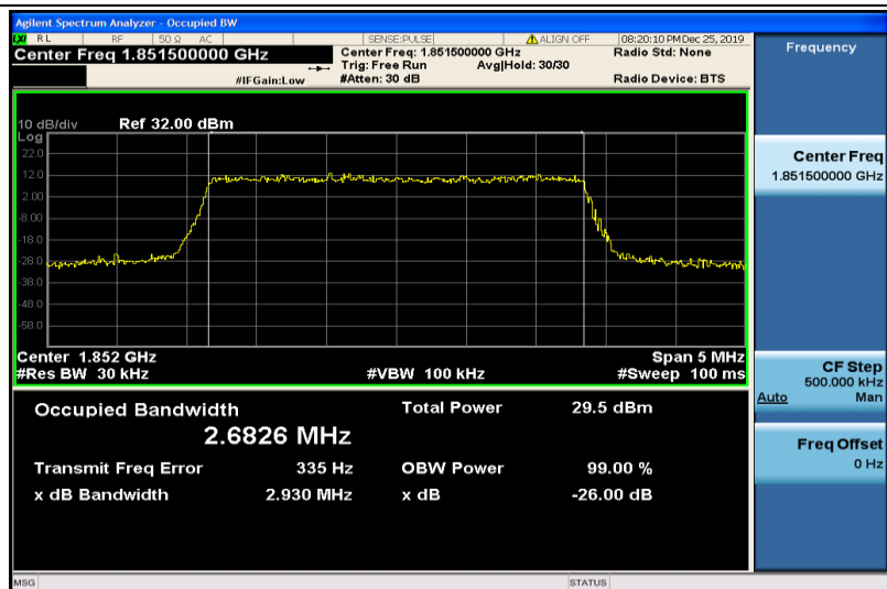
Band2-3MHz-16QAM-18615-15RB#0-2.6826
