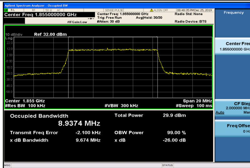
Band2-10MHz-16QAM-18650-50RB#0-8.9374
