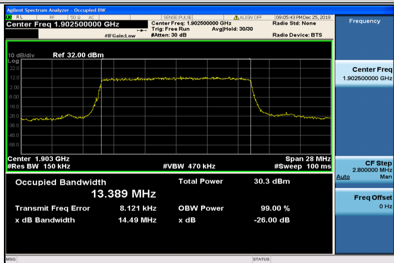
Band2-15MHz-QPSK-19125-75RB#0-13.389
