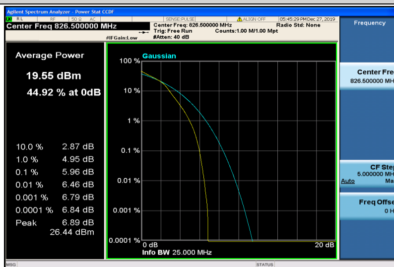
Band26-5MHz-16QAM-26815-25RB#0
