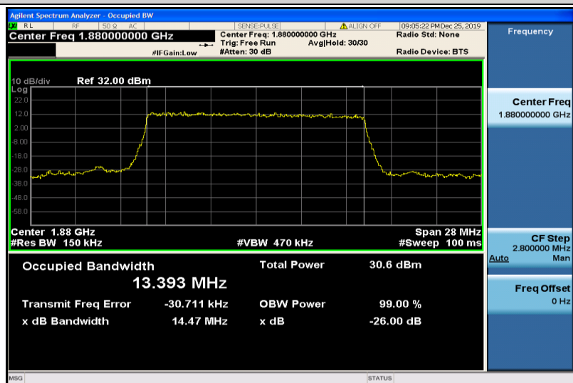
Band2-15MHz-QPSK-18900-75RB#0-13.393
