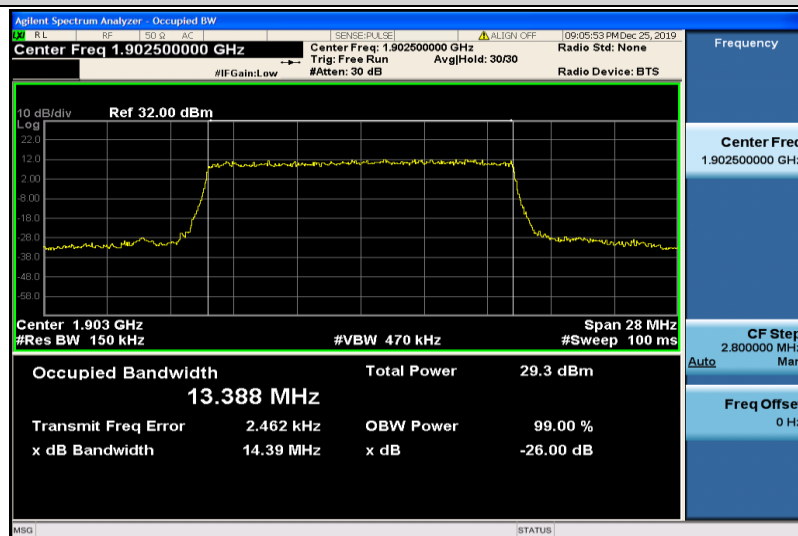
Band2-15MHz-16QAM-19125-75RB#0-13.388
