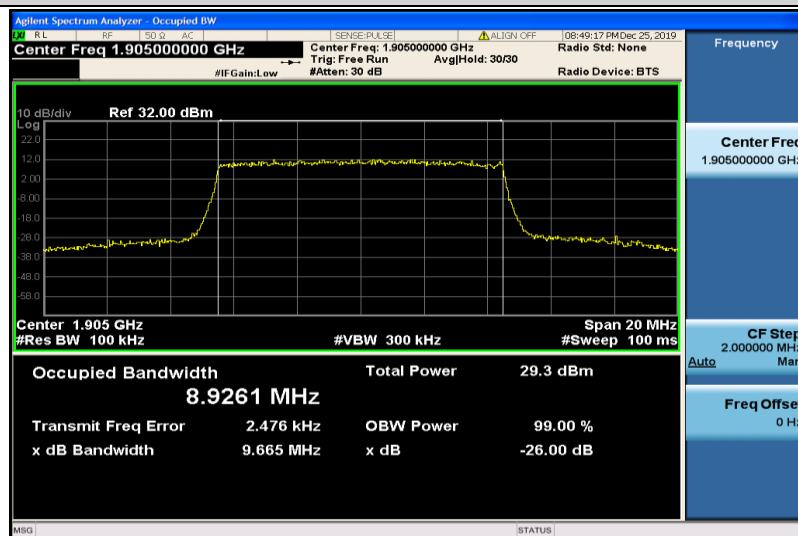
Band2-10MHz-16QAM-19150-50RB#0-8.9261
