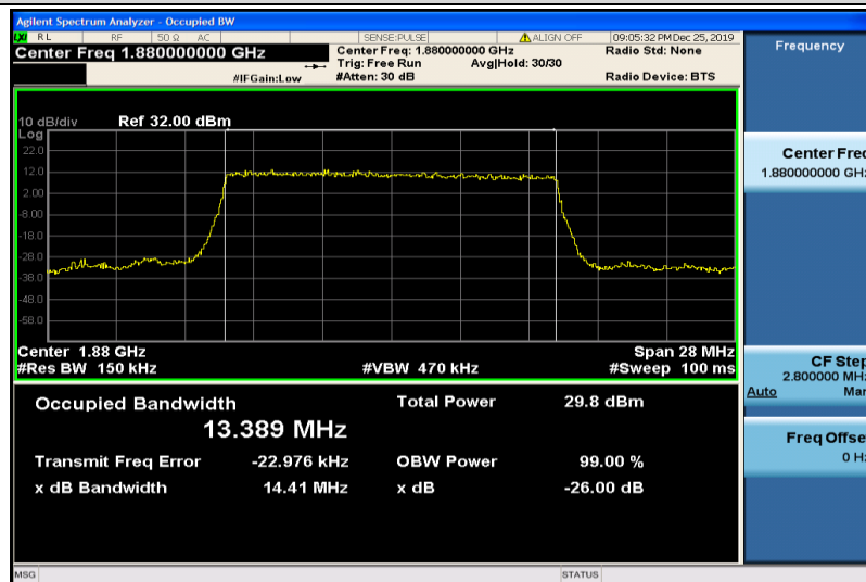
Band2-15MHz-16QAM-18900-75RB#0-13.389
