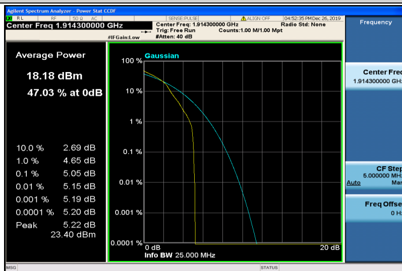
Band25-1.4MHz-16QAM-26683-1RB#0
