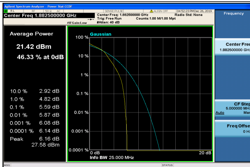
Band25-1.4MHz-16QAM-26365-6RB#0
