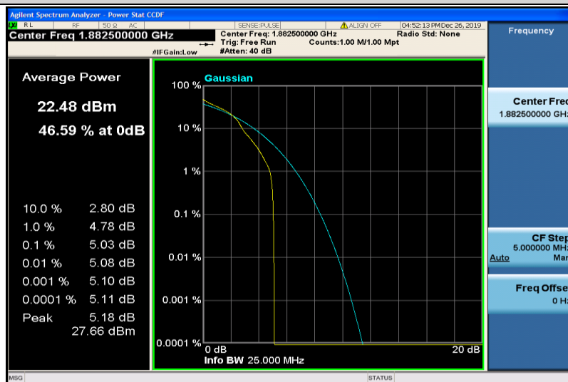
Band25-1.4MHz-16QAM-26365-1RB#0
