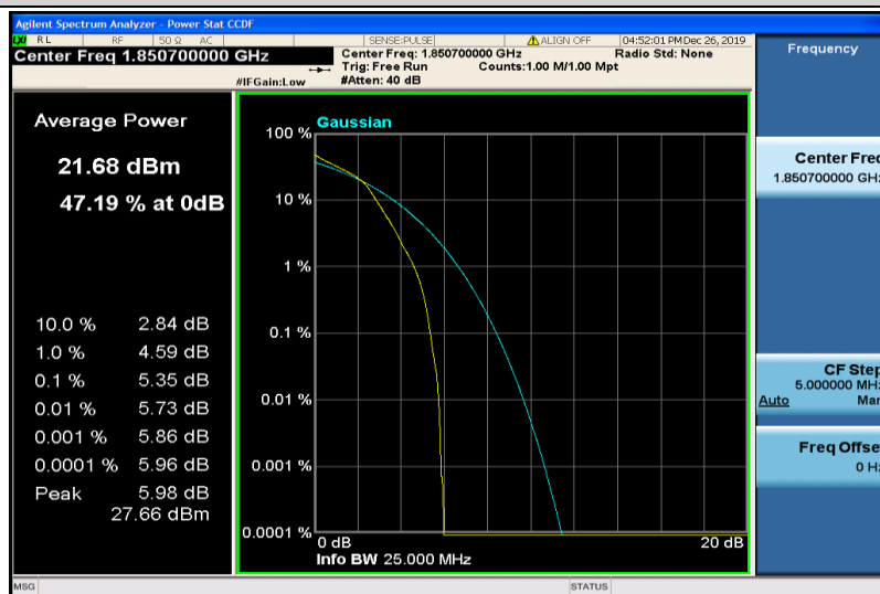
Band25-1.4MHz-16QAM-26047-6RB#0
