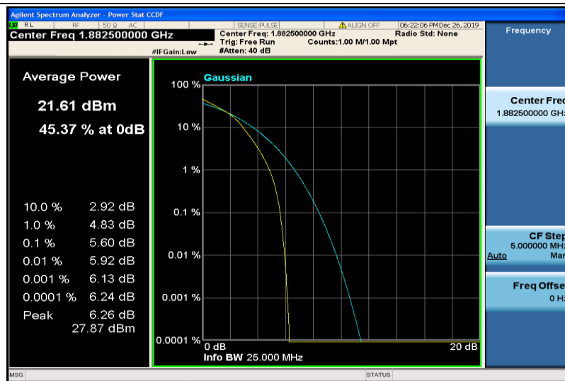
Band25-15MHz-16QAM-26365-75RB#0
