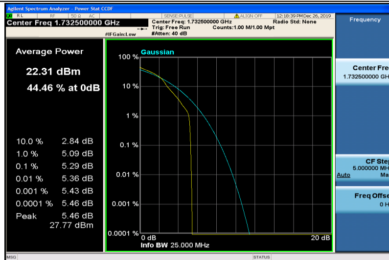
Band4-15MHz-16QAM-20175-1RB#0
