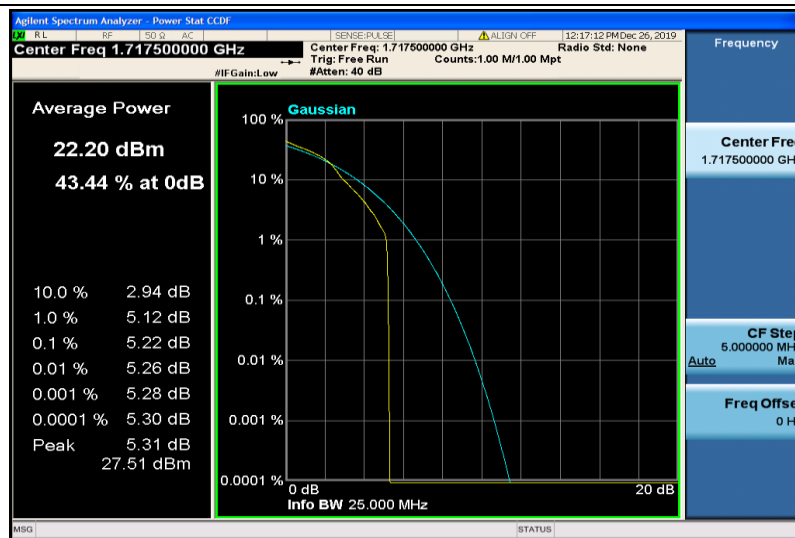
Band4-15MHz-16QAM-20025-1RB#0
