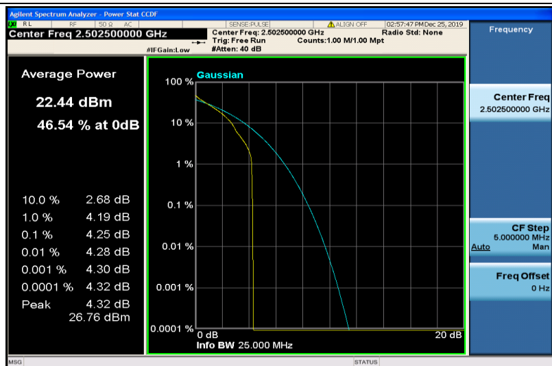
Band7-5MHz-QPSK-20775-1RB#0
