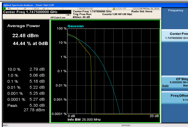
Band4-15MHz-16QAM-20325-1RB#0
