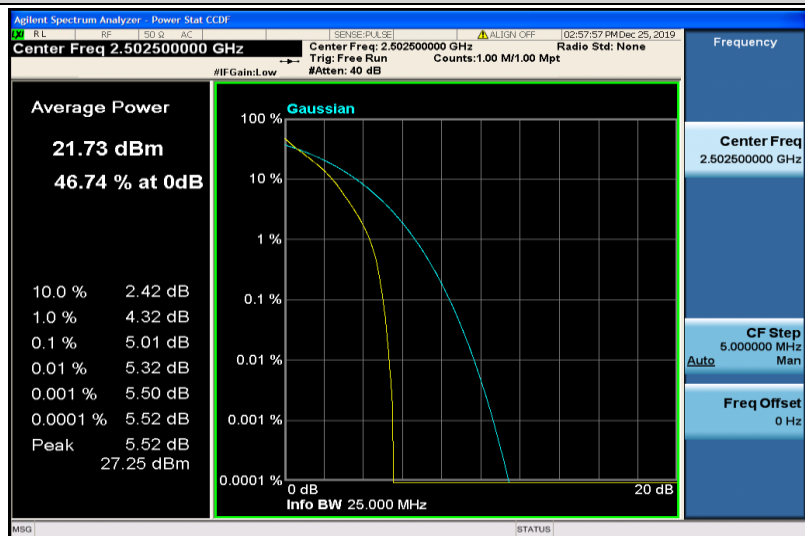
Band7-5MHz-QPSK-20775-25RB#0
