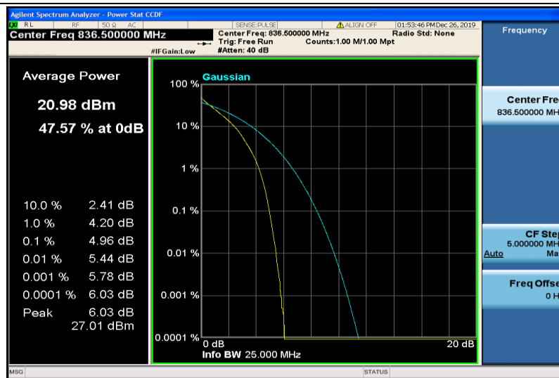
Band5-3MHz-QPSK-20525-15RB#0
