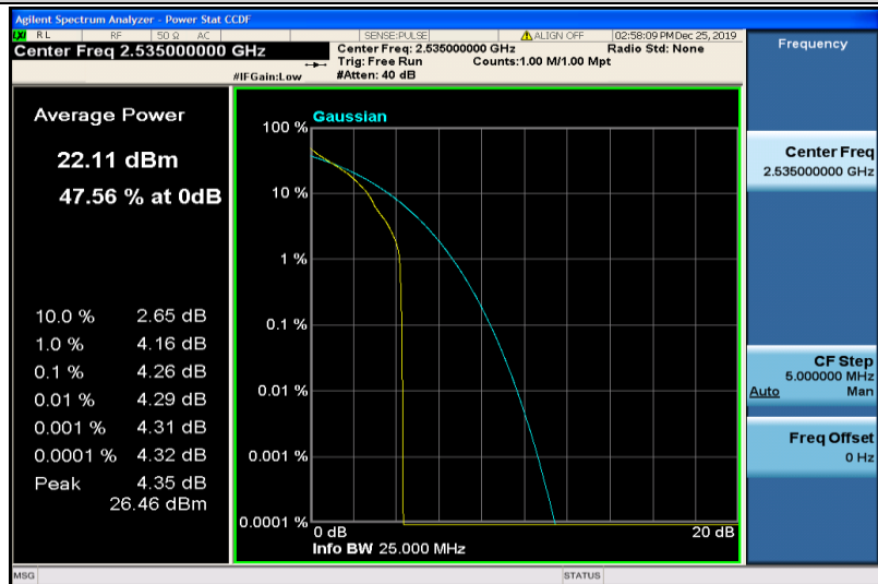
Band7-5MHz-QPSK-21100-1RB#0
