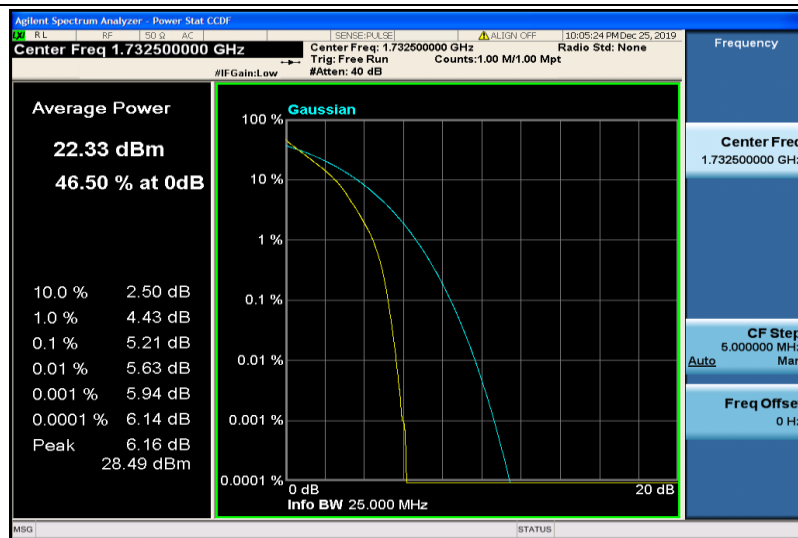
Band4-3MHz-QPSK-20175-15RB#0
