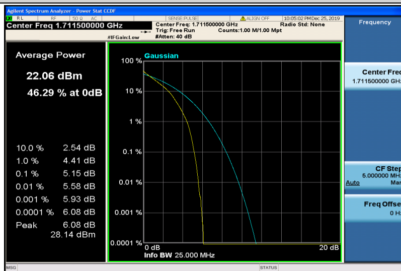
Band4-3MHz-QPSK-19965-15RB#0
