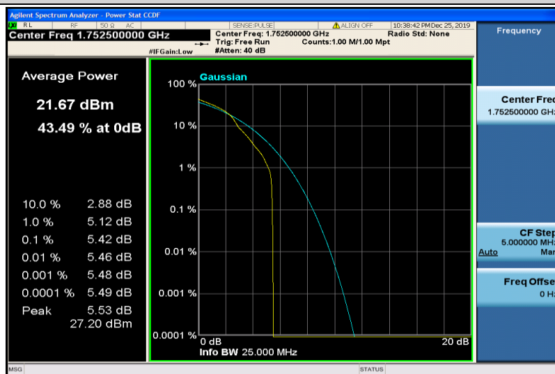
Band4-5MHz-16QAM-20375-1RB#0
