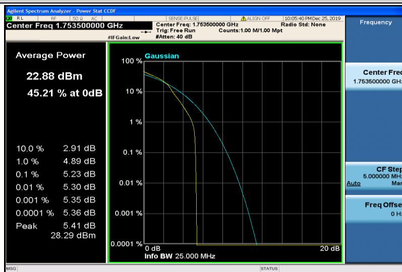
Band4-3MHz-16QAM-20385-1RB#0
