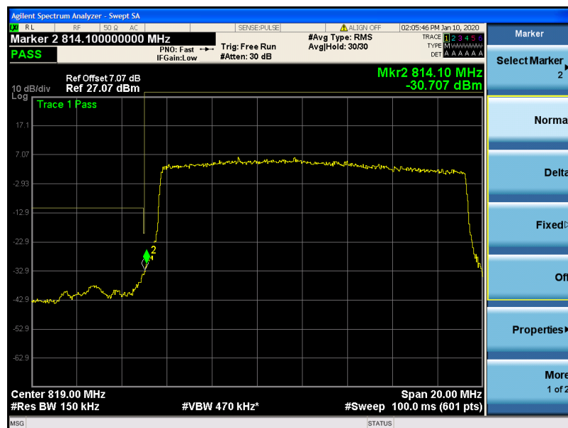
Band26-15MHz-QPSK-26765-75RB#0
