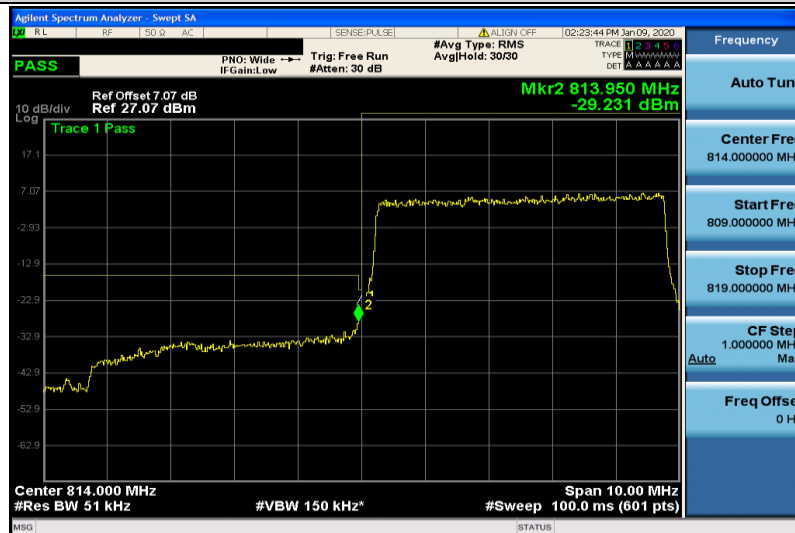
Band26-5MHz-QPSK-26715-25RB#0
