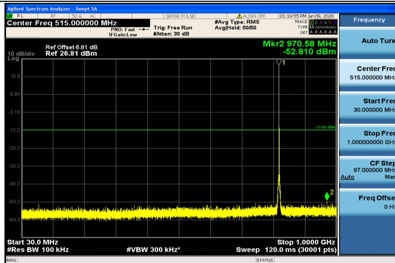
Band26-1.4MHz-16QAM-26783-1RB#0-30~1000MHz
