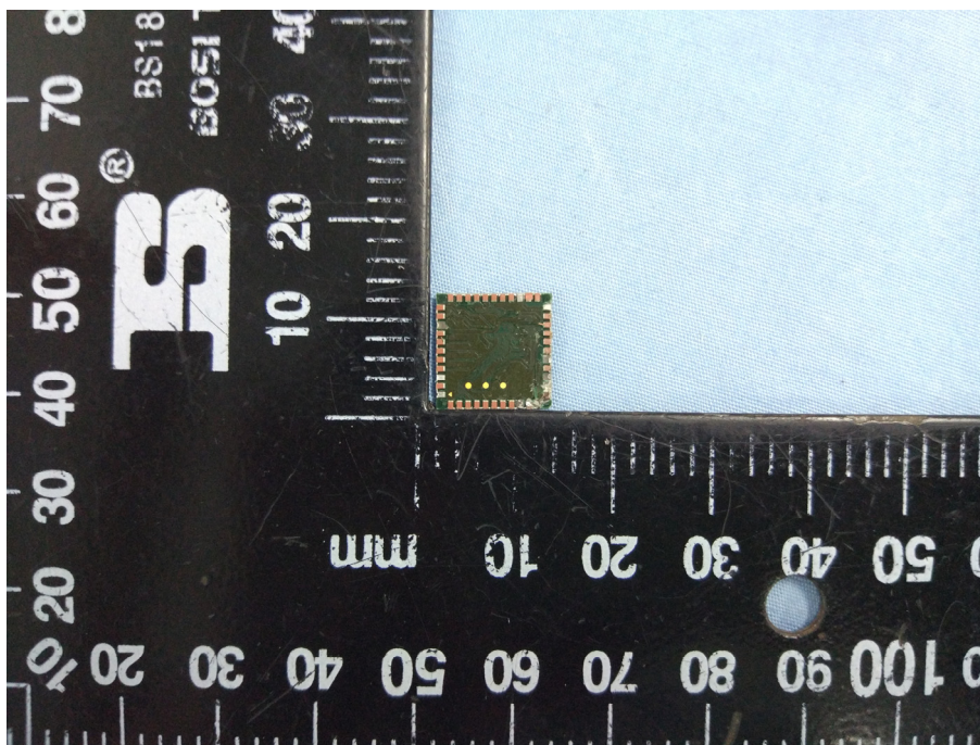
Solder Board-Component View 22(WIFI&BT)
