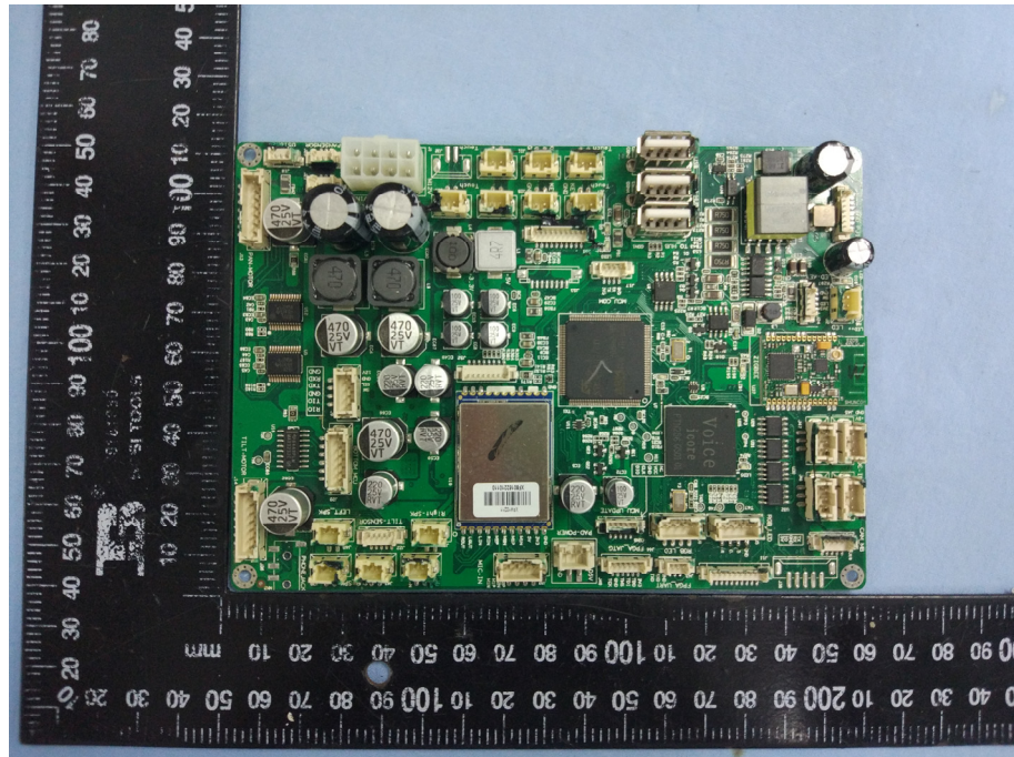
Solder Board-Component View 11 (MCU TOP)
