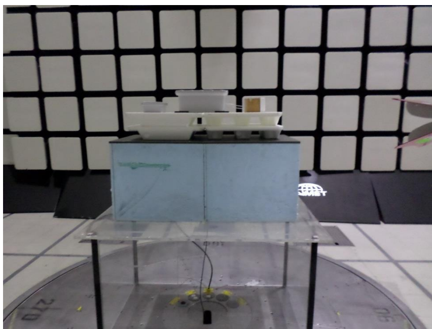
Photograph 2. Radiated Spurious Emissions, Test Setup (Above 1GHz) (A)
