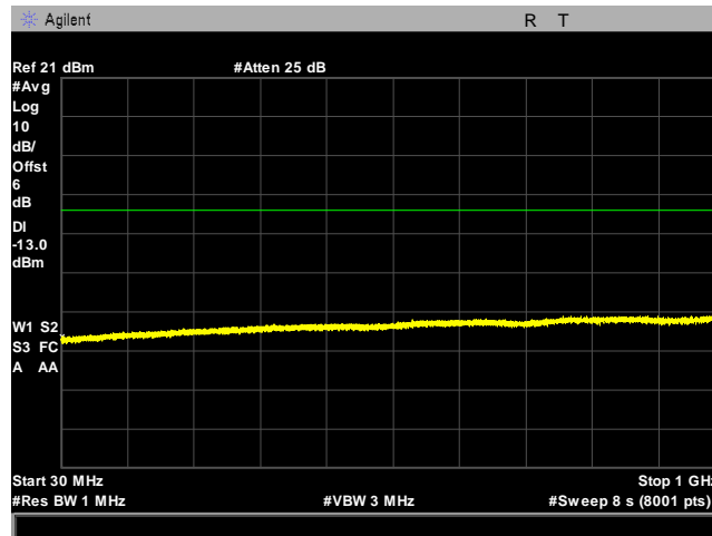
Plot 25. Spurious Emissions at Antenna Terminals, WCDMA Band IV, Mid Channel, 30MHz – 1 GHz
