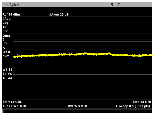
Plot 24. Spurious Emissions at Antenna Terminals, WCDMA Band IV, Low Channel, 14 GHz – 18 GHz
