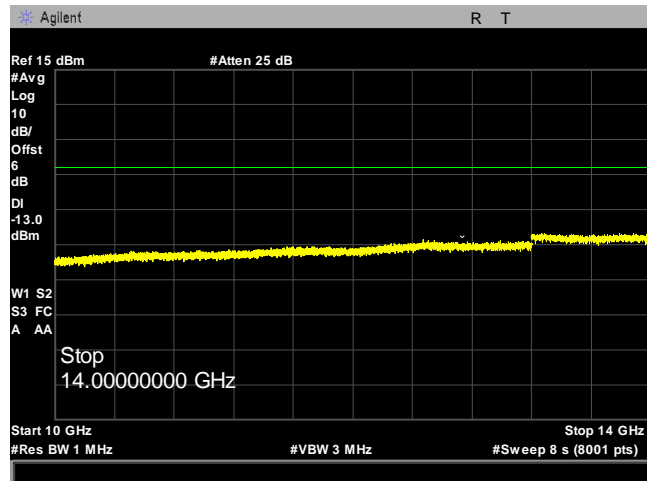
Plot 29. Spurious Emissions at Antenna Terminals, WCDMA Band IV, Mid Channel, 10 GHz - 14 GHz
