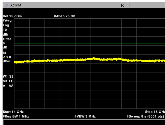
Plot 18. Spurious Emissions at Antenna Terminals, WCDMA Band IV, High Channel, 14 GHz - 18 GHz
