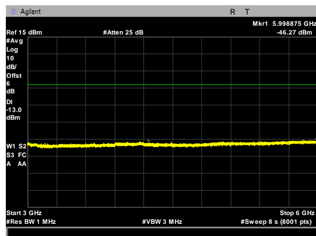
Plot 14. Spurious Emissions at Antenna Terminals, WCDMA Band IV, High Channel, 3 GHz - 6 GHz
