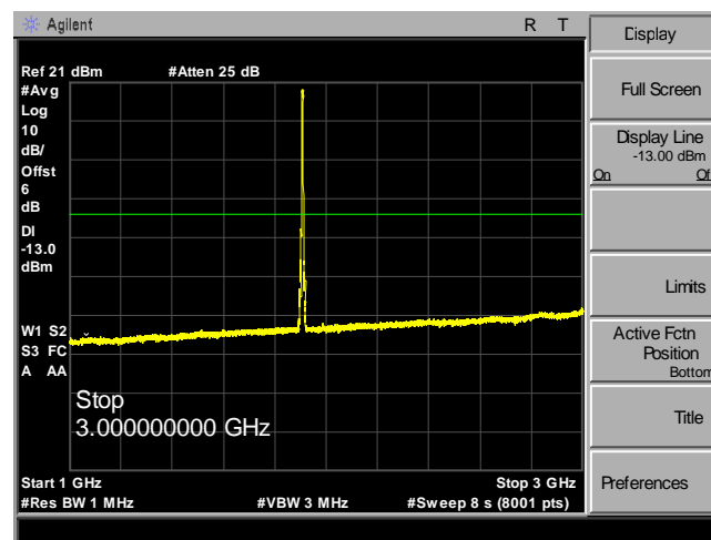
Plot 13. Spurious Emissions at Antenna Terminals, WCDMA Band IV, High Channel, 1 GHz to 3 GHz
