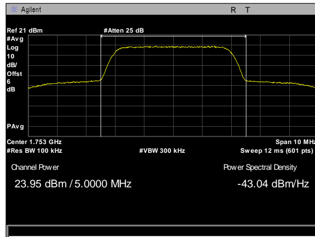
Plot 1. RF Power Output, WCDMA, Band IV Power, High Channel
