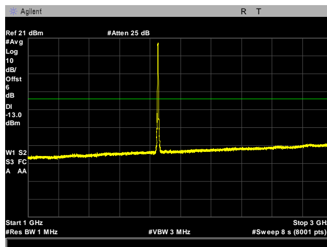
Plot 20. Spurious Emissions at Antenna Terminals, WCDMA Band IV, Low Channel, 1 GHz - 3 GHz
