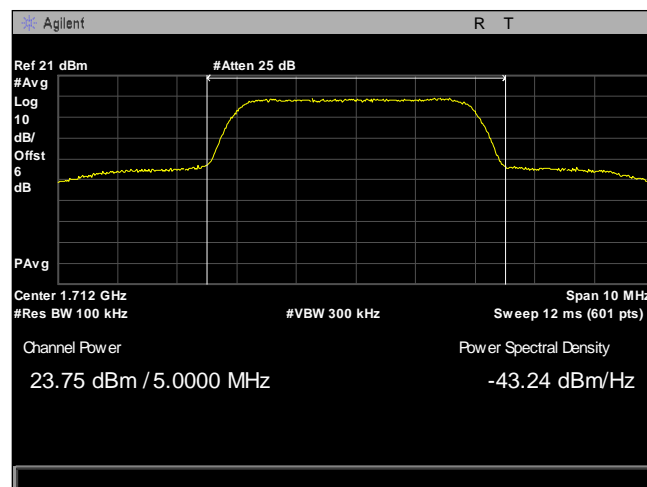
Plot 2. RF Power Output, WCDMA, Band IV Power, Low Channel
