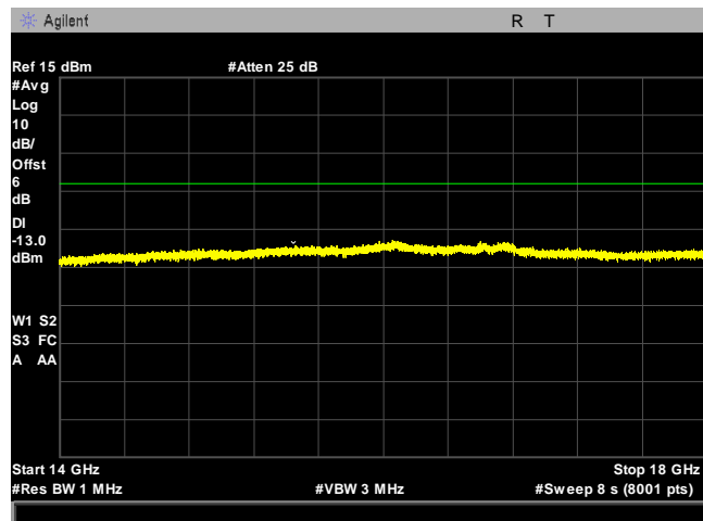
Plot 30. Spurious Emissions at Antenna Terminals, WCDMA Band IV, Mid Channel, 14 GHz - 18 GHz
