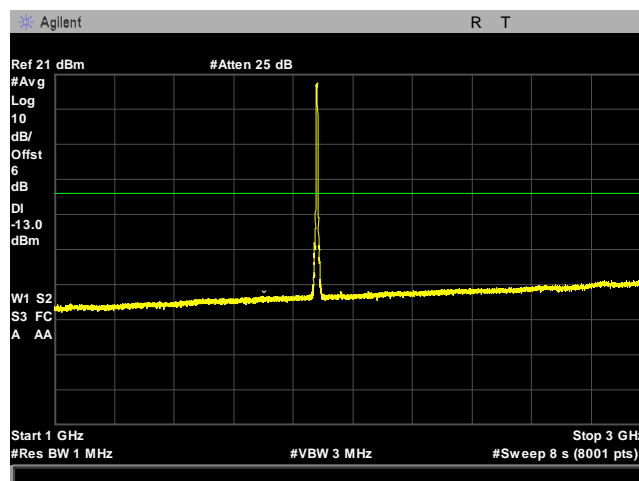
Plot 26. Spurious Emissions at Antenna Terminals, WCDMA Band IV, Mid Channel, 1 GHz - 3 GHz
