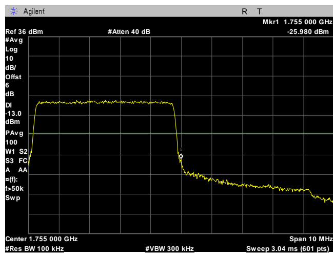
Plot 32. Spurious Emissions at Antenna Terminals, Right Band Edge
