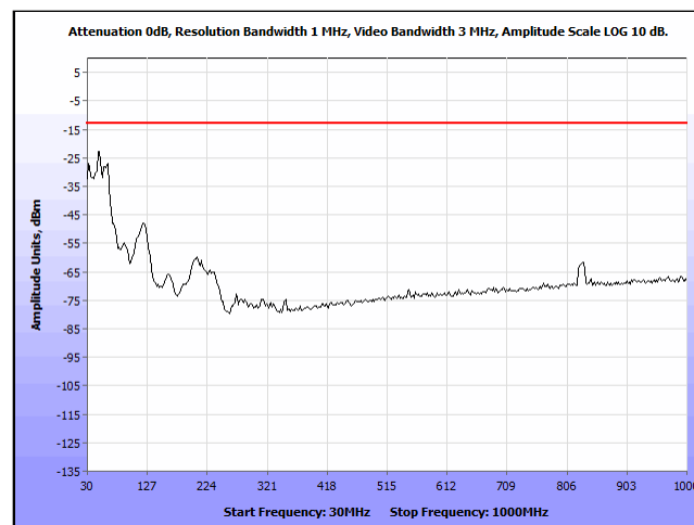
Plot 11. Radiated Spurious Emissions, 30MHz-1GHz
