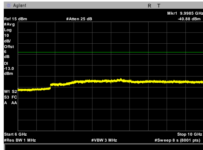
Plot 16. Spurious Emissions at Antenna Terminals, WCDMA Band IV, High Channel, 6 GHz - 10 GHz
