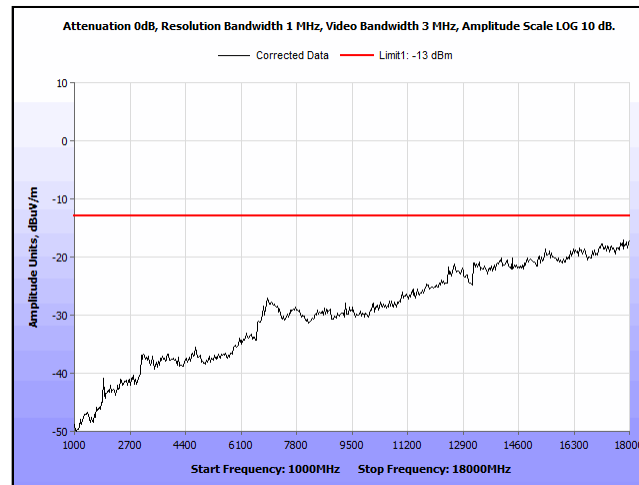
Plot 10. Radiated Spurious Emissions, 1GHz-18GHz
