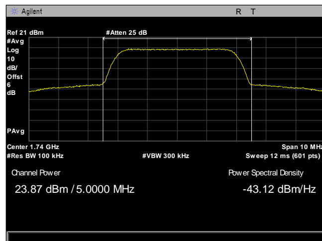
Plot 3. RF Power Output, WCDMA, Band IV Power, Mid Channel
