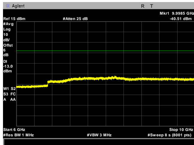
Plot 22. Spurious Emissions at Antenna Terminals, WCDMA Band IV, Low Channel, 6 GHz – 10 GHz
