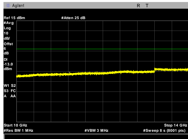
Plot 17. Spurious Emissions at Antenna Terminals, WCDMA Band IV, High Channel, 10 GHz - 14 GHz
