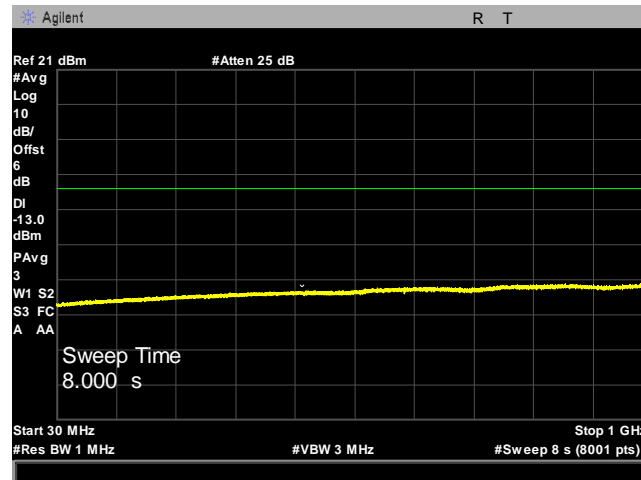
Plot 12. Spurious Emissions at Antenna Terminals, WCDMA Band IV, High Channel, 30 MHz - 1 GHz
