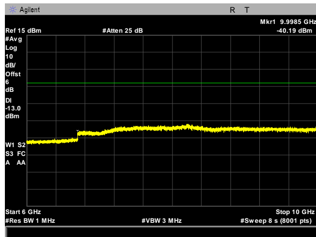
Plot 28. Spurious Emissions at Antenna Terminals, WCDMA Band IV, Mid Channel, 6 GHz - 10 GHz
