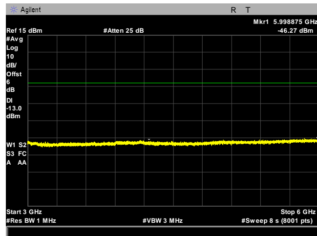
Plot 15. Spurious Emissions at Antenna Terminals, WCDMA Band IV, High Channel, 3 GHz to 6 GHz
