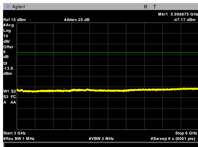
Plot 27. Spurious Emissions at Antenna Terminals, WCDMA Band IV, Mid Channel, 3 GHz - 6 GHz
