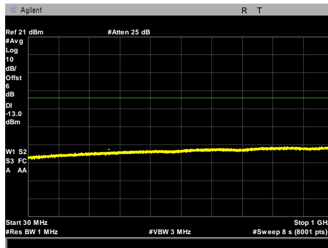
Plot 19. Spurious Emissions at Antenna Terminals, WCDMA Band IV, Low Channel, 30 MHz – 1 GHz
