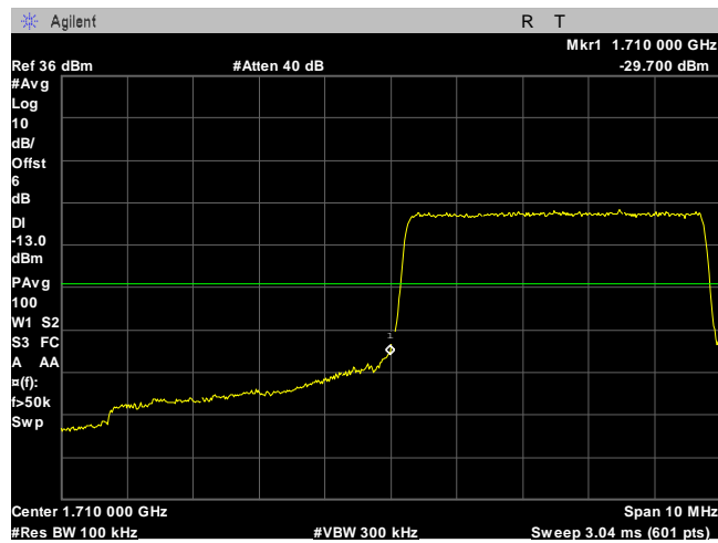
Plot 31. Spurious Emissions at Antenna Terminals, Left Band Edge
