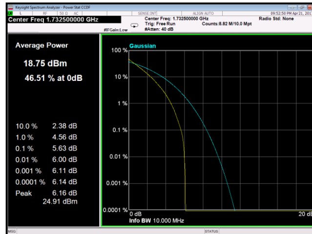
Plot 8. Peak to Average Ratio, WCDMA IV Mid Channel
