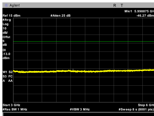
Plot 21. Spurious Emissions at Antenna Terminals, WCDMA Band IV, Low Channel, 3 GHz – 6 GHz
