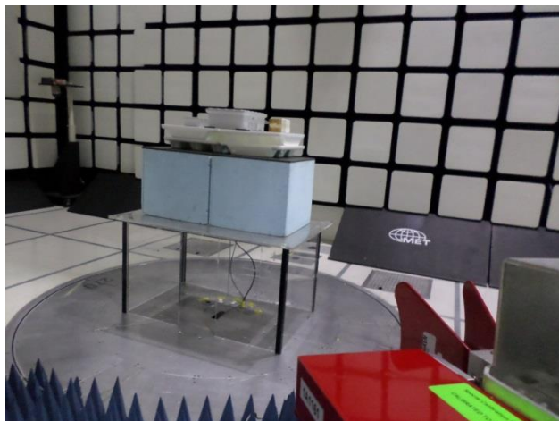
Photograph 9. Radiated setup, 18-40GHz antenna view
