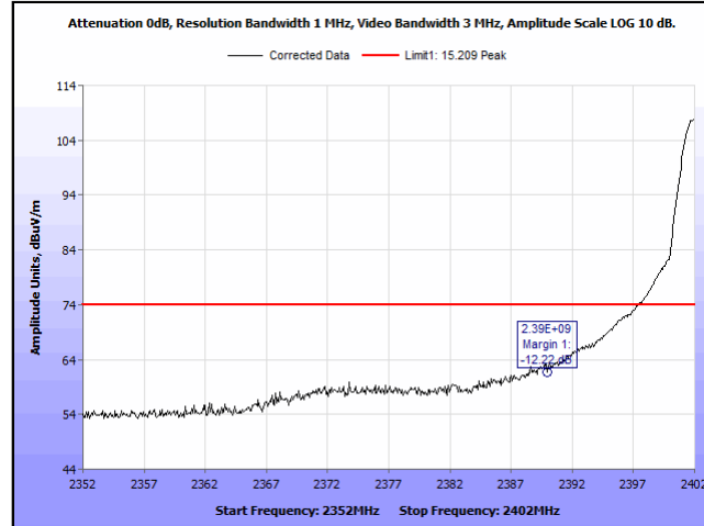
Plot 28. Radiated Restricted Band Edge, BT LE, 2402 MHz, Peak
