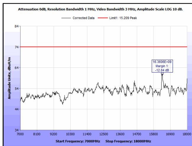
Plot 22. Spurious Radiated Emissions, BT LE - 2402 - 7-18GHz – Peak
