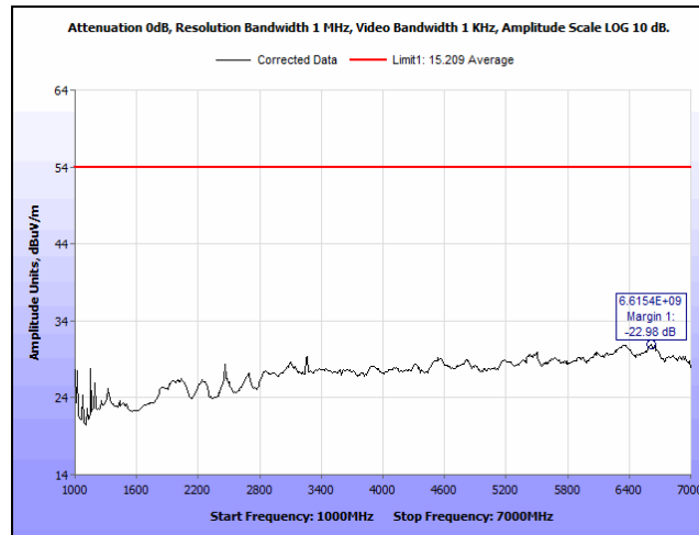
Plot 56. Radiated Spurious Emissions, 802.11g 2437MHz 1-7GHz Avg
