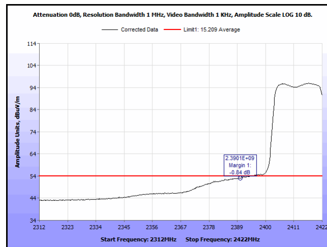
Plot 108. Radiated Restricted Band Edge, 802.11n HT40, 2422 MHz, Pwr 10, Average
