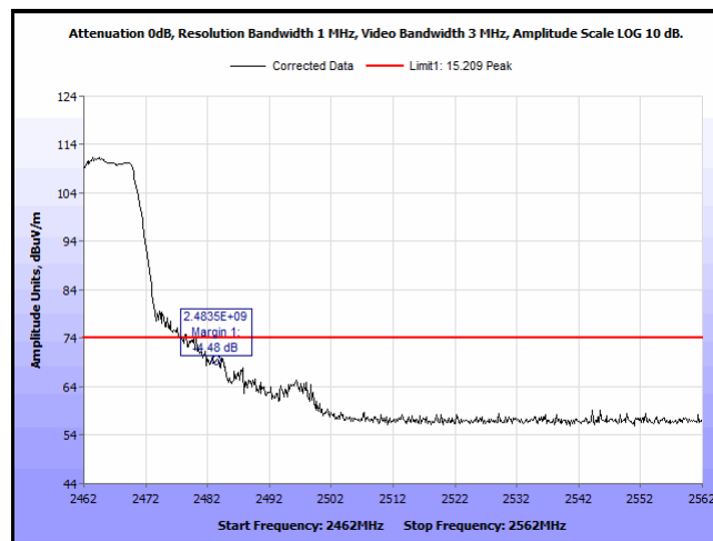
Plot 103. Radiated Restricted Band Edge, 802.11g, 2462 MHz, 12 Pwr, Peak
