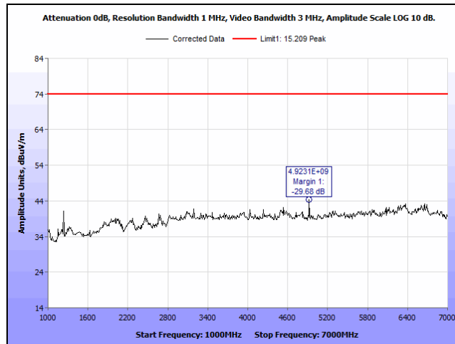
Plot 53. Radiated Spurious Emissions, 802.11b 2462MHz 1-7GHz Peak
