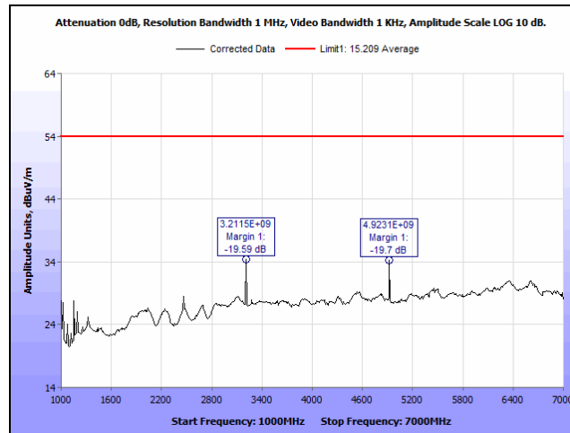
Plot 60. Radiated Spurious Emissions, 802.11n HT20 2412MHz 1-7GHz Avg
