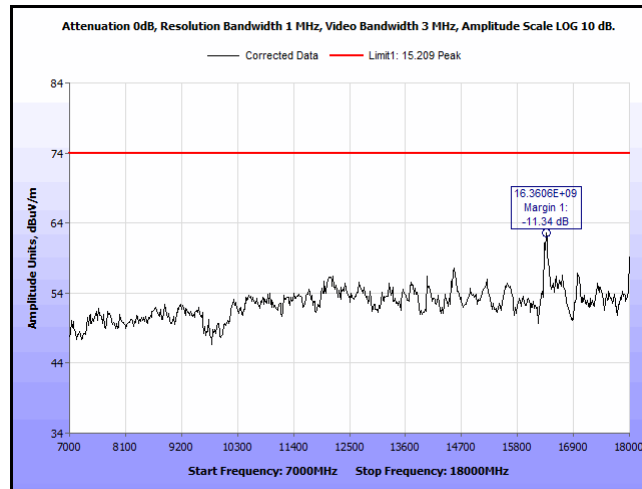
Plot 89. Radiated Spurious Emissions, 802.11n HT20 2462 7-18GHz Peak
