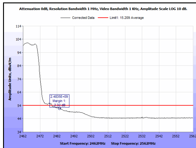
Plot 102. Radiated Restricted Band Edge, 802.11g, 2462 MHz, 12 Pwr, Average
