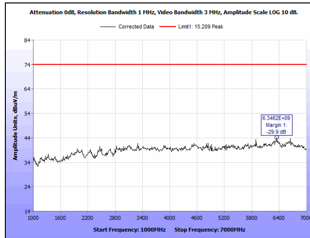
Plot 59. Radiated Spurious Emissions, 802.11g 2462MHz 1-7GHz Peak
