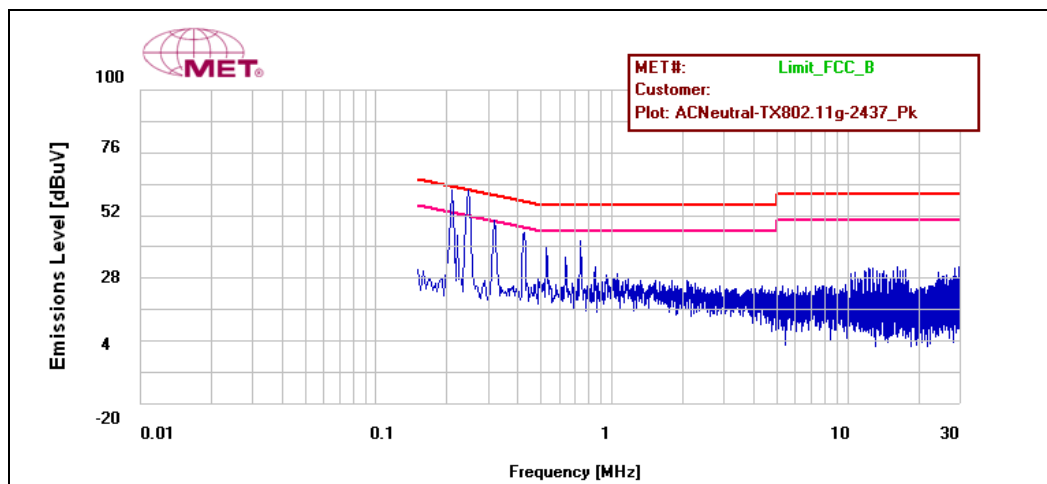
Plot 8. Conducted Emissions, 15.207(a), 2.4 GHz WiFi, 802.11g, Neutral Line
