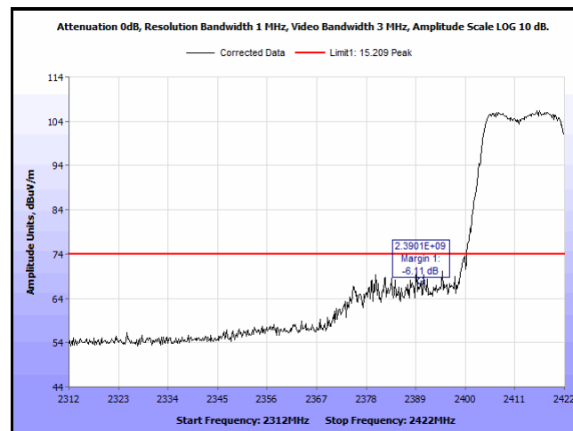
Plot 109. Radiated Restricted Band Edge, 802.11n HT40, 2422 MHz, Pwr 10, Peak
