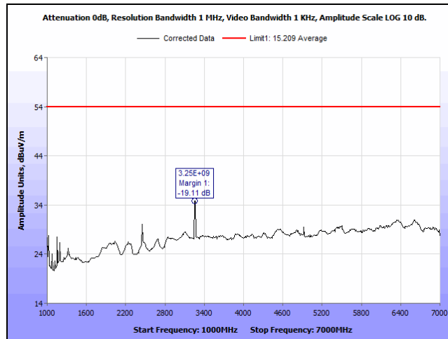
Plot 62. Radiated Spurious Emissions, 802.11n HT20 2437MHz 1-7GHz Avg
