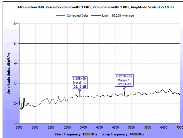
Plot 50. Radiated Spurious Emissions, 802.11b 2437MHz 1-7GHz Avg
