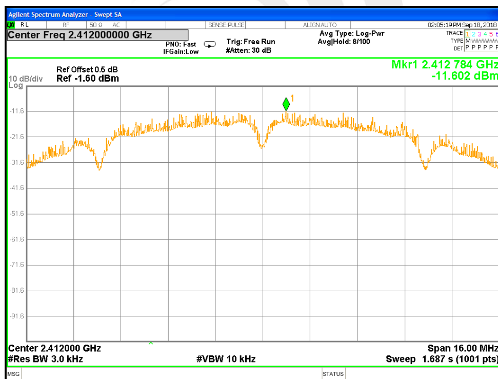
TX CH01
