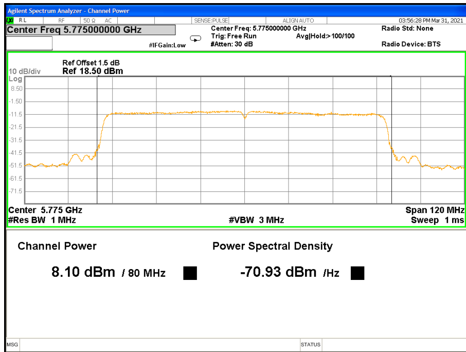
5775MHz_AV_Ant B
