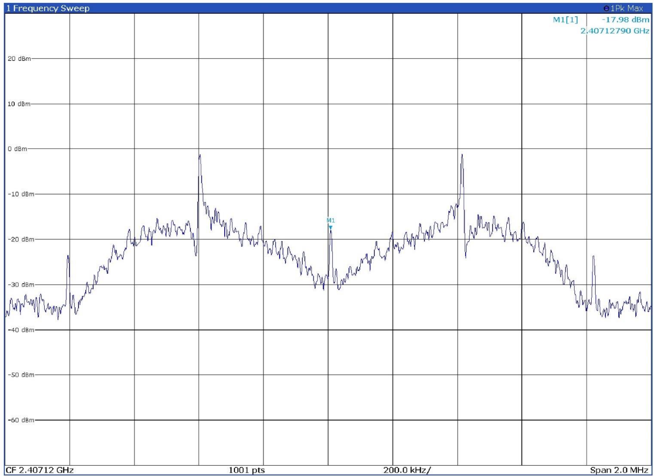
Figure 8.6-10: PSD on low channel – Antenna port 4
