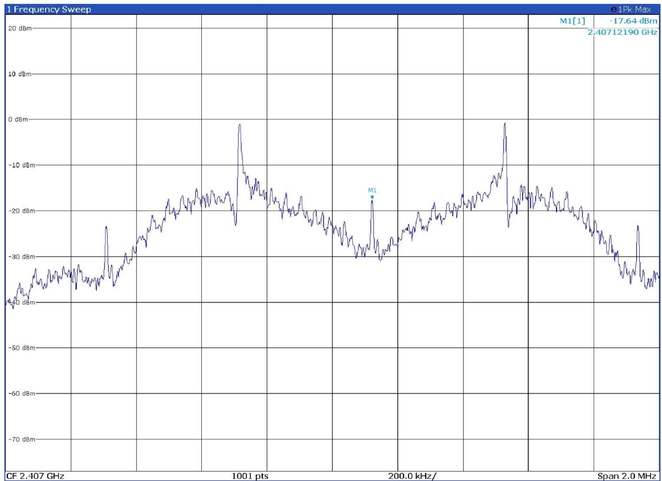
Figure 8.6-1: PSD on low channel – Antenna port 1
