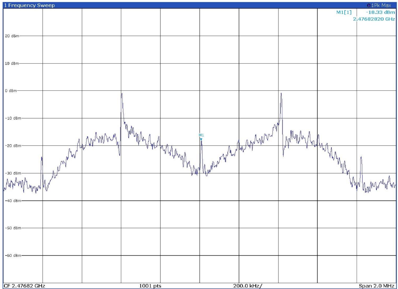
Figure 8.6-3: PSD on high channel – Antenna port 1
