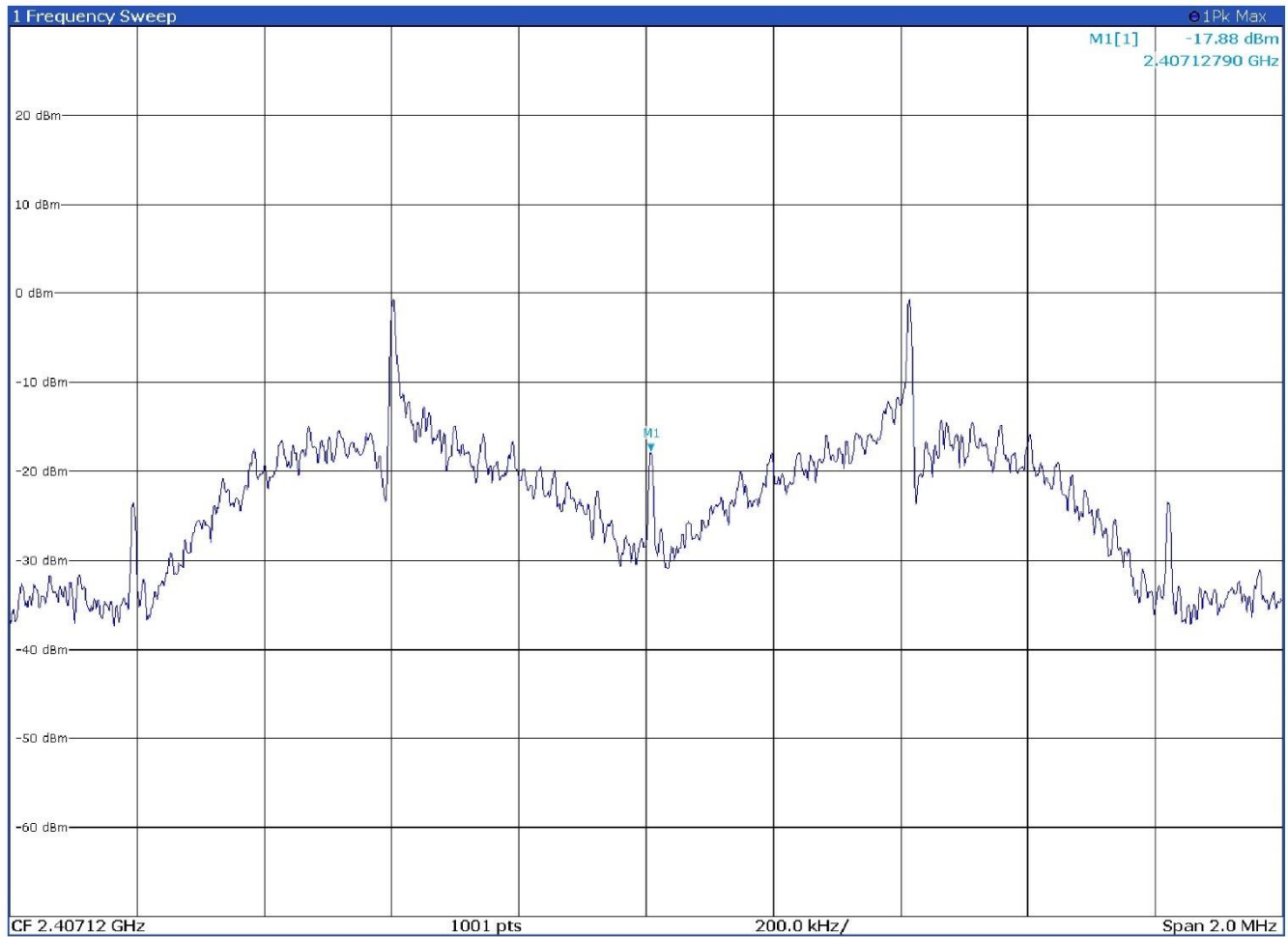
Figure 8.6-4: PSD on low channel – Antenna port 2
