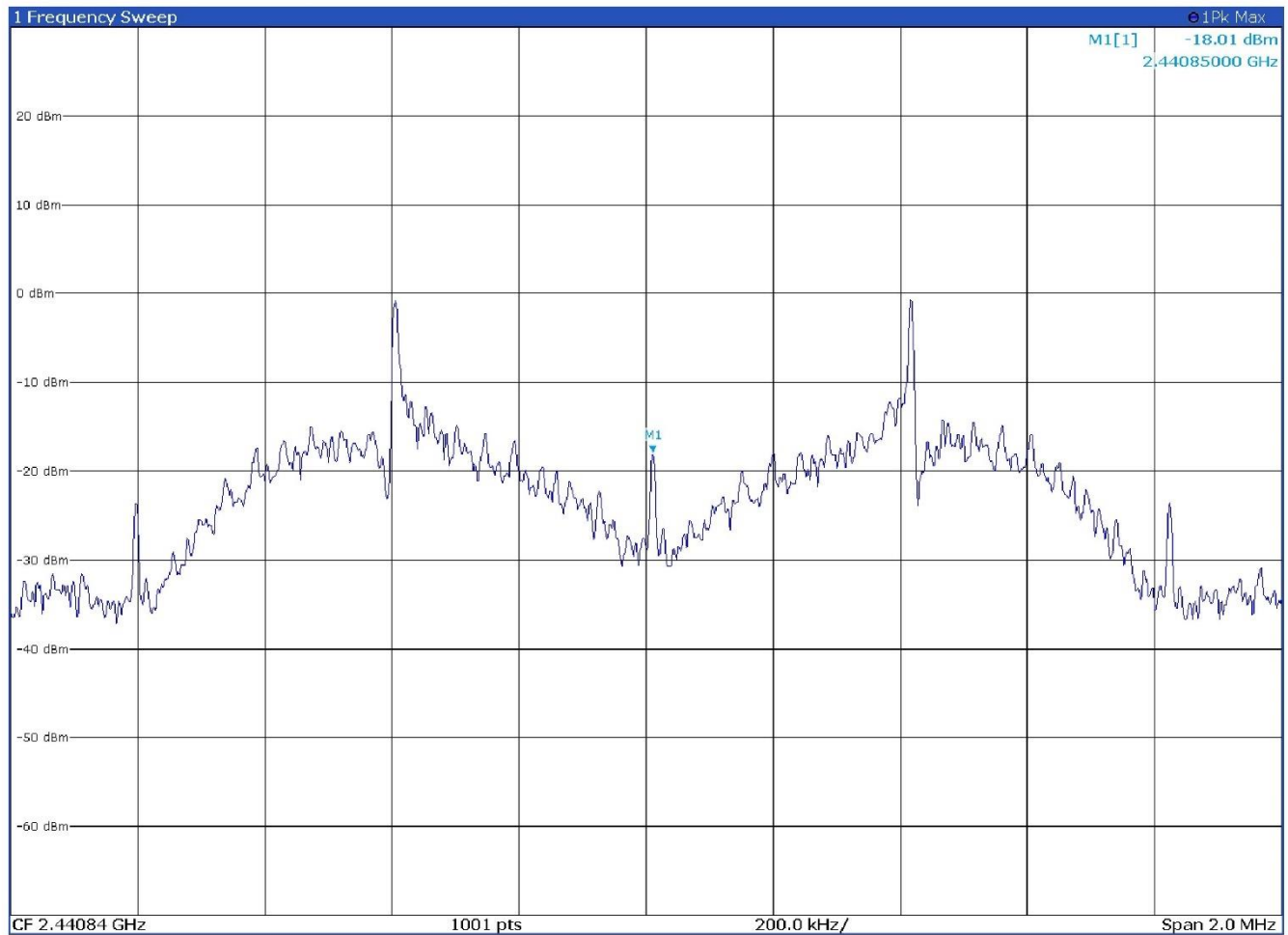
Figure 8.6-2: PSD on mid channel – Antenna port 1
