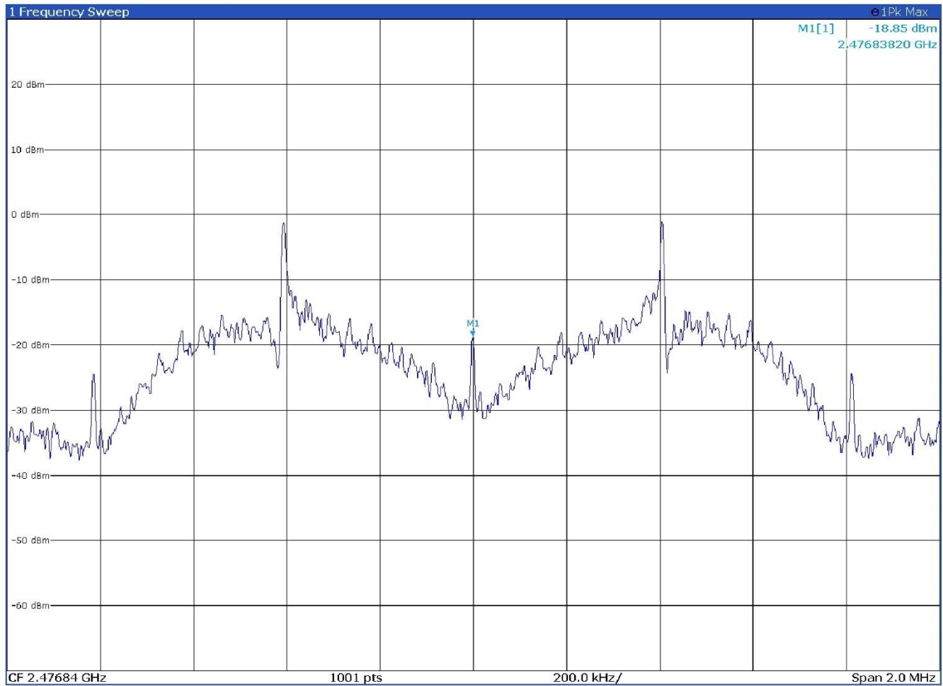
Figure 8.6-12: PSD on high channel – Antenna port 4
