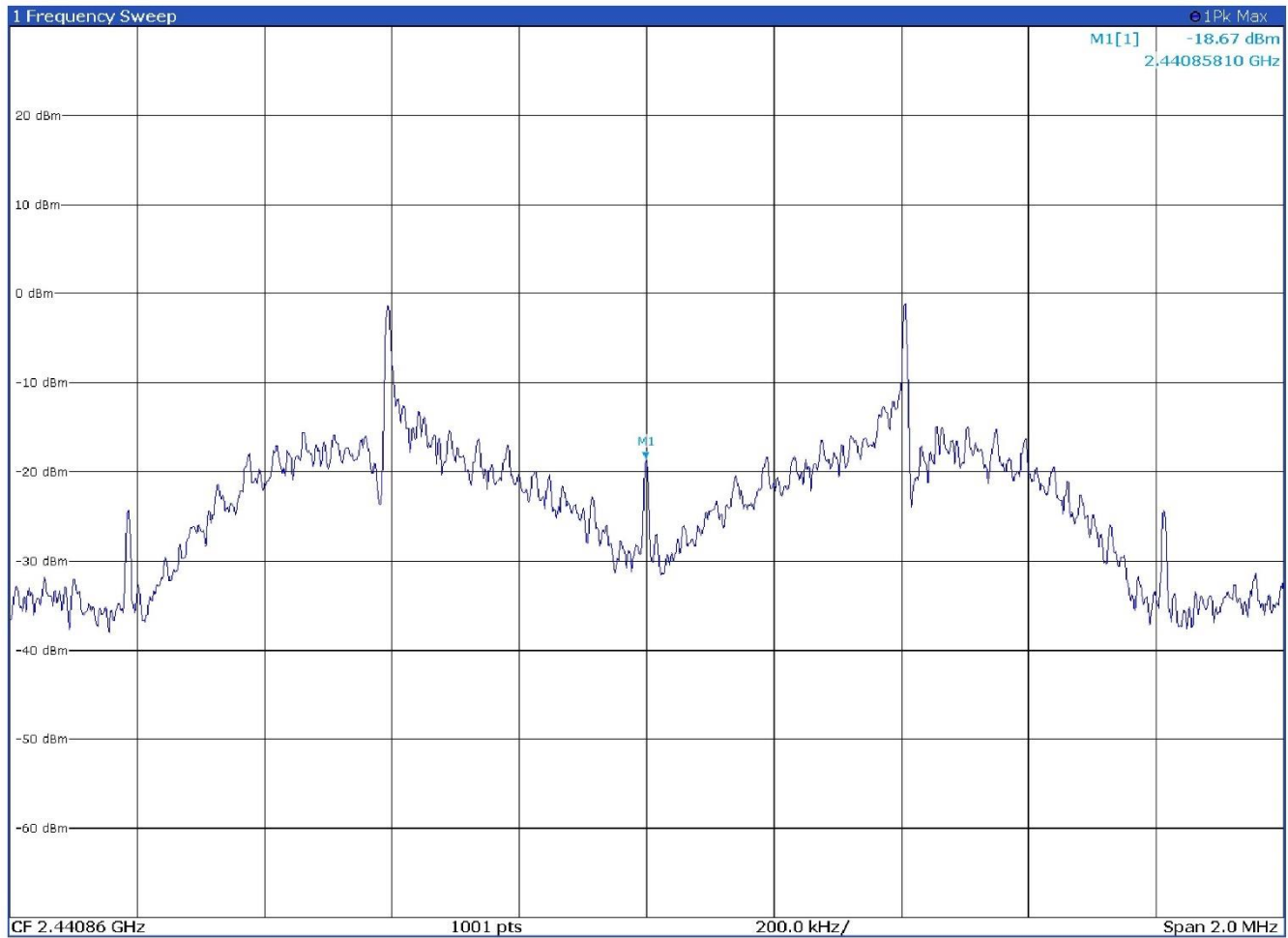
Figure 8.6-11: PSD on mid channel – Antenna port 4
