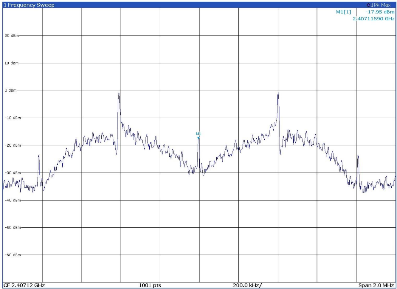
Figure 8.6-7: PSD on low channel – Antenna port 3
