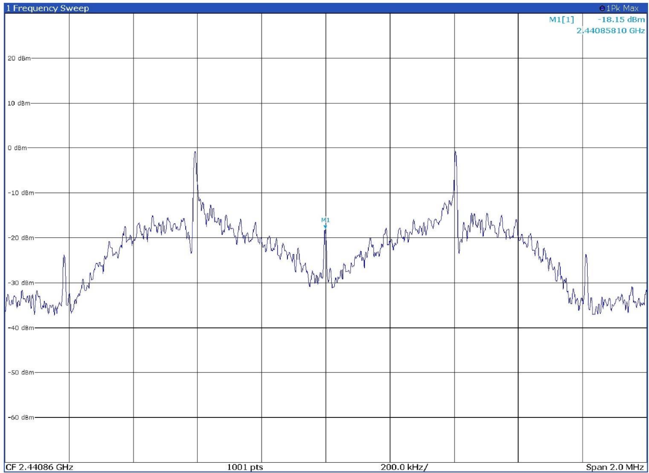
Figure 8.6-5: PSD on mid channel – Antenna port 2
