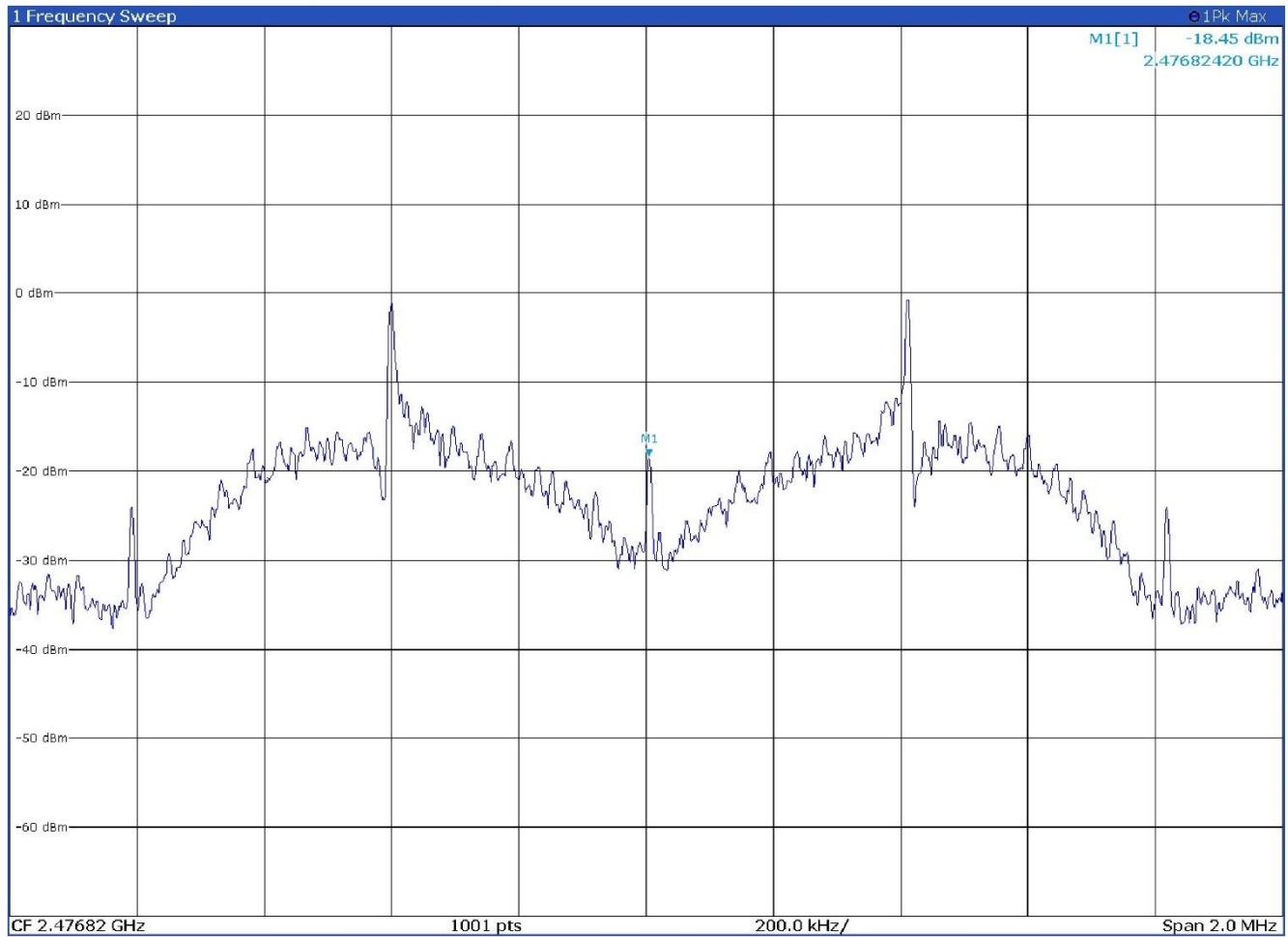
Figure 8.6-9: PSD on high channel – Antenna port 3
