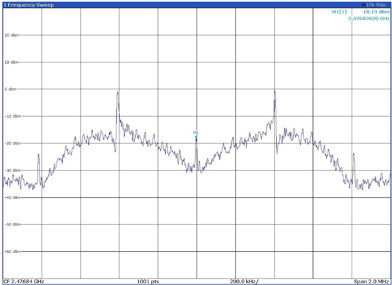
Figure 8.6-6: PSD on high channel – Antenna port 2
