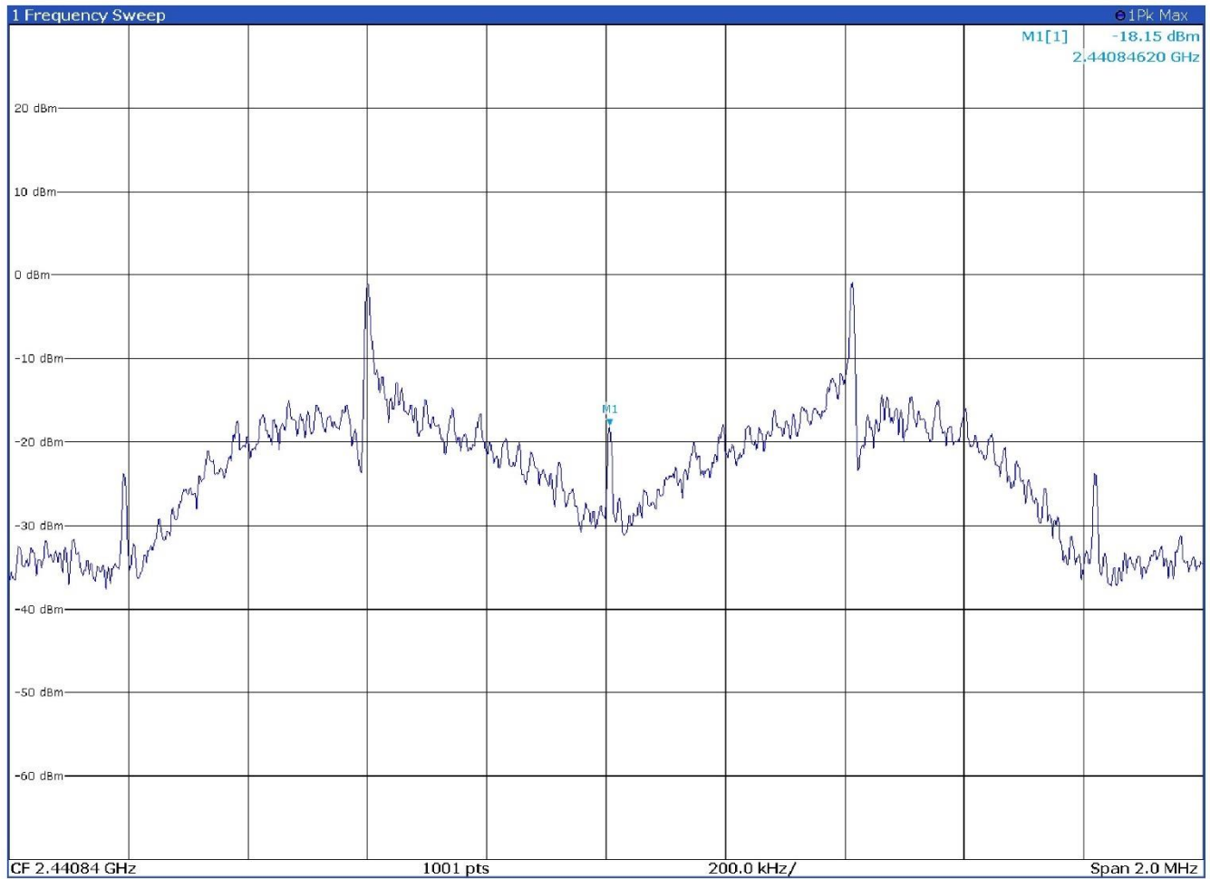
Figure 8.6-8: PSD on mid channel – Antenna port 3
