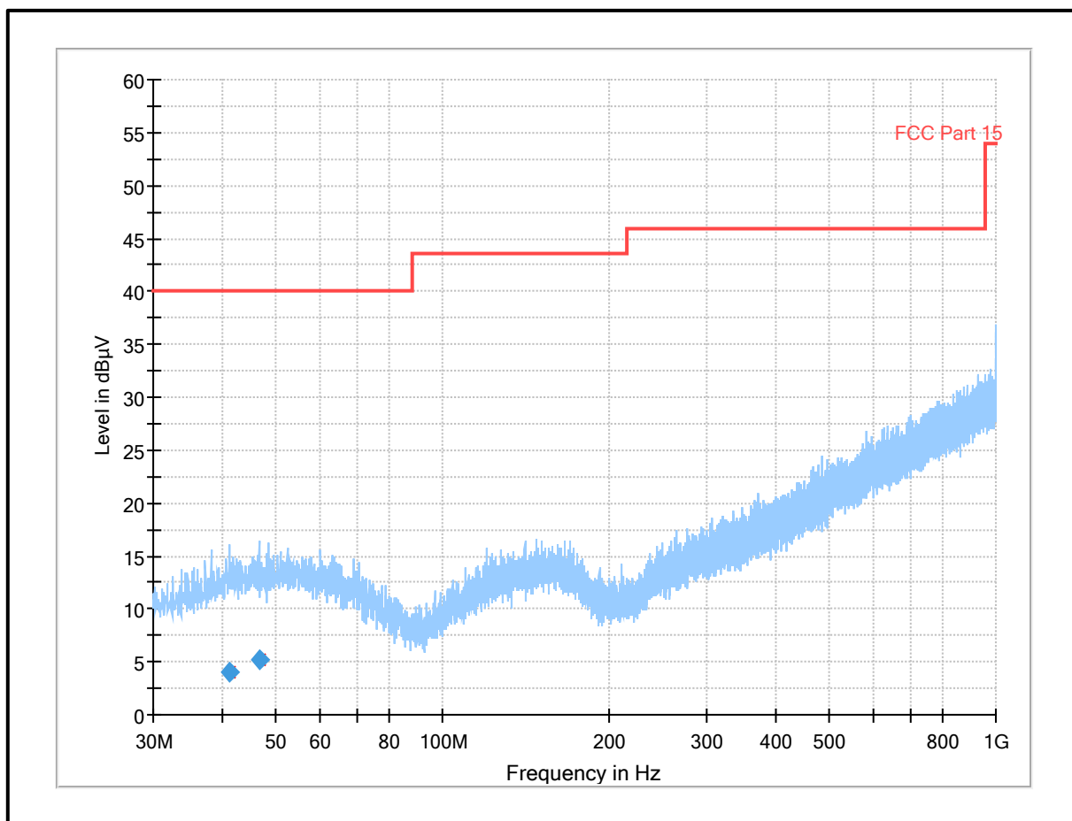
Plot: 30 MHz-1 GHz: Bluetooth Low Energy / Middle Channel
