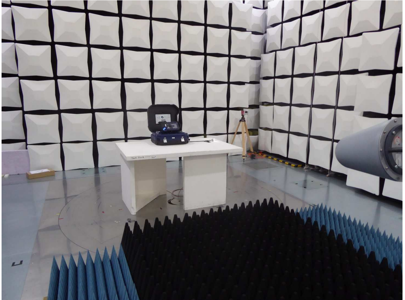
Test setup fully anechoic chamber (1 - 13 GHz)
