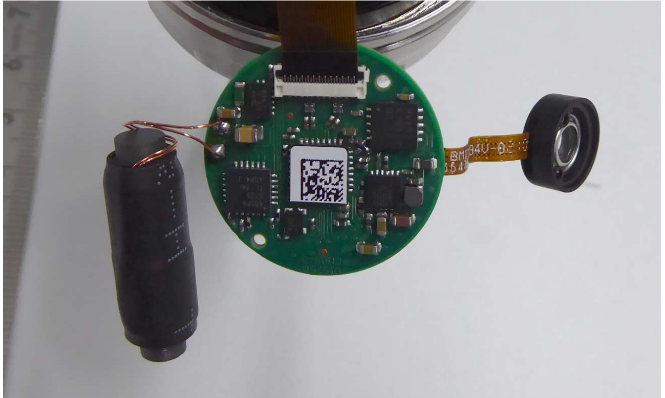
Wöhler VIS 750 - camera head 2
