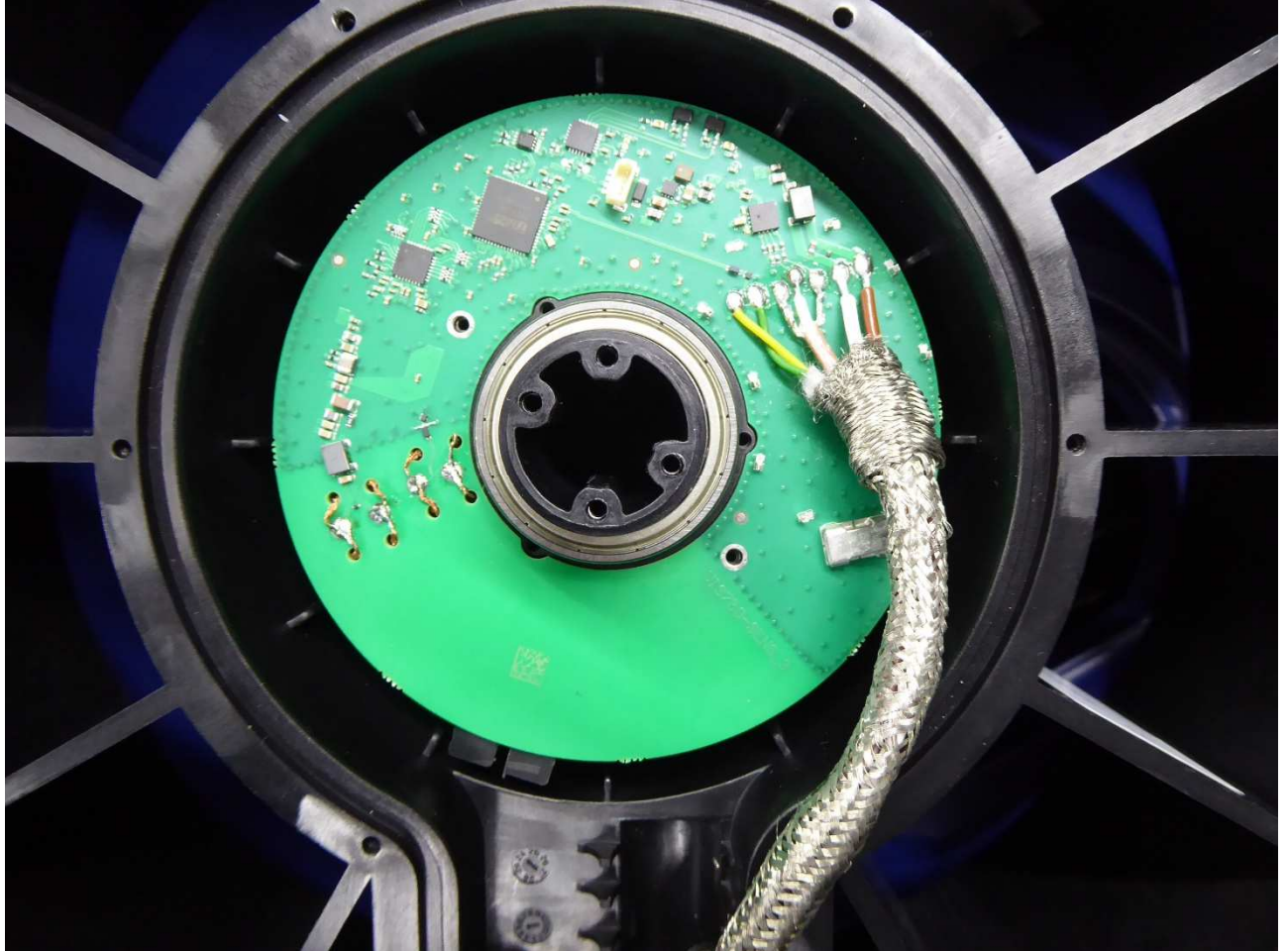
Wöhler VIS 750 - PCB
