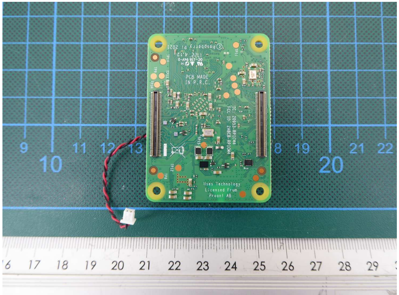
Wöhler VIS 750 – VIS 7 HD (monitor unit): Raspberry Pi PCB bottom view
