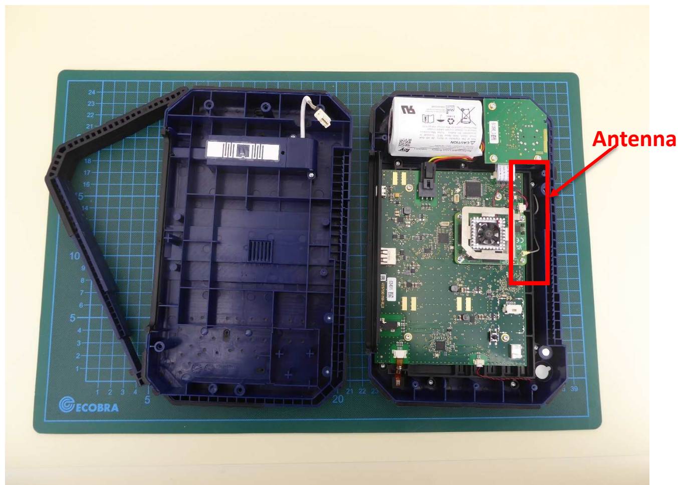
Wöhler VIS 750 – VIS 7 HD (monitor unit) disassembled - 2
