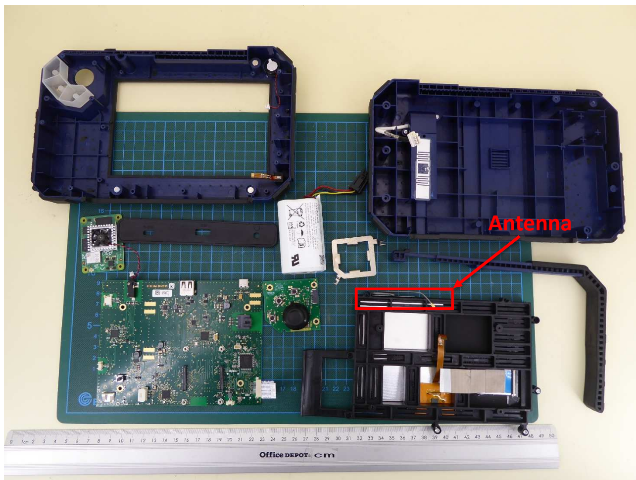
Wöhler VIS 700 – VIS 7 HD (monitor unit) disassembled - 1
