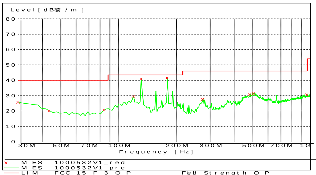
30MHz~1GHz, Vertical
