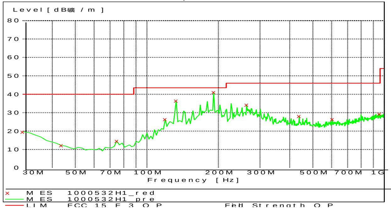
30MHz~1GHz, Horizontal
