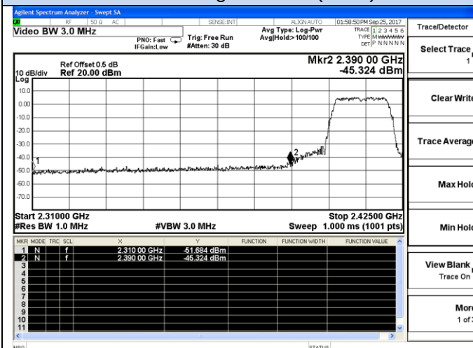
802.11g-Low channel(Peak)
