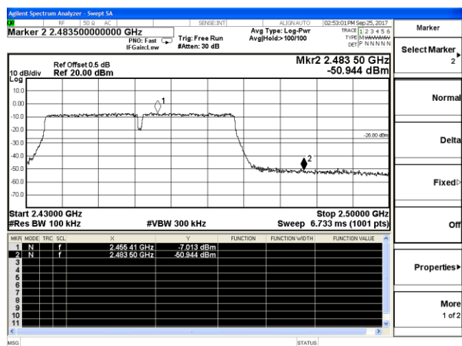
802.11n-HT40-High channel
