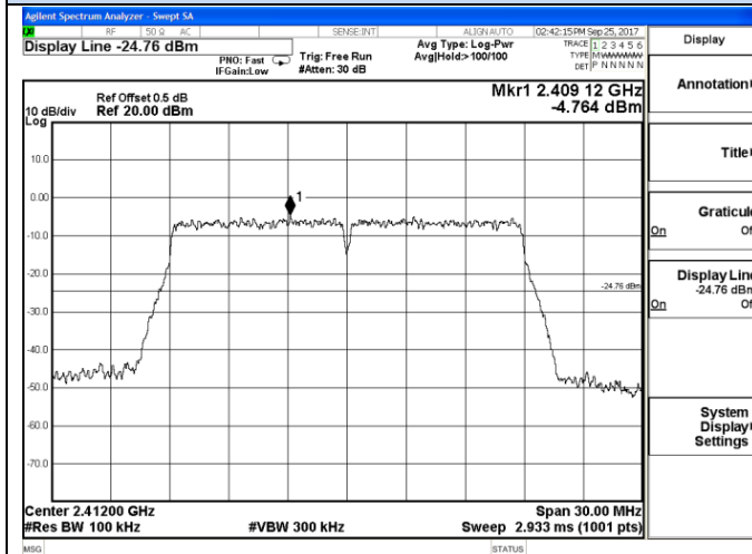
IEEE 802.11n HT20-Channel 1 / 2412 MHz
