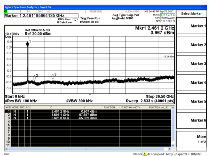
802.11b-High channel
