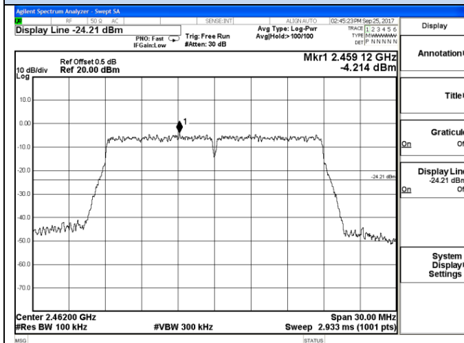
IEEE 802.11n HT20-Channel 11 / 2462 MHz
