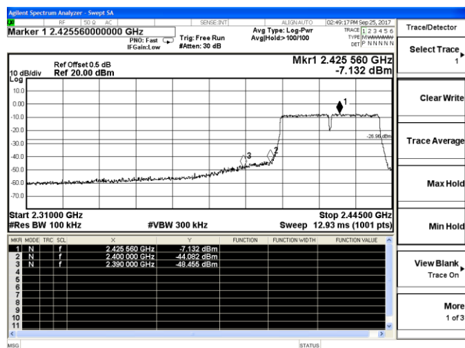
802.11n-HT40-Low channel
