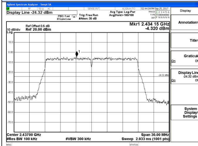
IEEE 802.11n HT20-Channel 6 / 2437 MHz
