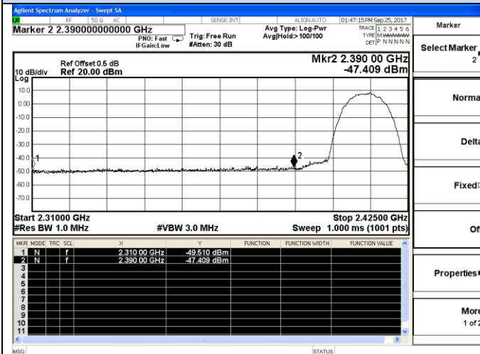
802.11b-Low channel(Peak)
