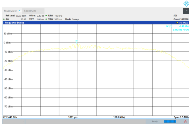
\pi/4 -DQPSK on Channel 39
