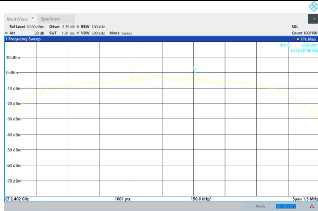
\pi/4 -DQPSK on Channel 00
