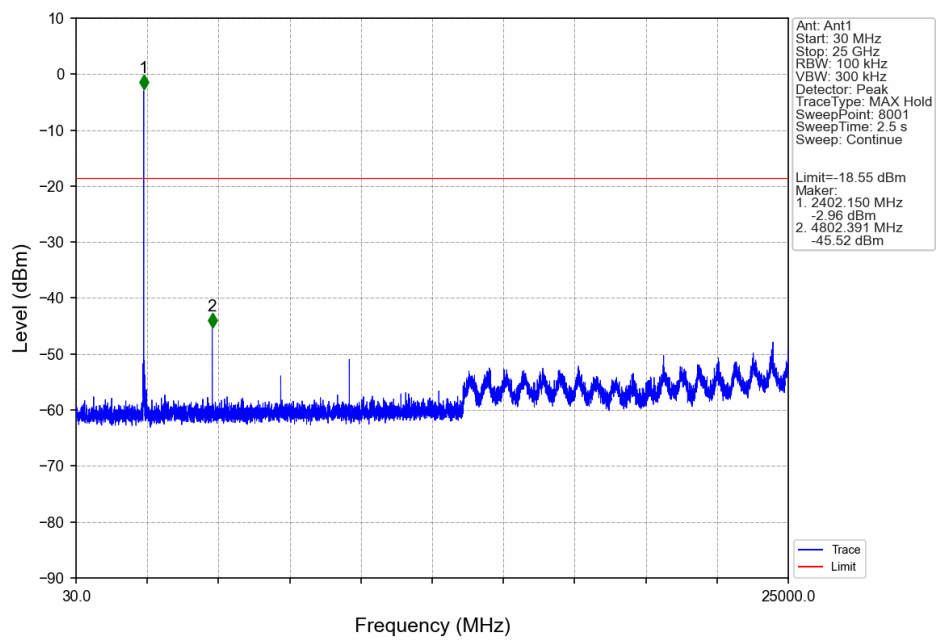
8DPSK_3DH5_LCH_2402MHz_Ant1_NTNV
