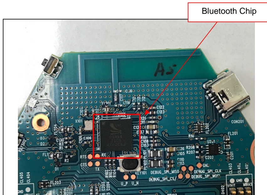
View of Bluetooth Chip
