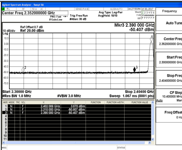
Channel 0 / 2402 MHz – Peak
