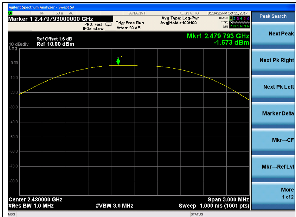
(Channel 39, 2480MHz, GFSK)
