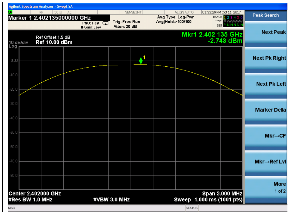
(Channel 0, 2402MHz, GFSK)
